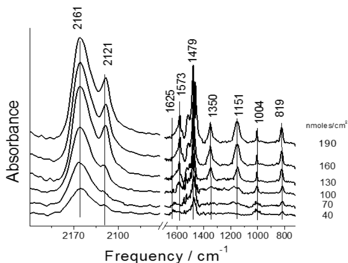
Figure 6.6: A series of ATR infrared spectra of BPDI adsorbed on a thin gold film using aliquots of 0.005 mM BPDI. The resulting BPDI doses, in \text{nmole/cm}^2 , are indicated adjacent to the corresponding spectrum.
