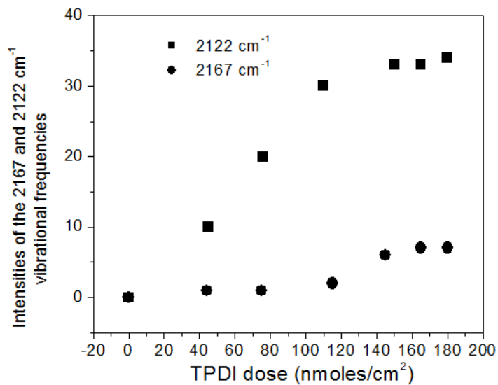
Figure 6.9: The variation in intensities of the 2167 and 2122 cm -1 vibrational frequencies as a function of TPDI dose (in nmoles/cm 2 ).
