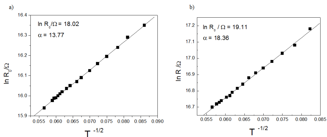
Figure 7.2: The linear \ln(R) versus T^{-1/2} dependence for two different samples is predicted by the model of Abeles and Sheng. R_o sheet resistance of the film prior to dosing, and scales with gold coverage. a) Gold nanoparticles with initial coverage of 15.00 nS linked with BPDT molecules and b) gold nanoparticles with initial coverage of 5.0 nS linked with TPDT
