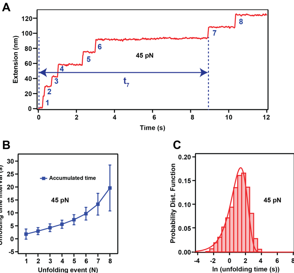
Figure 2.18. Graphs showing the accumulated time interval to measure the unfolding rate for protein L unfolding at 45 pN. (A) Representative trace of unfolding polyprotein L8 at a constant force 45 pN showing the accumulated time. (B) Graph showing the average accumulated time of polyprotein L8 as a function of unfolding events. Error bars represents the standard deviation of the average. (C) Histograms of the natural logarithm of the measured accumulated times of protein L at 45 pN. The continuous line represents the individual fit using a single exponential law.
