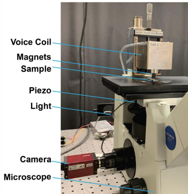
Figure 2.4. Image of the mechanically isolated magnetic tweezers setup and its components with supporting structures on the pneumatic table.
