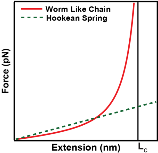
Figure 1.3. Worm-like chain model showing the nonlinear behavior of extension of an entropic polymer elasticity as a function of force. This model describes the protein becoming an unstructured polypeptide chain after crossing the barrier.
