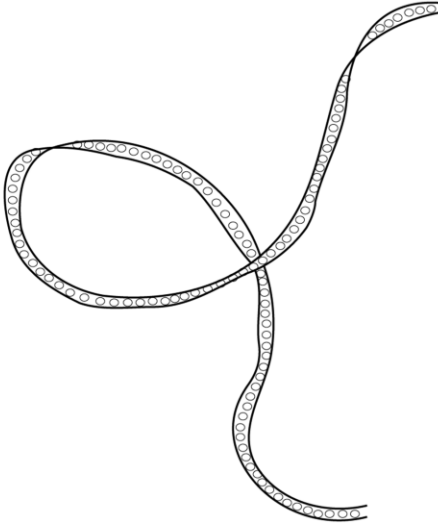
Figure 1.1. Schematic of a peptide bond, an unfolded peptide, and native folded structure of protein chain. (A) General structure of protein showing regular polypeptide backbone (\text{NH}-\text{CH}-\text{CO})_i with various side groups (\text{R}_1, \text{R}_2, \dots, \text{R}_i) , whose sequence in the chain is different for each protein (as established by Sanger in 1950s). NH groups of the backbone can form hydrogen bonds with CO groups of the other amino acid residues. (B) A polypeptide linear chain of amino acids forming the primary structure of protein as a polypeptide. (C) Schematic of a three-dimensional folded structure of B1 domain of protein L containing an \alpha -helix and three \beta -strands [PDB: 1HZ5].
