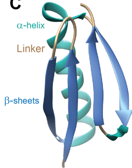
Figure 1.1. Schematic of a peptide bond, an unfolded peptide, and native folded structure of protein chain. (A) General structure of protein showing regular polypeptide backbone (\text{NH}-\text{CH}-\text{CO})_i with various side groups (\text{R}_1, \text{R}_2, \dots, \text{R}_i) , whose sequence in the chain is different for each protein (as established by Sanger in 1950s). NH groups of the backbone can form hydrogen bonds with CO groups of the other amino acid residues. (B) A polypeptide linear chain of amino acids forming the primary structure of protein as a polypeptide. (C) Schematic of a three-dimensional folded structure of B1 domain of protein L containing an \alpha -helix and three \beta -strands [PDB: 1HZ5].
