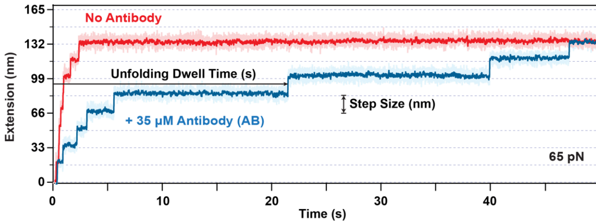
Figure 3.5. Unfolding protein L8 in the presence and absence of antibodies. Example of a trace of the same single molecule unfolding all its eight domains in the absence (red) and presence (blue) of antibodies ( 35 \mu\text{M} ) under a constant force ( 65 \text{ pN} ). Each step corresponds to the unfolding and extension of a protein L domain. The unfolding dwell-time and step size are defined as indicated by the arrows [Image source: (Dahal et al. 2020)].
