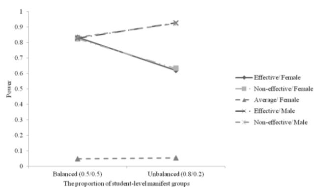
Figure 4.6 Power of Detecting Both-level DIF When Conducting Confirmatory Analyses: S_group
