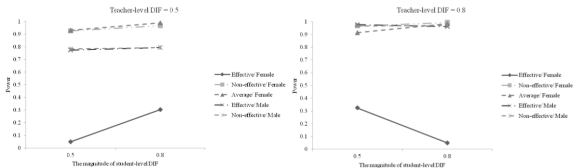
Figure 4.5 Power of Detecting Both-level DIF When Conducting Confirmatory Analyses: 3-way interaction
