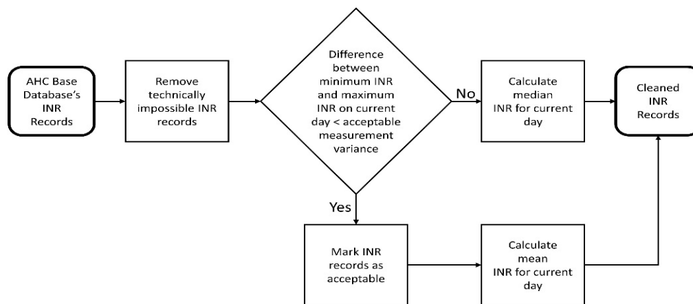
Figure 4.6. INR records cleaning algorithm.
