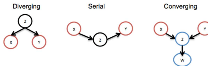
Figure 3.4. D-Separation.
