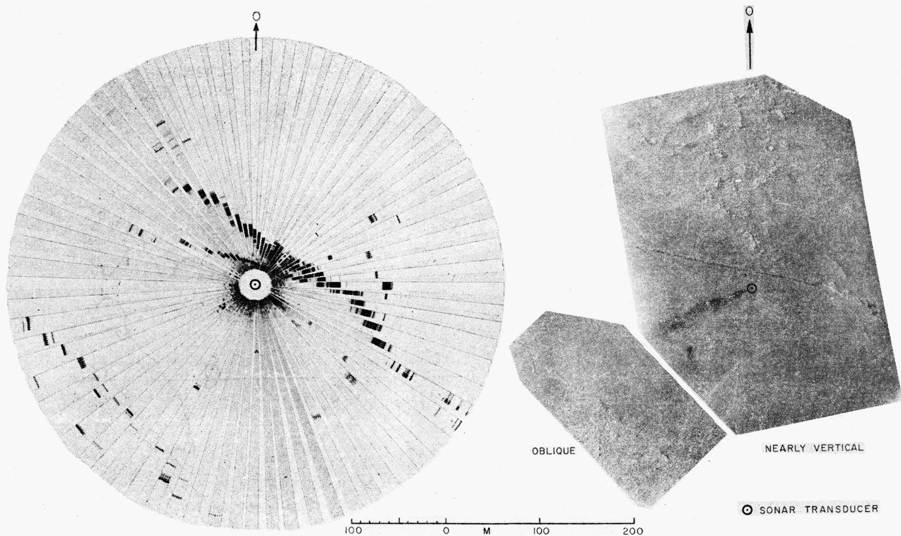
Figure 3. Comparison of Underice Sonar Map (left) and Aerial Photograph of the Sea Ice Surface (right). The data were taken at a site about 175 km north of Barrow, Alaska. The ice thickness at the sonar hole was 1.5 meters and the transducer was at 8.8 meters depth. The underice ridge at the top is generally deeper than the sonar transducer, and thus blocks sound from reaching most areas beyond it. Sonar maps taken at different transducer depths give additional information about the nature of the underice surface. The smoke grenades were used as reference points.
