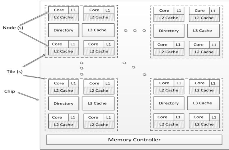
Figure 1. Target System Architecture
