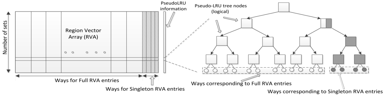
Figure 5. Asymmetric Region Vector Array Design. The ways holding small entries are shaded in dark gray.
