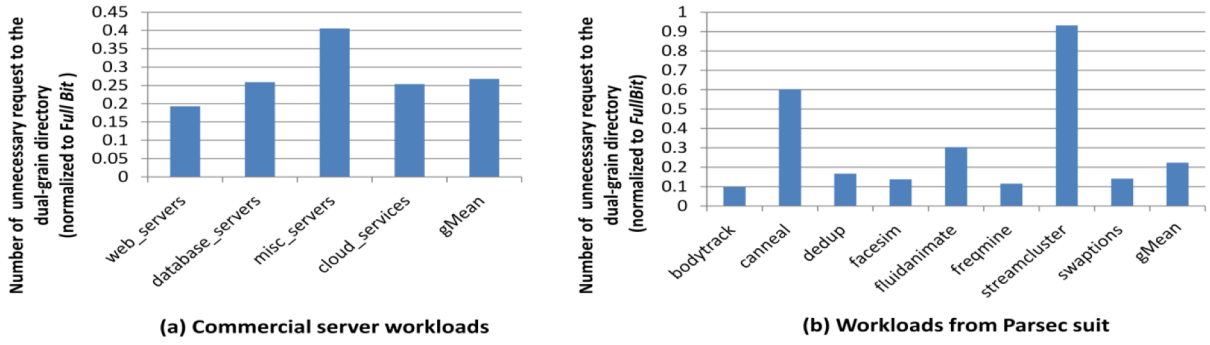
Figure 7. Normalized Number of "Unnecessary" Look-ups to the Coherence Directory.
