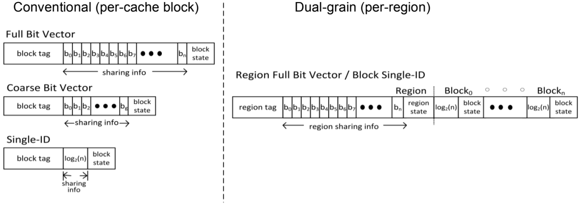
Figure 2. Directory Entry Comparison. The full bit vector tracks at node ( n ) granularity, while the coarse-grain bit vector tracks sharers at group ( g ) granularity.
