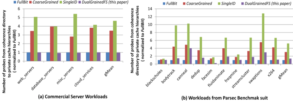
Figure 6. Comparison of Number of Coherence Probes Generated by Different Directory Schemes.
