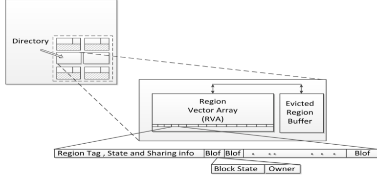
Figure 4. Basic Data Structures for Maintaining Region Grain Coherence.
