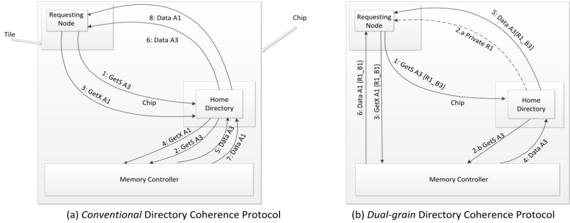
Figure 3. Region Privatization Example. Rx_y stands for blocks address that maps to region address "x" and the "y" block within region.
