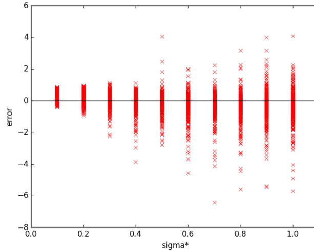
Figure 8: Range of hedged errors per \sigma_* for a Digital call option \sigma = 0.1 . The larger \sigma_* is, the more unpredictable are the errors.
