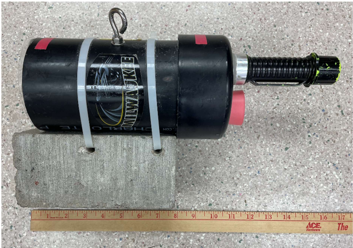
Figure 3: Diagram and photo of light trap designed for capture of Hemimysis based on input from Brown et al. 2017.
