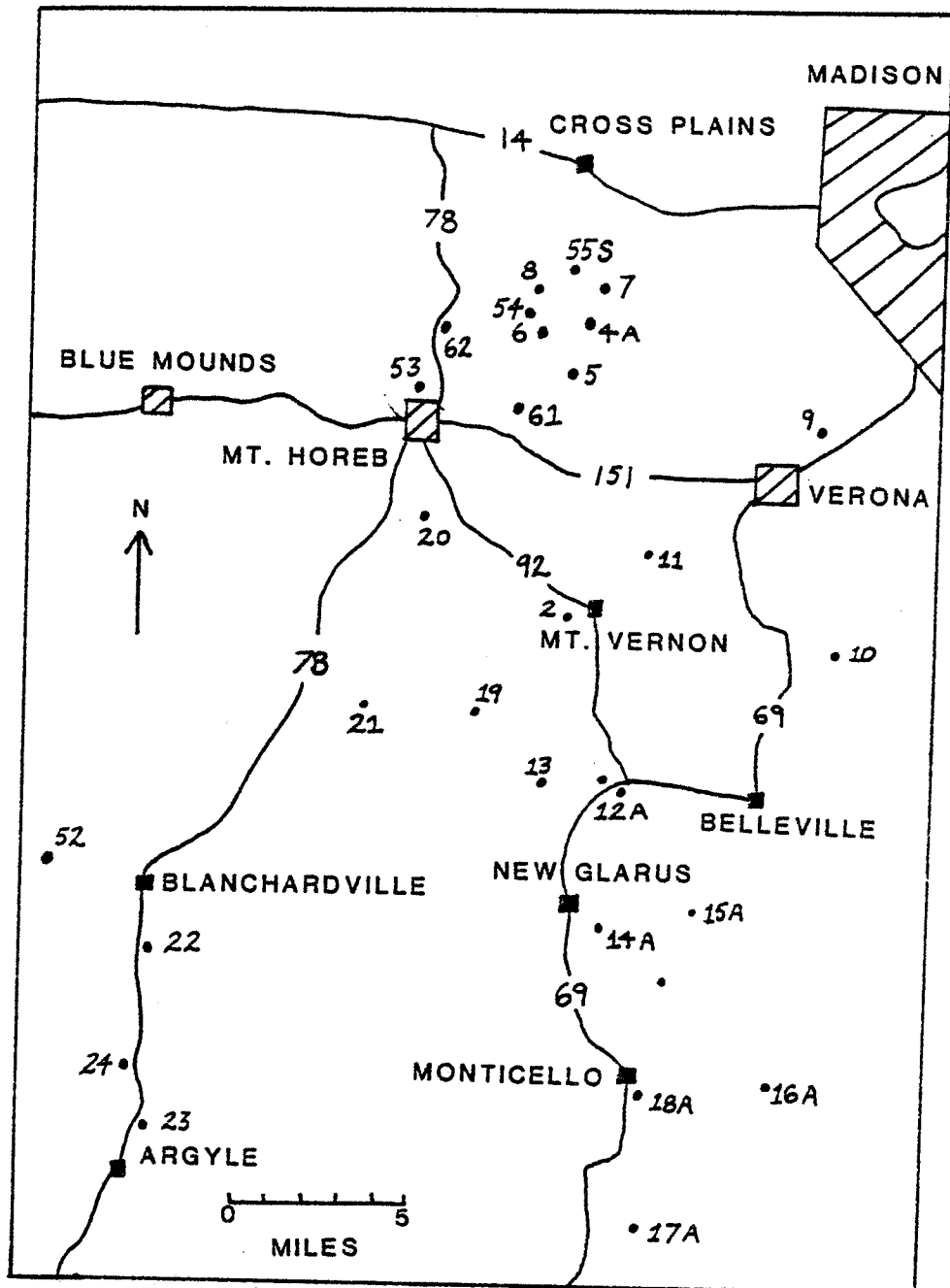
FIGURE 4: Outcrop index map for the Madison study area. See Figure 3 for legend. Outcrops #4-#24 have eolian facies. Outcrops #52-#55 are marine and #61 and #62 have both facies.
