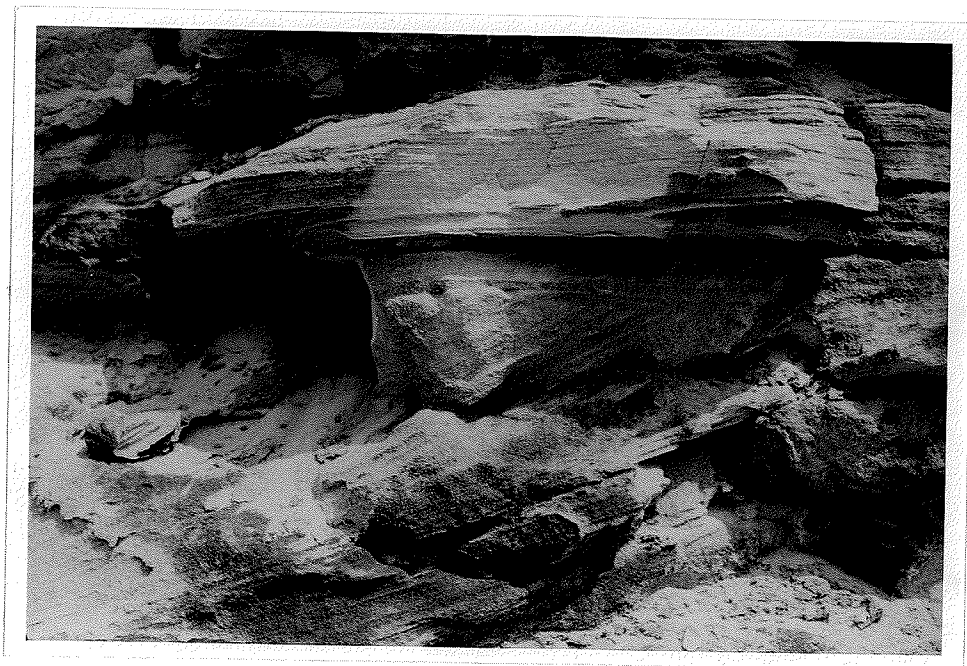
FIGURE 15: Bounding surface at New Glarus (outcrop #14, Appendix A). Note parallel laminae above and truncated laminae below the surface.
