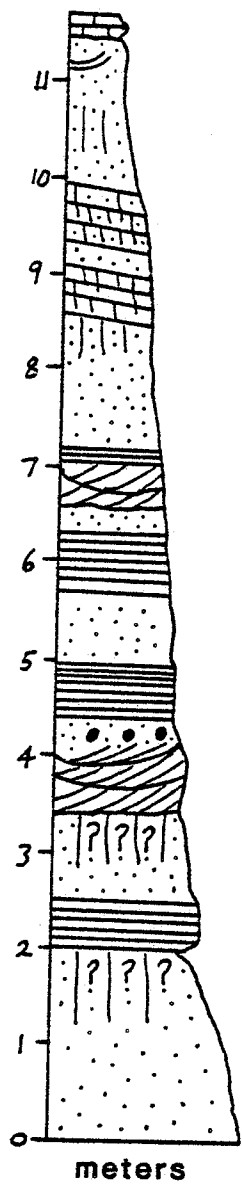
FIGURE 24: Measured section of Highway 178 roadcut near Starved Rock State Park, Illinois (outcrop #56, Appendix A).
