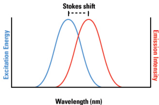
Figure 1-5: Stokes shift [58].
