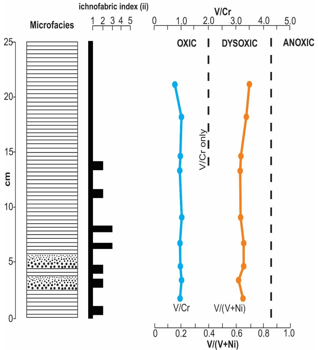
Figure 6 - Paleoredox indices (V/Cr and V/(V+Ni)), ichnofabric indices, and microstratigraphy (event beds vs. background sedimentation) of the 65 m horizon (ISP2) at Indian Springs. Event beds are dotted intervals (graded beds). Background sedimentation is shown as thin lines (laminations).
