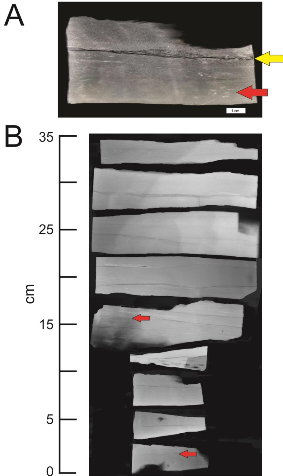
Figure 10 – X-radiographed slabs of rock samples from ISP1. A. Sample ISP1-6, yellow arrow indicating event bed, red arrow indicating bioturbation in the form of burrows. B. Red arrows indicating background laminations.
