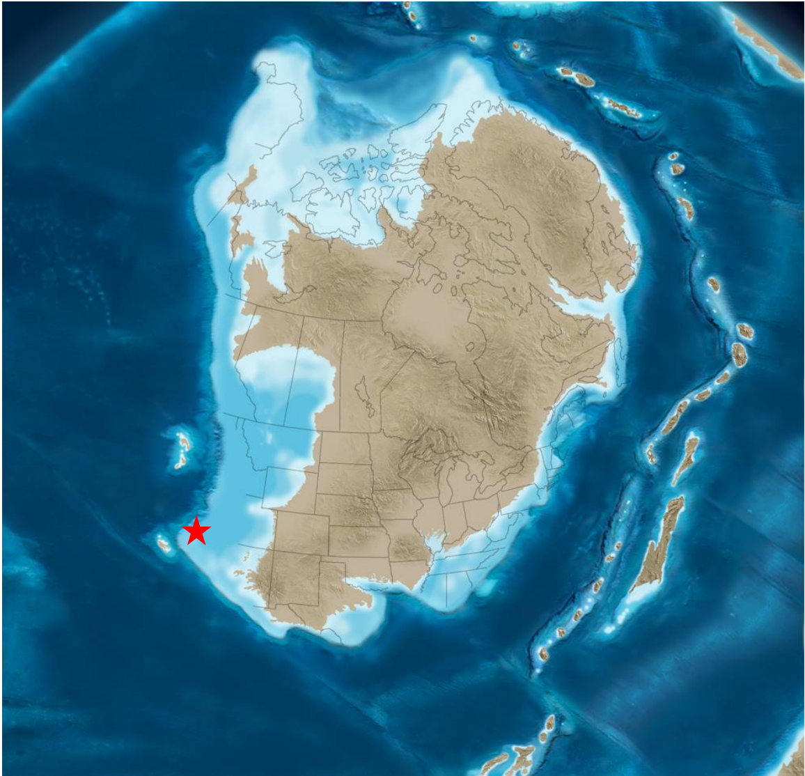
Figure 3 – Paleogeographic map of North America during the early Cambrian. Field site starred in red. From http://jan.ucc.nau.edu/~rcb7/namC510.jpg
