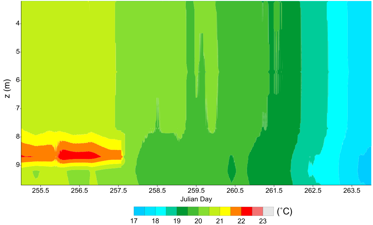
Figure 3.12f. Depth-time temperature plot for Station 8-13 from September 11-19, 2012.
