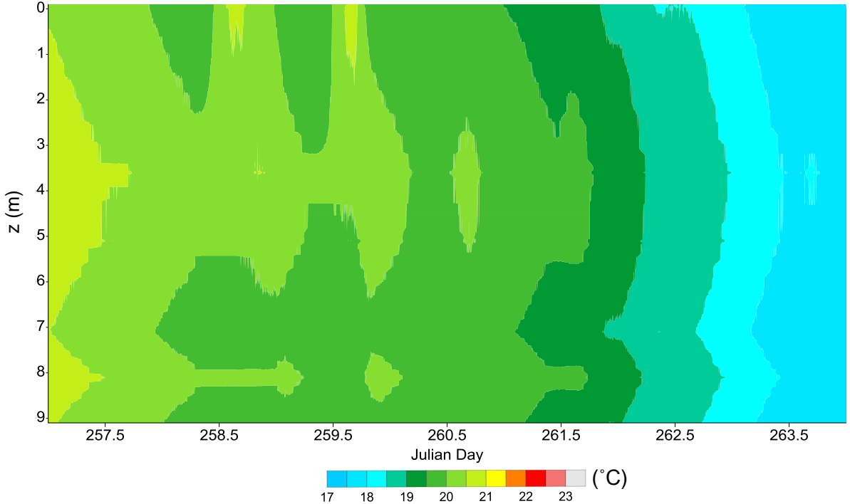
Figure 3.12g. Depth-time temperature plot for Station 9 from September 11-19, 2012.
