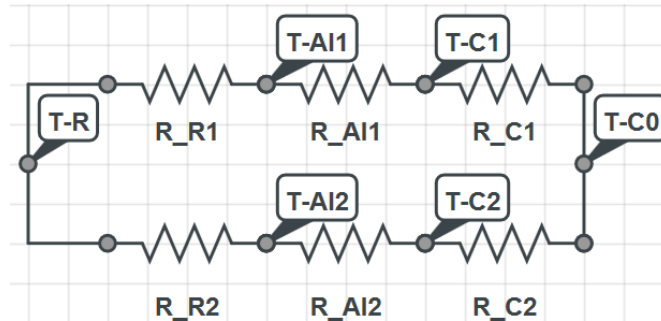
Figure 3.7: Radial Thermal Resistance Circuit of Frontal View of Coolant Chiller in Parallel
