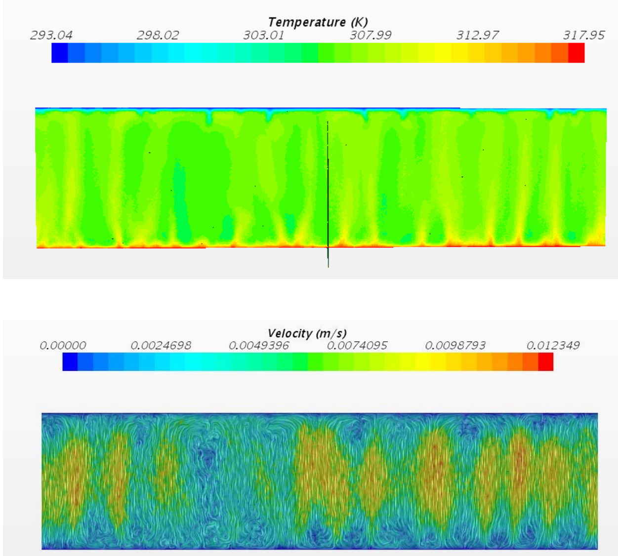
Figure B3: Side View of the Temperature and Velocity Profiles of the Bottom Coolant for 45°C
