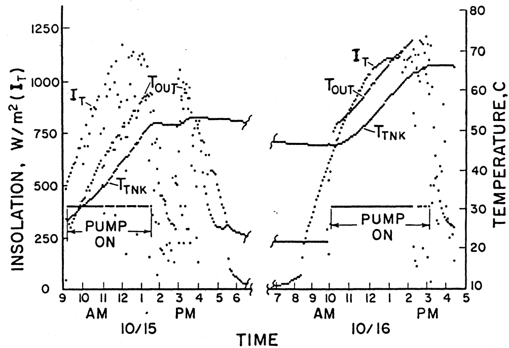
FIGURE 4.A.4. RAW DATA FROM MG&E SYSTEM TEST, OCTOBER 15 AND 16, 1982.
