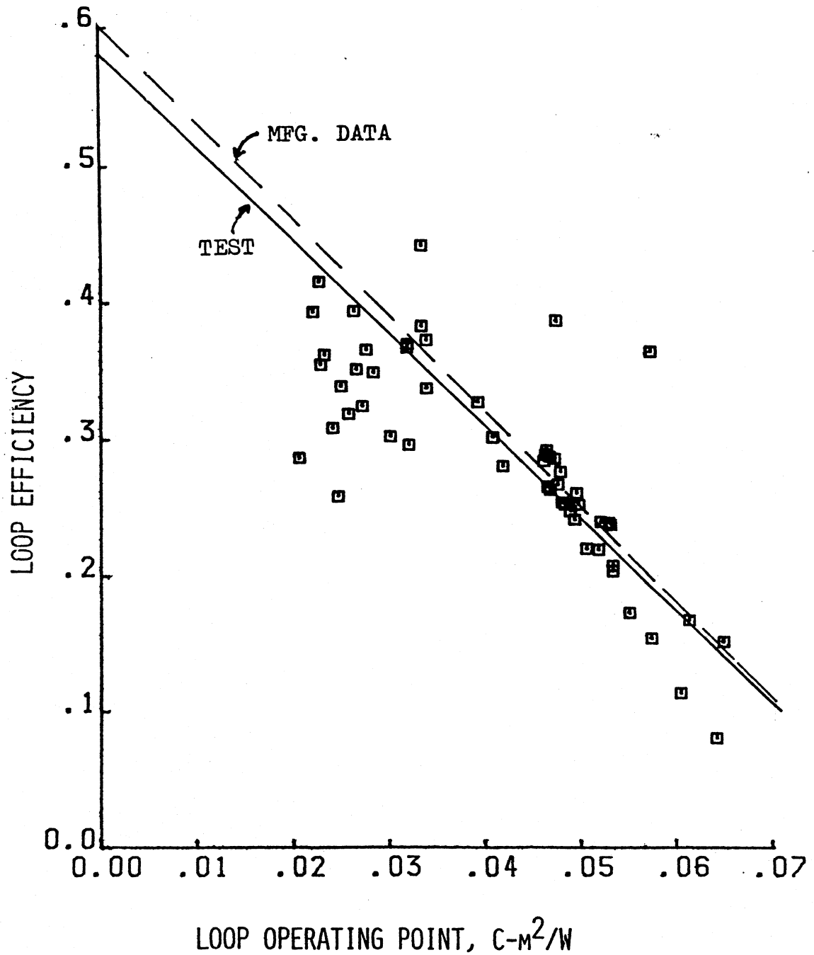
FIGURE 4.A.7. COLLECTOR LOOP EFFICIENCY VS. OPERATING POINT, MG&E SYSTEM, OCTOBER 15 AND 16, 1982.
