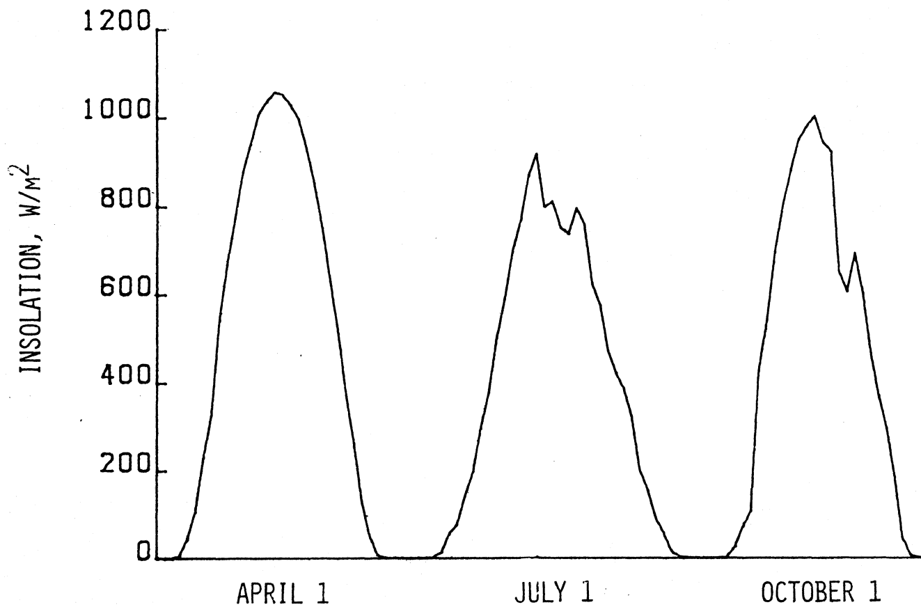
FIGURE 2.D.2. TILTED SURFACE INSOLATION PROFILES USED IN SIMULATIONS OF SDHW SYSTEM TESTS. MADISON, WISCONSIN, SLOPE = 45°
