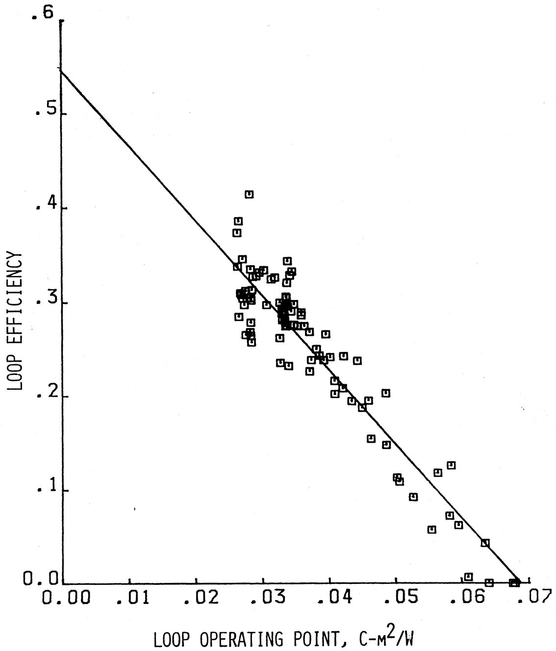
FIGURE 4.B.2. COLLECTOR LOOP EFFICIENCY VS. OPERATING POINT, BECKMAN SYSTEM, MAY 8 AND 9, 1983.
