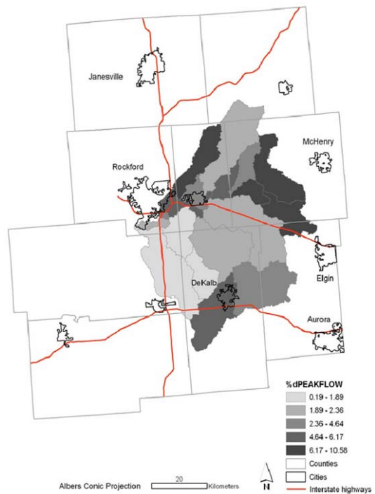
Figure 7. Same as Figure 4 but for annual peak flow
