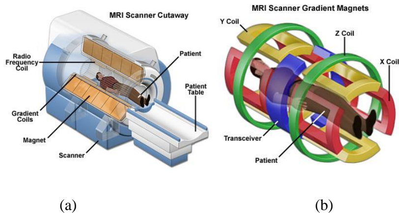
Fig 1.1: (a) MRI scanner system cutaway. (b) MRI scanner gradient magnets. (a) and (b) are from national high magnetic field laboratory. http://www.magnet.fsu.edu
