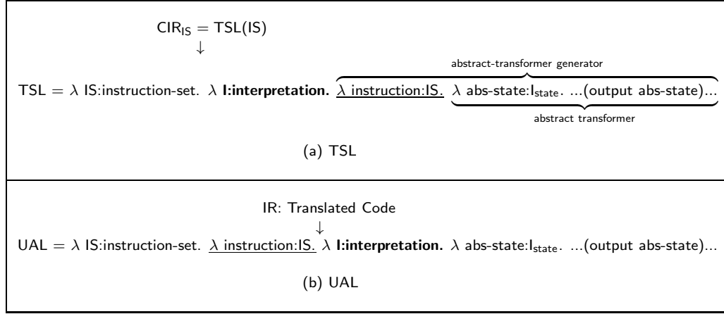
Fig. 20. A comparison of the UAL approach and TSL. (Note the use of dependent-type notation: “ instruction:IS ” means that instruction is an element of the language IS , and “ abs-state:I state ” means that abs-state is a state element in the space of values defined by interpretation I .)
