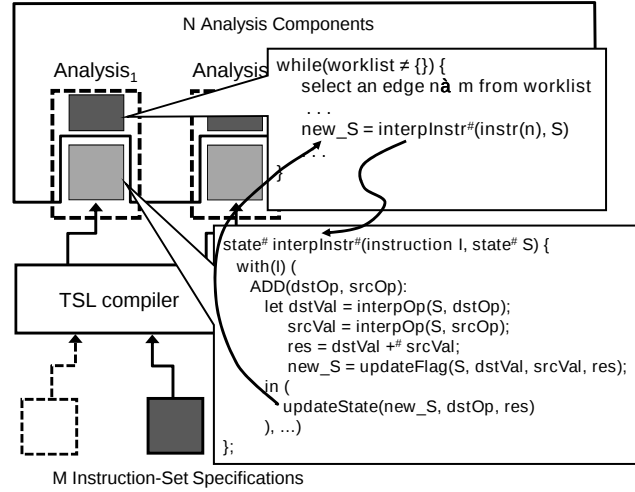
Fig. 9. How a TSL-generated abstract interpreter for instructions, \text{interplnstr}^\# , is invoked by an analysis engine that performs classical worklist-based propagation of abstract states.
