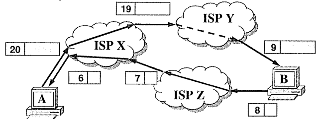
Figure 1: A uses Bill-Pay nanopayments to achieve priority service through congested ISP Y .
