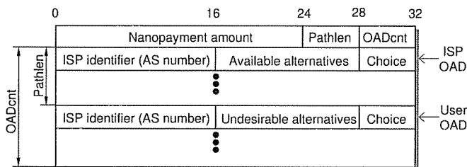
Figure 2: The Bill-Pay header structure
