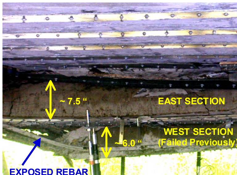
Figure 6.22. Concrete crushing along top of east section
