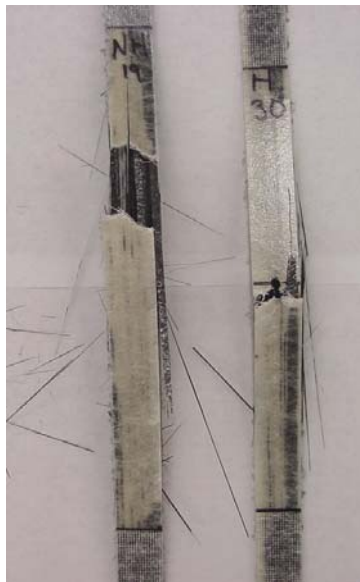
Figure 6.47. Failed coupons of virgin material (left – no hole; right – central hole)
