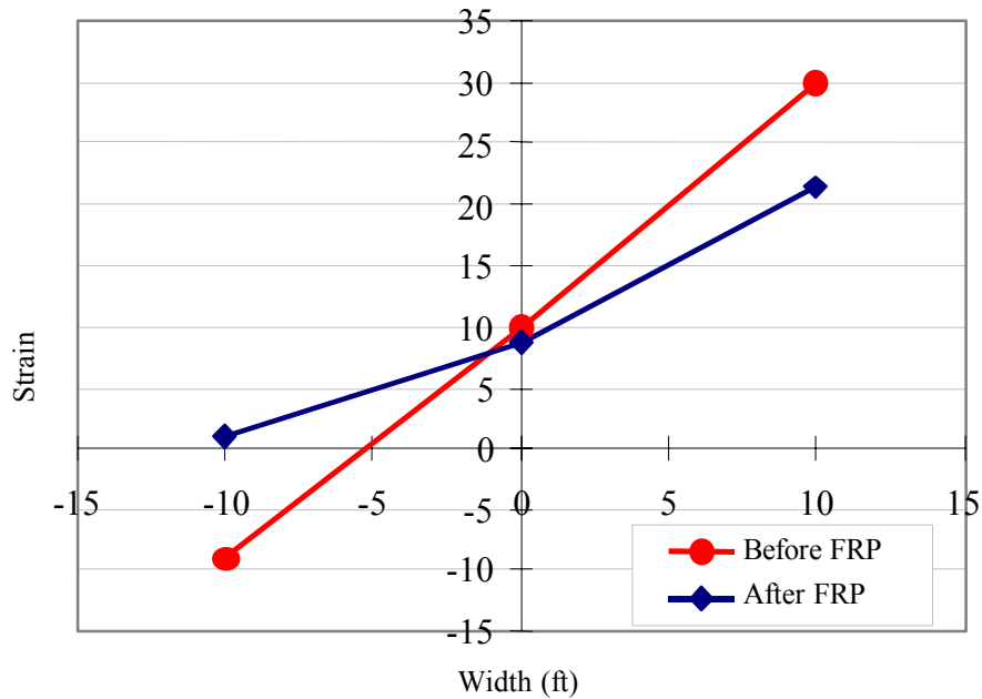
Figure 4.41. Strain distribution for Load Case IV
