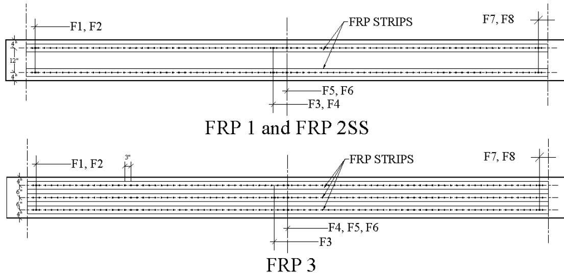
Figure 5.13. Location of FRP strain gages on laboratory beams
