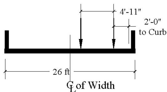
Figure 4.35. Load case for service load tests
