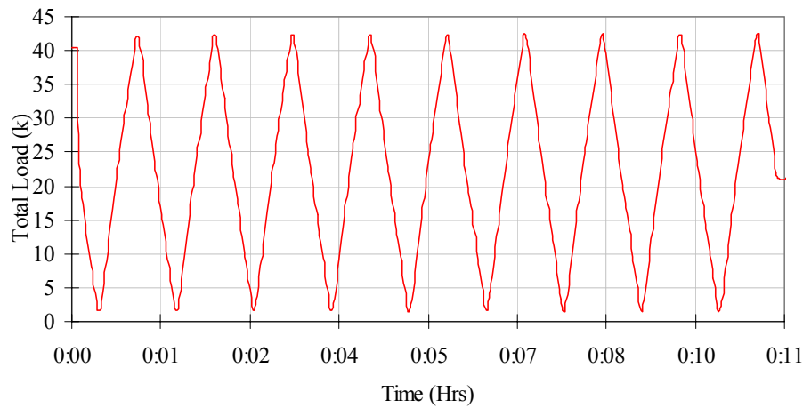
Figure 5.16. Loading cycles for beam FRP 3 in the inelastic range
