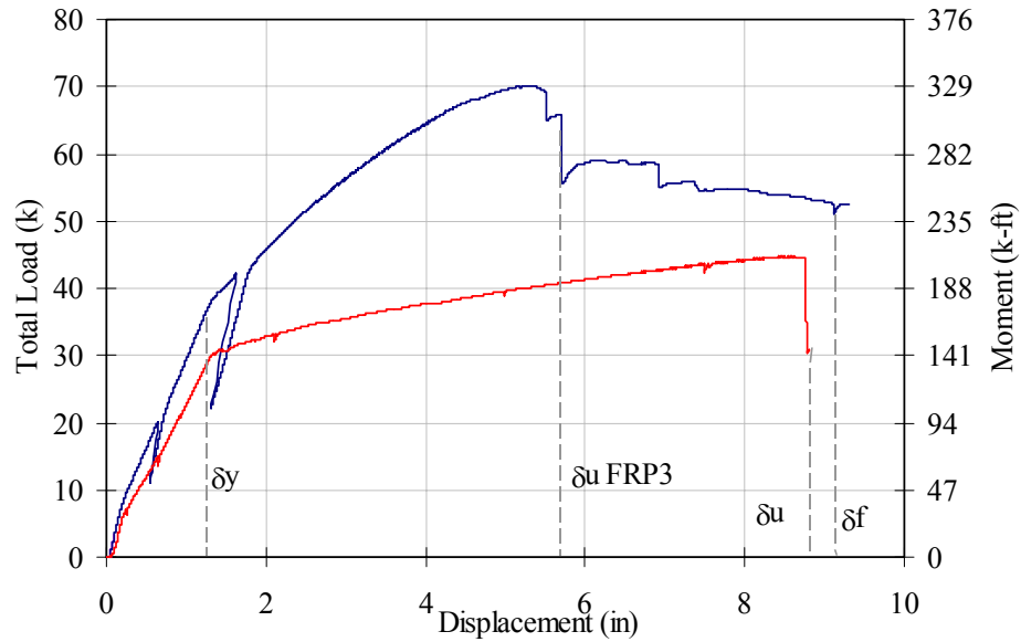
Figure 5.45. Comparison between beam FRP 3 and beam C-1
