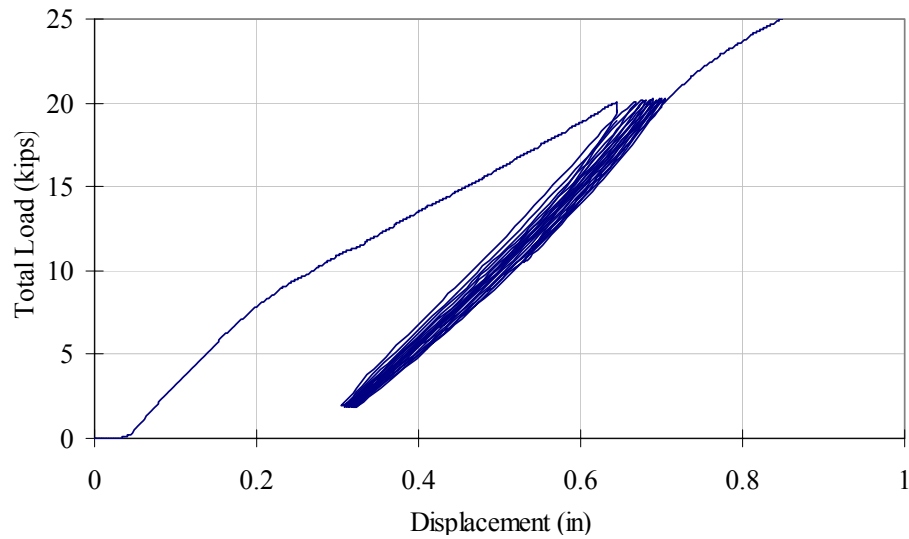
Figure 5.42. Load vs. Displacement plot for elastic cyclic loading on FRP 3
