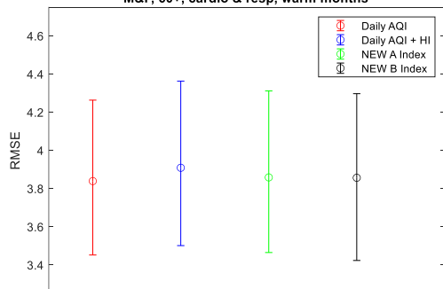
RMSE values of regression models in predicting mortality (lag 2) with 95% confidence intervals M&F, 60+, cardio & resp, warm months
