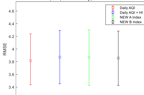
RMSE values of regression models in predicting mortality (lag 1) with 95% confidence intervals M&F, 60+, cardio & resp, warm months
