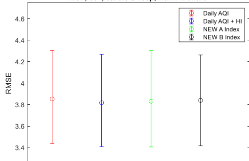
RMSE values of regression models in predicting mortality (lag 0) with 95% confidence intervals M&F, 60+, cardio & resp, warm months
