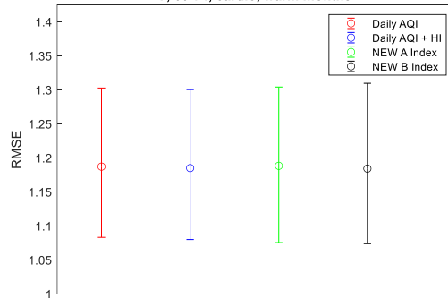
RMSE values of regression models in predicting mortality (lag 1) with 95% confidence intervals F, 60-74, cardio, warm months
