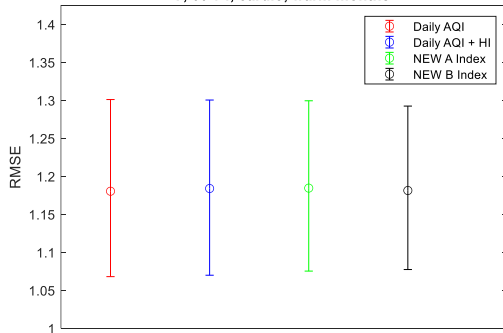
RMSE values of regression models in predicting mortality (lag 0) with 95% confidence intervals F, 60-74, cardio, warm months
