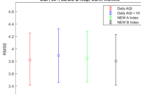
RMSE values of regression models in predicting mortality (lag 3) with 95% confidence intervals M&F, 60+, cardio & resp, warm months
