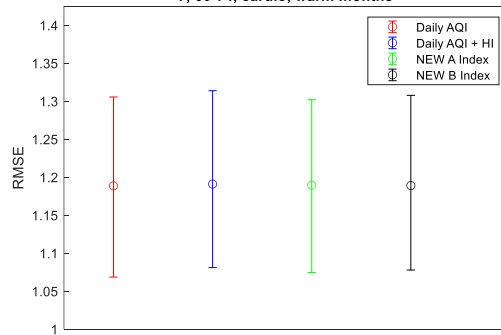
RMSE values of regression models in predicting mortality (lag 3) with 95% confidence intervals F, 60-74, cardio, warm months
