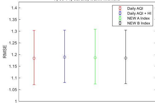
RMSE values of regression models in predicting mortality (lag 2) with 95% confidence intervals F, 60-74, cardio, warm months
