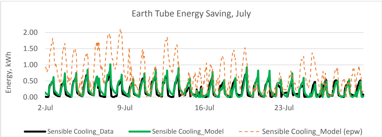
Figure 137. Model Validation, Earth Tube Sensible Cooling Energy Saving, July
