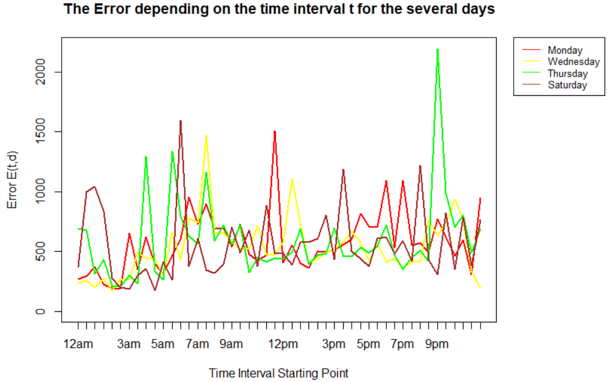
Figure 3: The error E(t, d) over time t for Monday, Wednesday, Thursday and Saturday.
