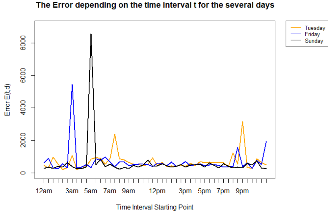
Figure 4: Error E(t, d) over time t for Tuesday, Friday and Sunday
