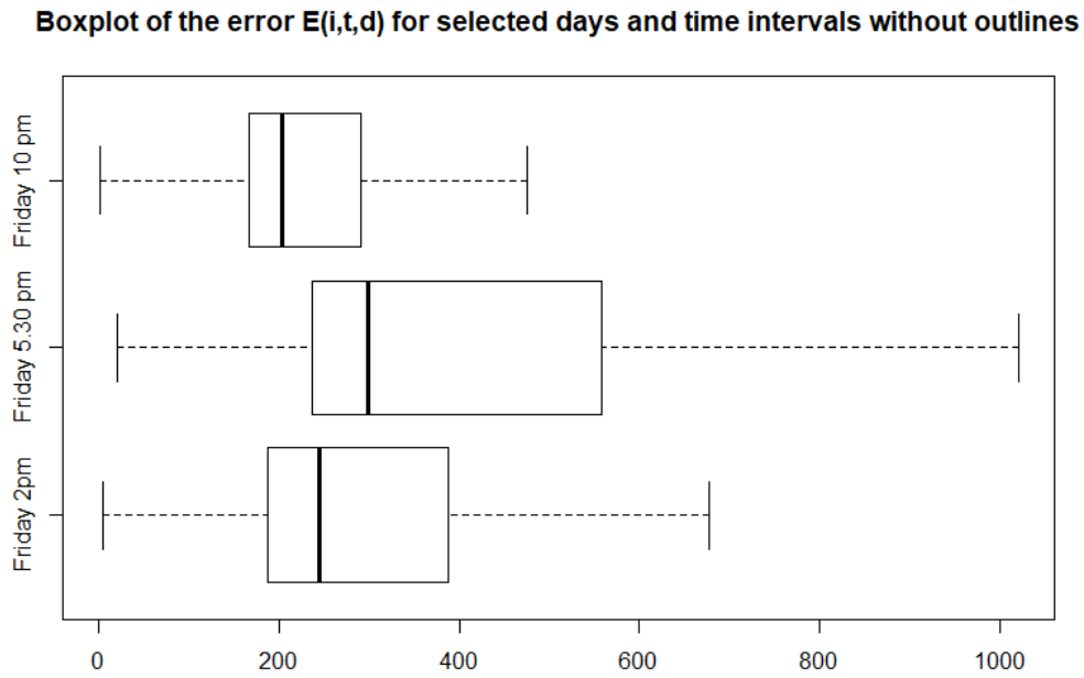
Figure 11: Boxplots of E(i,t,d) s for Friday at time intervals [2 pm, 2.30 pm), [5.30 pm, 6 pm) and [10 pm, 10.30 pm), without outliers.
