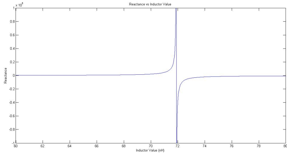
Figure 23: Reactance versus inductor value for a parallel LC tank with C=21.6 pF.
