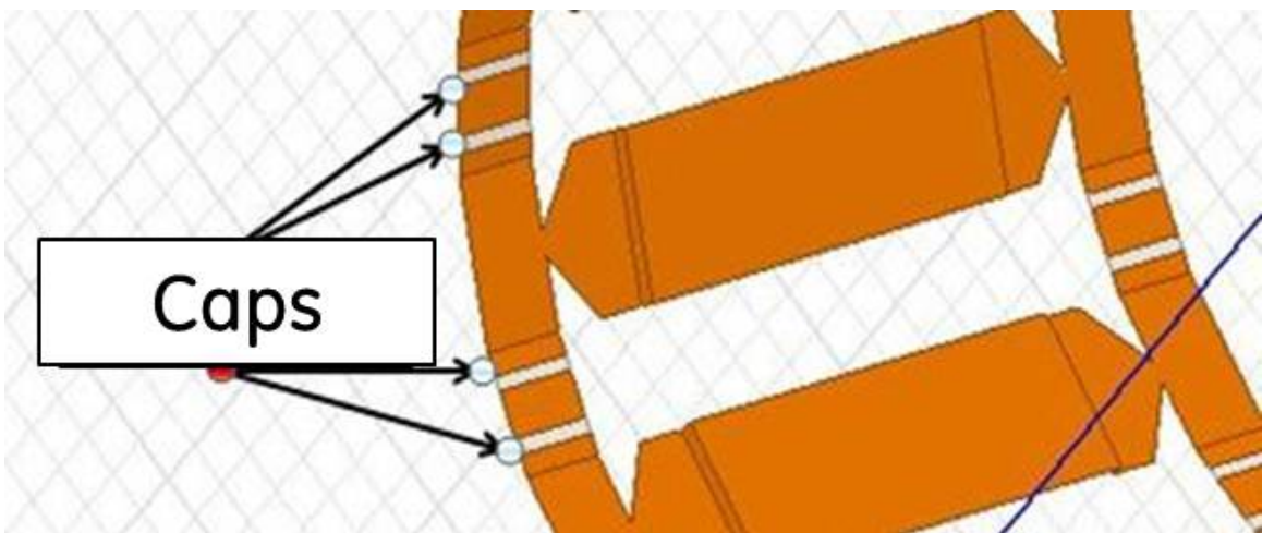
Figure 6: High pass birdcage capacitor locations.
