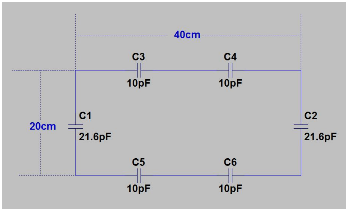
Figure 20: Tuning loop design details.
