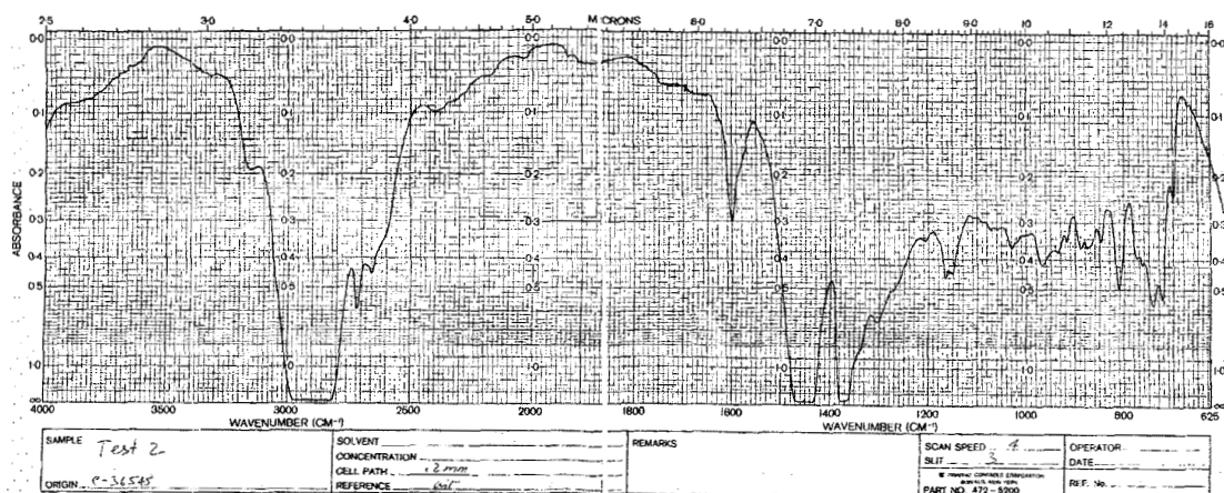
Figure 6. IR scan for the tested Ramapo oil with 0.2 mm cell path and air as reference beam. The absorbance difference in signature band \sim 700 to 1200\text{ cm}^{-1} shows that the Ramapo and TU oils are different products.
