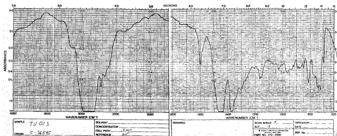
Figure 7. IR scan for the tested TU oil with 0.2 mm cell path and air as reference beam. The absorbance difference in signature band around 700 to 1200\text{ cm}^{-1} shows that the Ramapo and TU oils are different products.
