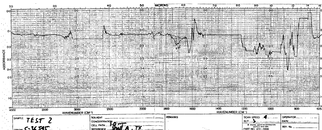
Figure 4. IR scan for the tested Ramapo oil with 1 mm cell path and new oil as reference beam. Little to none of oxidation inhibitor was detected at 3660 cm -1 . Carbonyl compounds detection region at 1700 to 1730 cm -1 shows more absorbance than that of TU oil in Figure 5.
