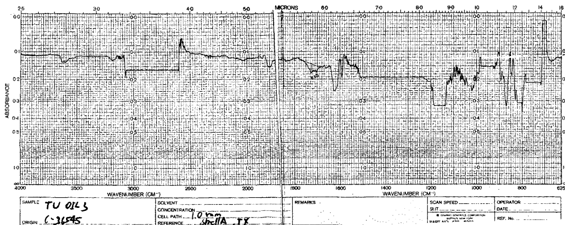
Figure 5. IR scan for the tested TU oil with 1 mm cell path and new oil as reference beam. Little to none oxidation inhibitor was detected at 3660 cm -1 . Carbonyl compounds detection region at 1700 to 1730 cm -1 shows less absorbance than that of Ramapo oil in Figure 4.
