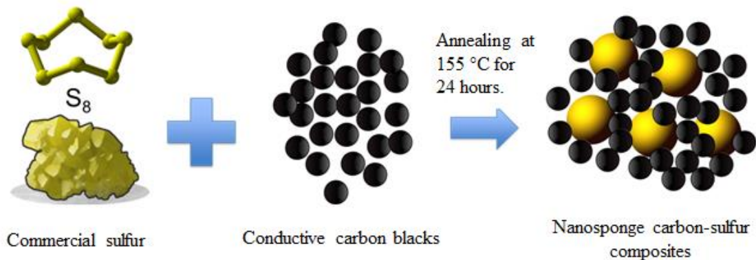
Figure 3.11 Synthesis of nanosponge sulfur carbon composites.
