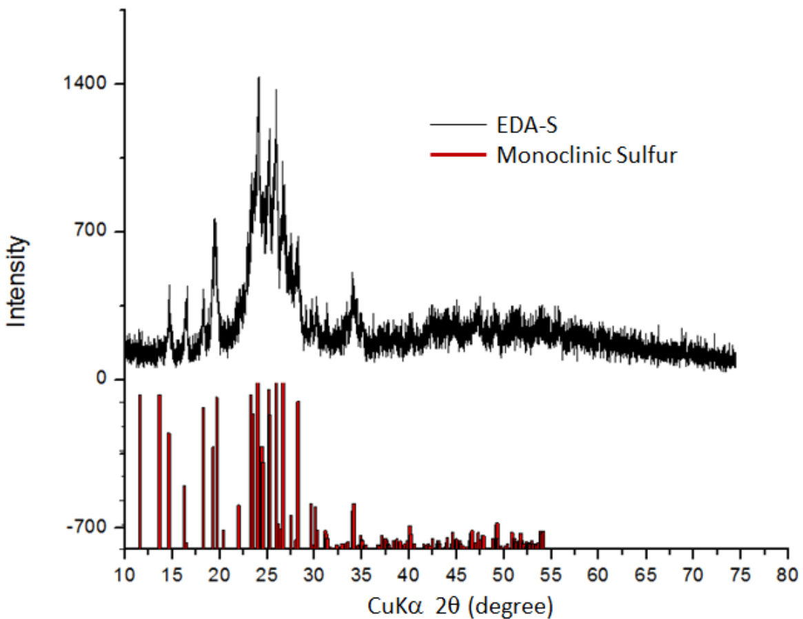
Figure 3.12 XRD pattern of nanosponge sulfur carbon composites.
