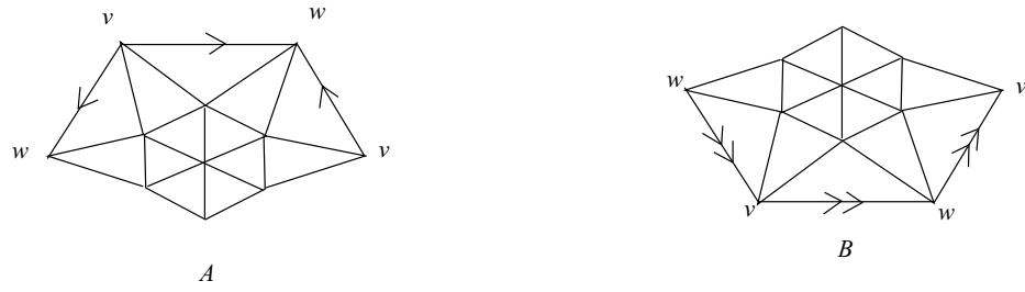
Figure 3.9: J “splits” into Collapsibles
