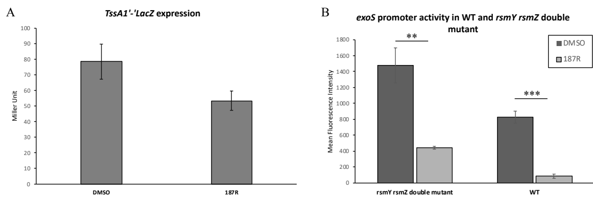
Figure 2.7 Effect of 187R on rsmY/Z/A regulatory pathway. (A) expression of tssA1' - lacZ translational fusion reporter with 187R and DMSO respectively. (B) exoS promoter activity in in the rsmYZ double mutant with the present of 187R and DMSO respectively. Statistical significance was determined using an two-tailed student's t-test (**, P < 0.01 ; ***, P < 0.001 ).
