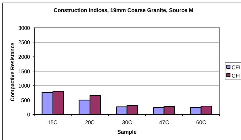
Figure 4.10. Construction Indices for 19mm Coarse Granite
