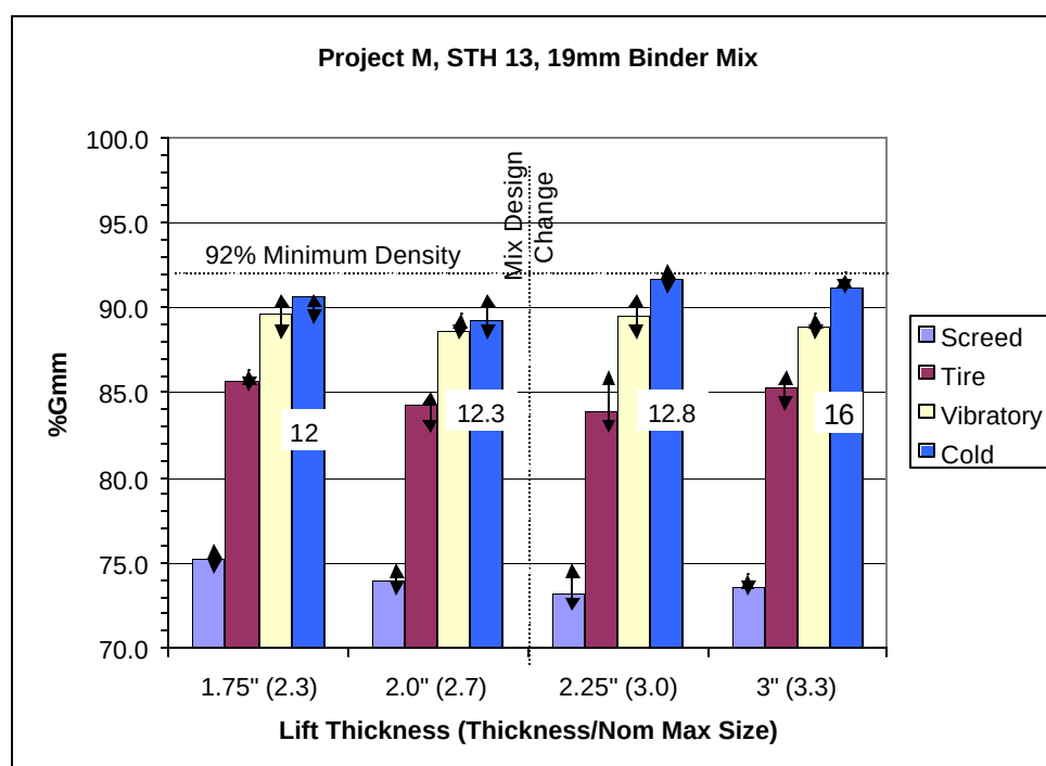
Figure 5.3. Project M, 19mm Binder Density Results
