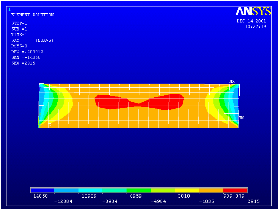
Figure 5.9. ANSYS Analysis of 1500 gram Sample
