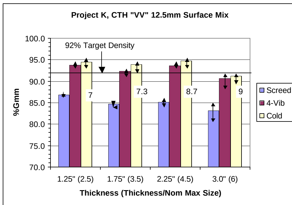
Figure 5.2. Project K, 12.5mm Surface Density Results
