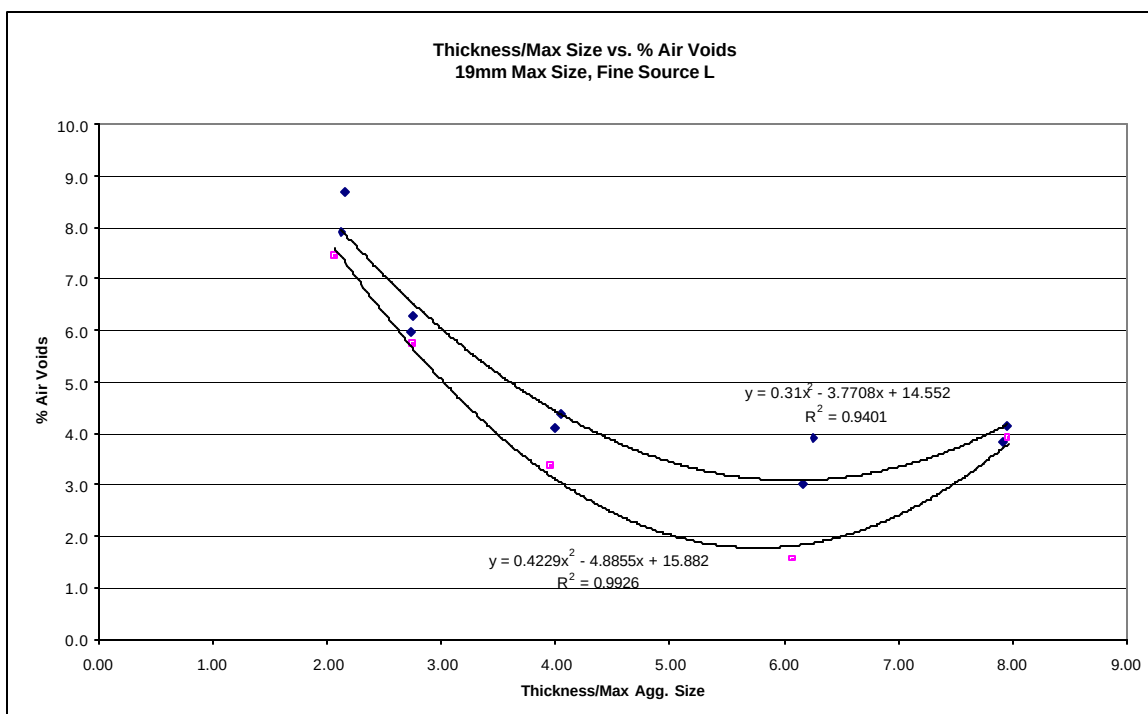
19mm Fine Limestone, Source L Air Void Plot
