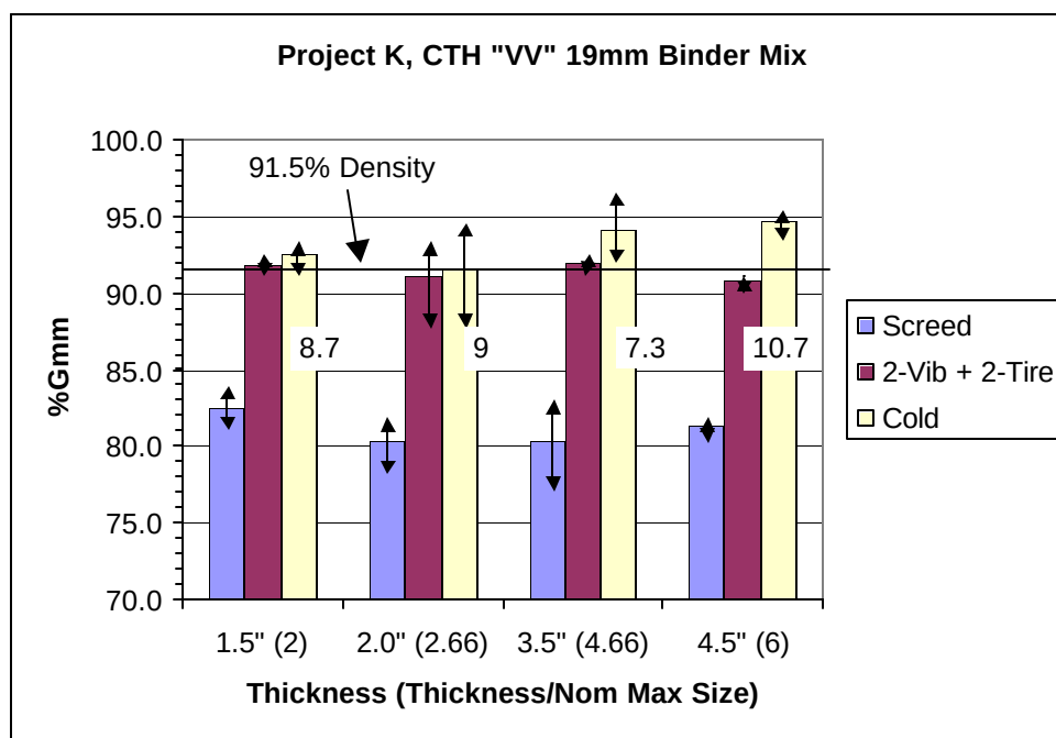
Figure 5.1. Project K, 19mm Binder Density Results
