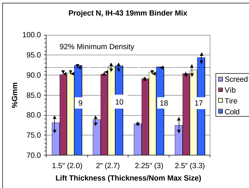
Figure 5.5. Project N, 19mm Binder Density Results
