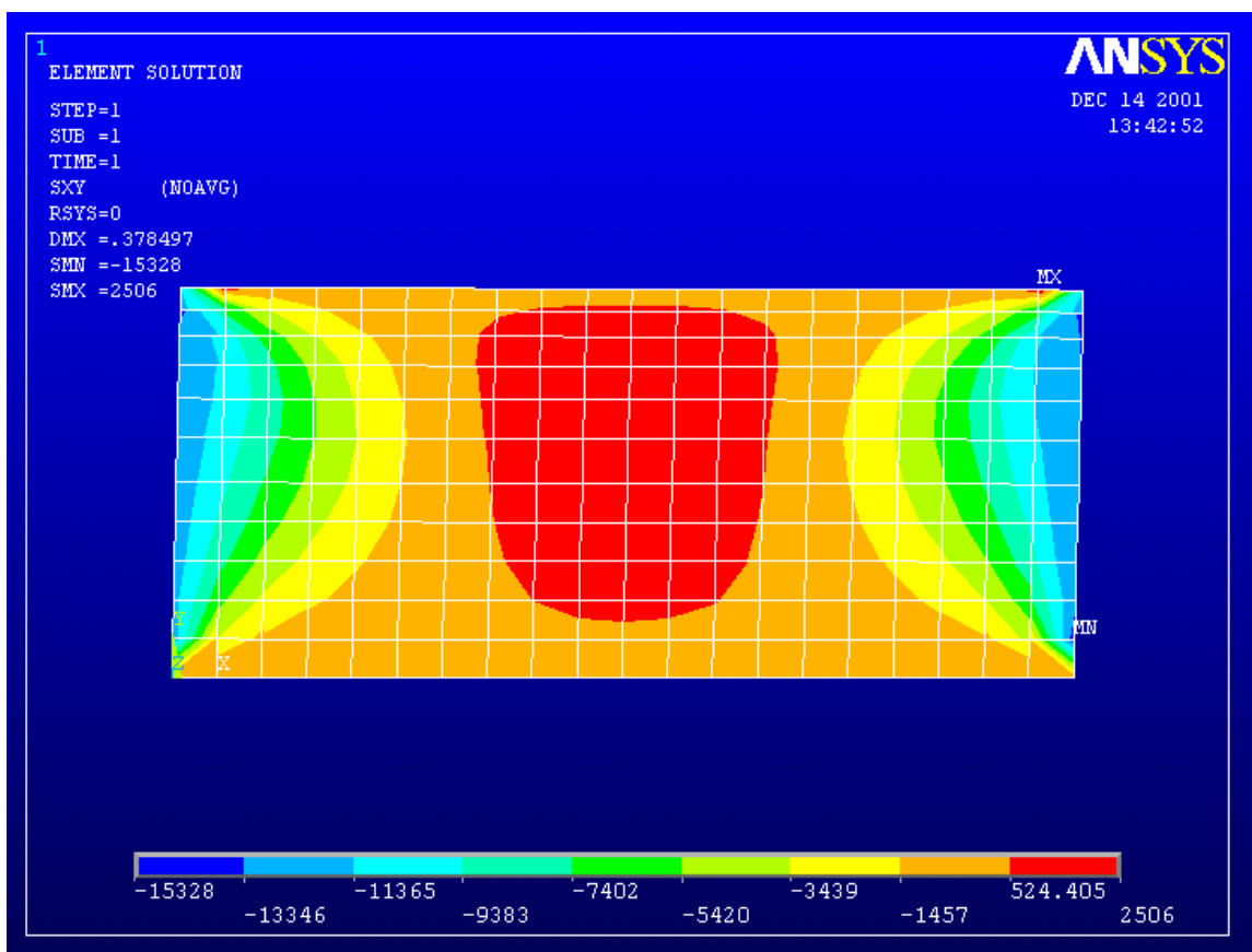
Figure 5.10. ANSYS Analysis of 3000 gram sample
