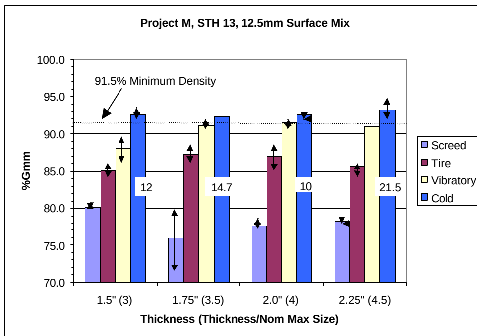
Figure 5.4. Project M, 12.5mm Surface Density Results
