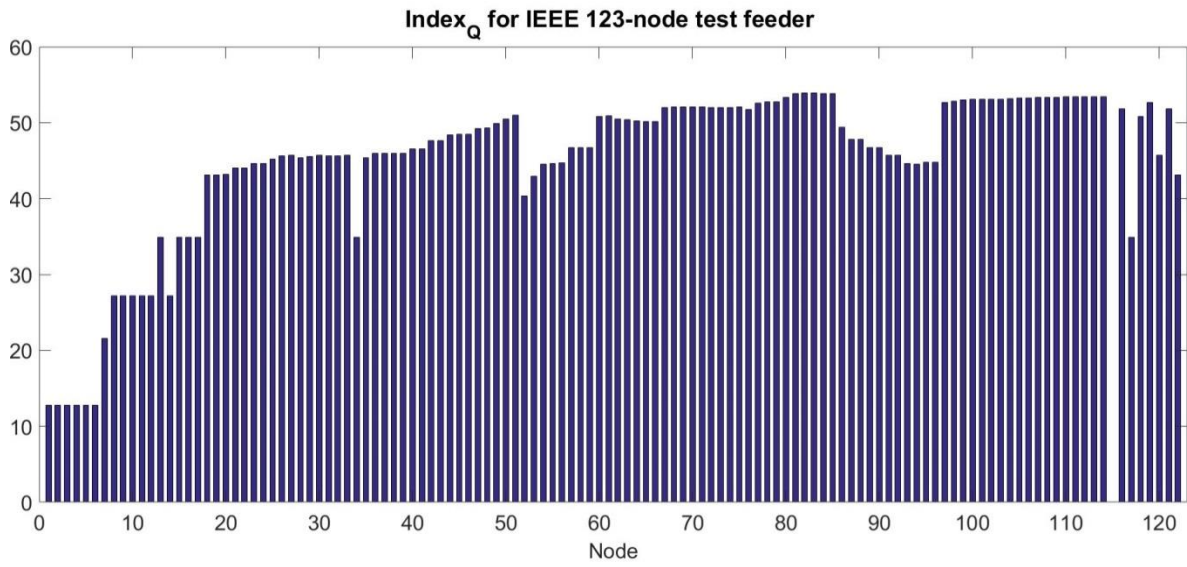
Figure 5. 8 Index Q of IEEE 123-node test feeder
