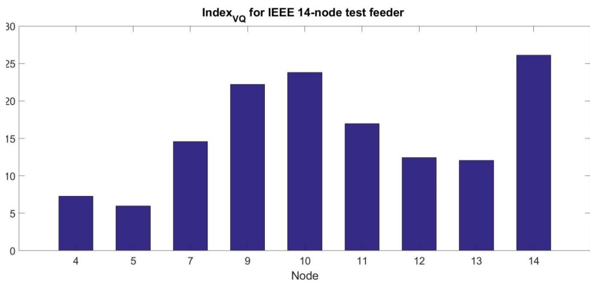
Figure 3.6 Index VQ of 14-node system
