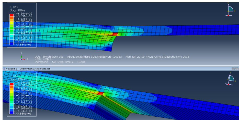
Figure 5.6: Shear stress distribution for paste adhesive
