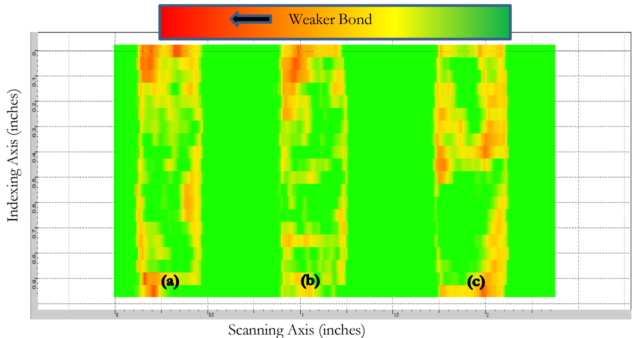
Figure 4.5: UT of Paste SLJ, (a) Control, (b) Mold Release, (c) Grease
