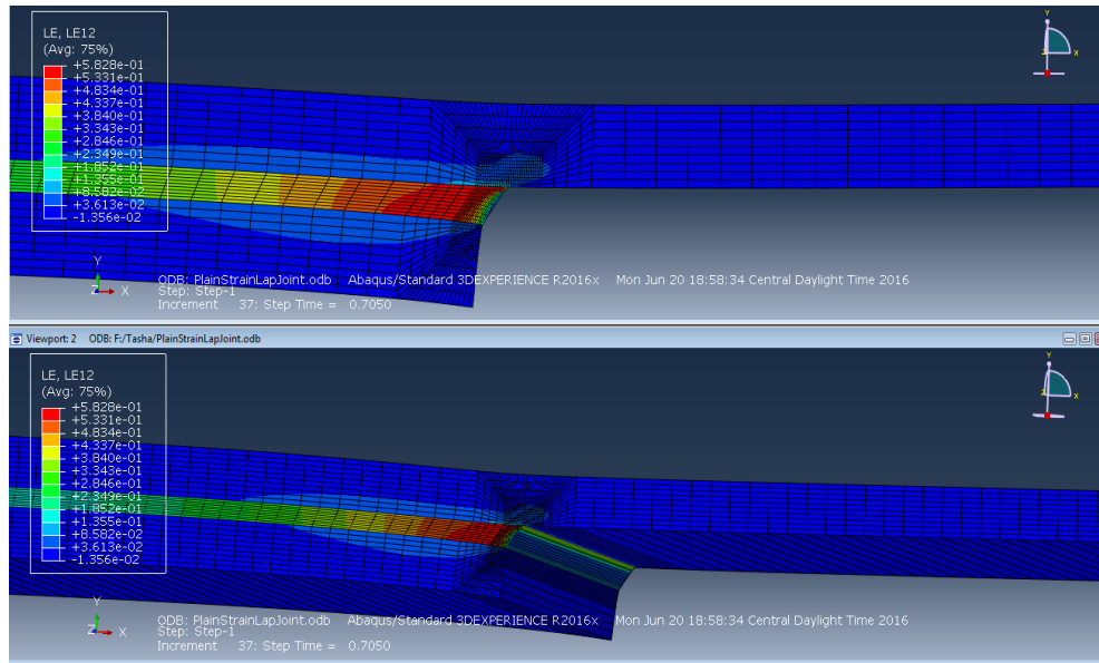
Figure 5.12: Shear strain distribution along bond line for 10-element mesh film adhesive
