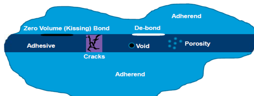
Figure 1.1: Defects that can occur in composite materials [1]
