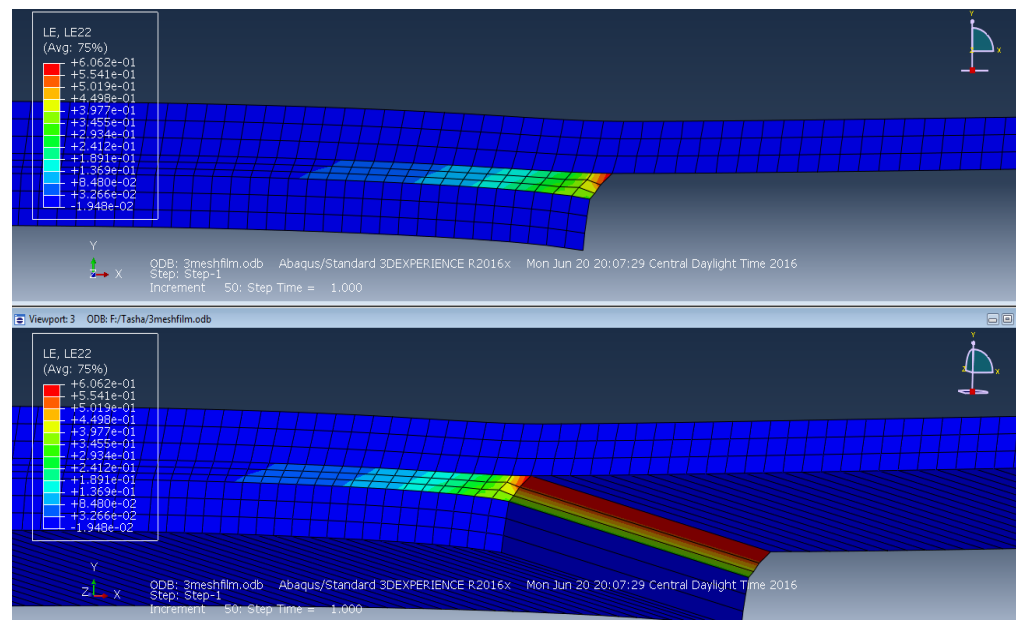
Figure 5.5: Peel strain distribution for film adhesive
