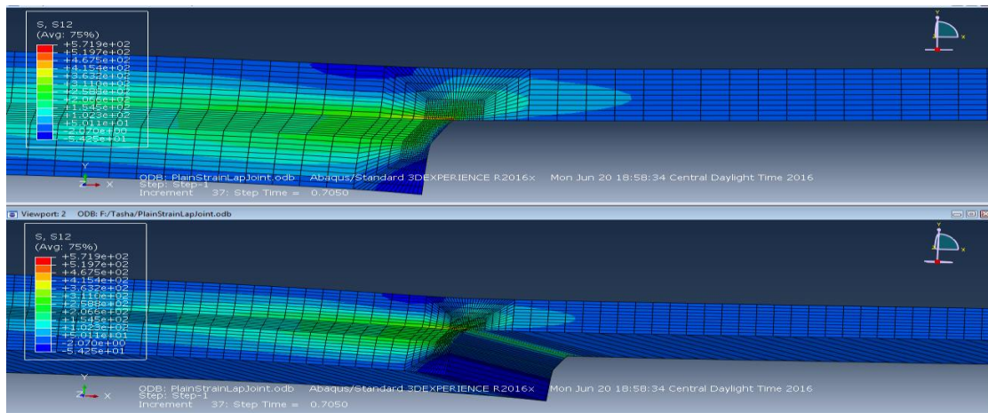
Figure 5.10: Shear Stress distribution along bond line for 10-element mesh film adhesive
