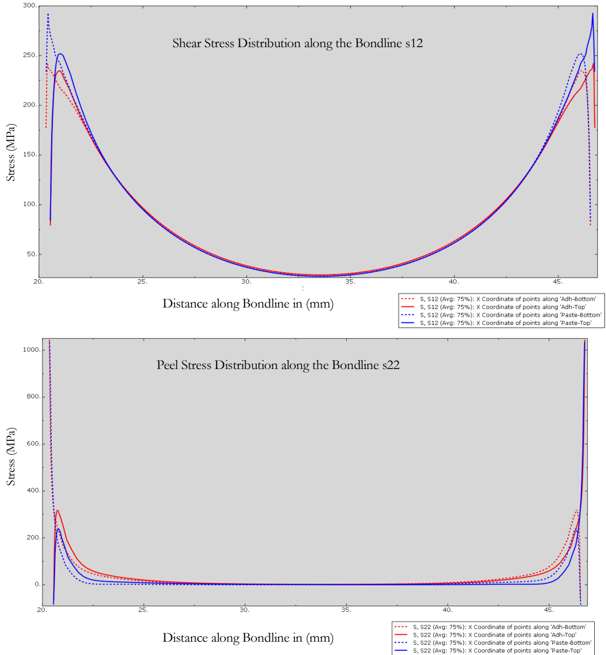
Figure 5.19: Peel and shear stress distributions for different adhesives
