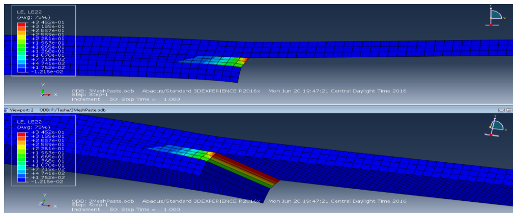
Figure 5.9: Peel Strain distribution for paste adhesive
