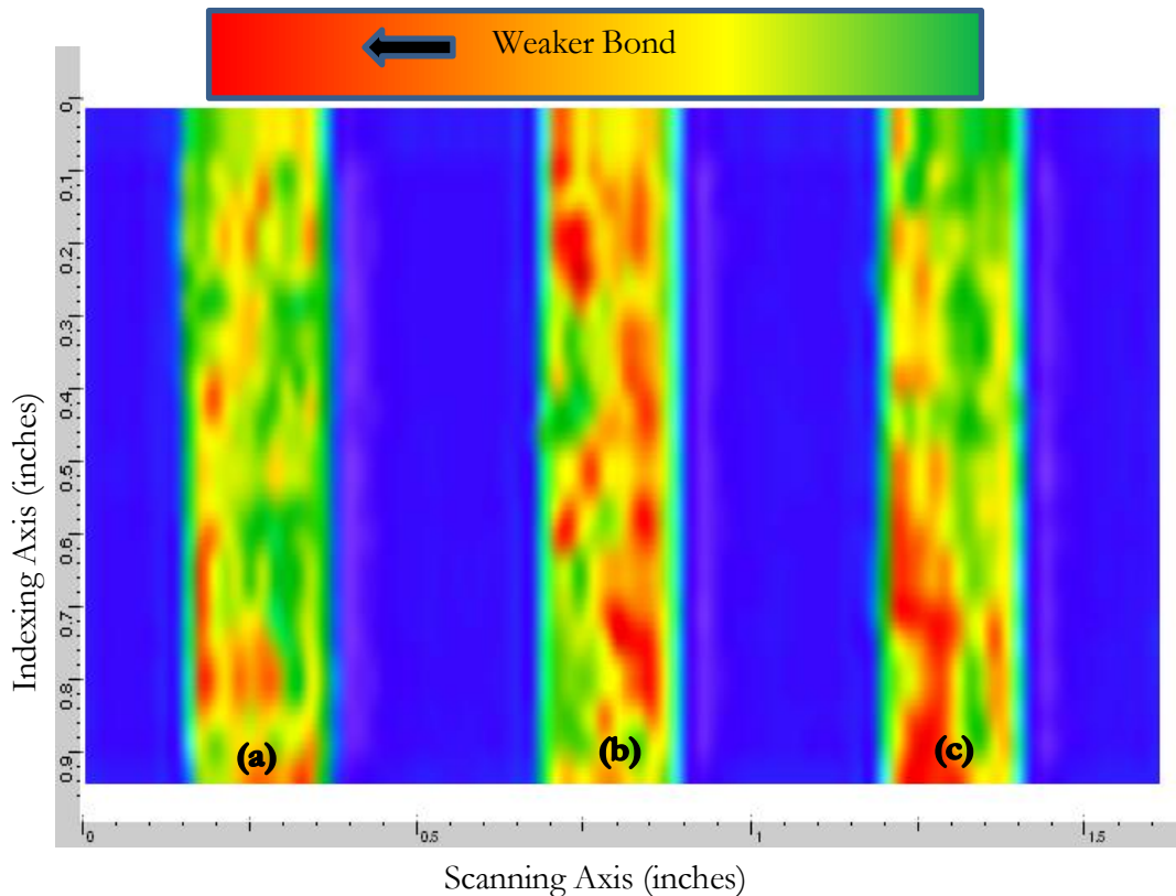
Figure 4.4: UT of Film adhesive SLJ, (a) Control, (b) Mold Release, (c) Grease
