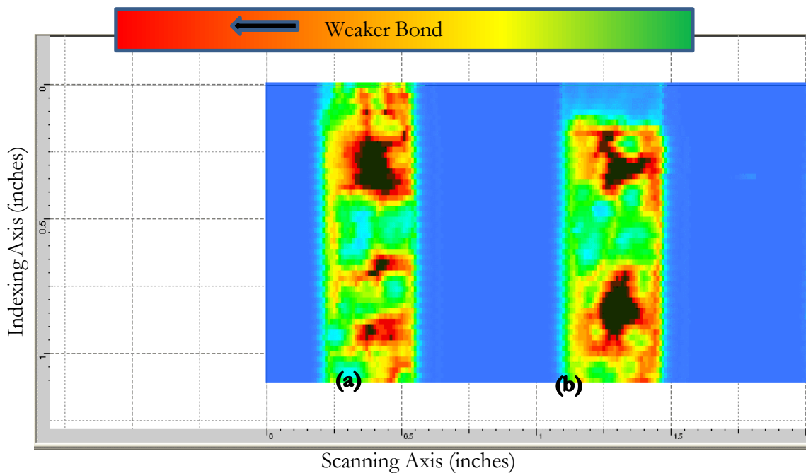
Figure 4.3: UT SLJ with Tape-Teflon Sandwich (Red regions have higher attenuations)
