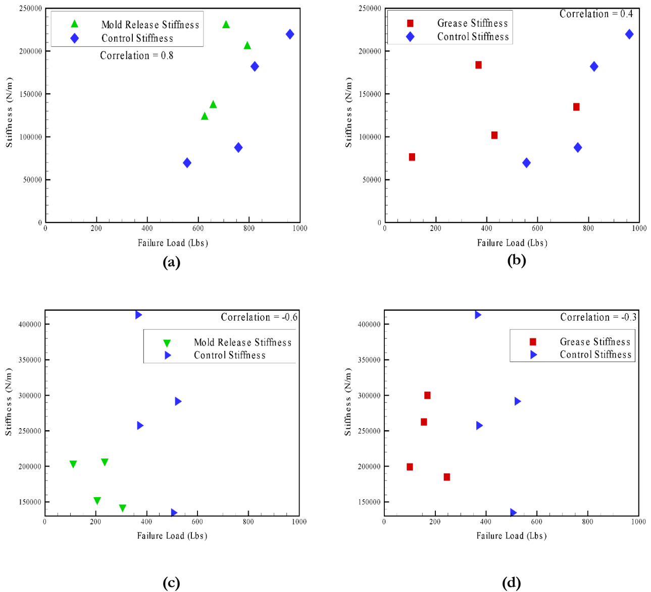
Figure 4.11: Stiffness vs Failure load for (a) Mold release (film) (b) Grease (film) (c) Paste mold release (d) Paste grease contamination
