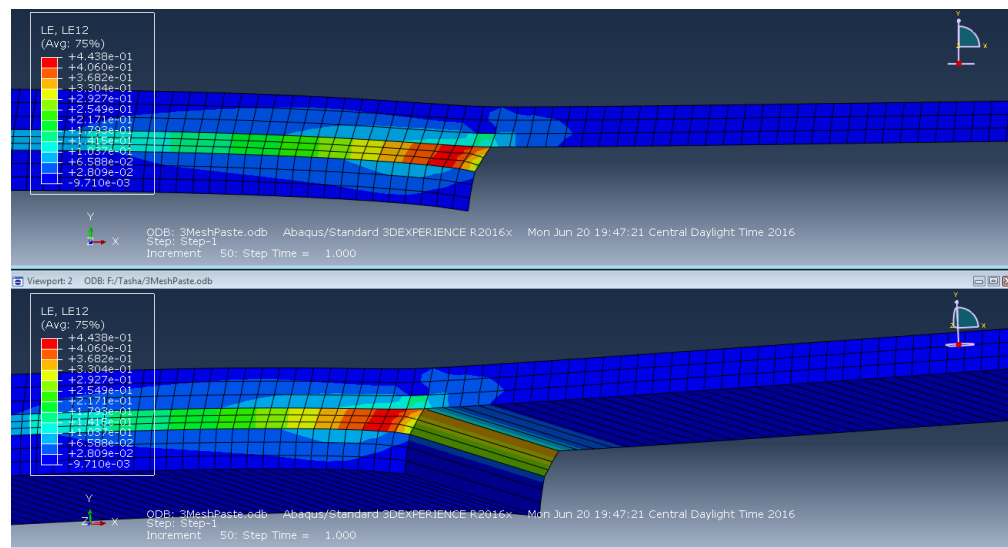
Figure 5.8: Shear Strain distribution for paste adhesive
