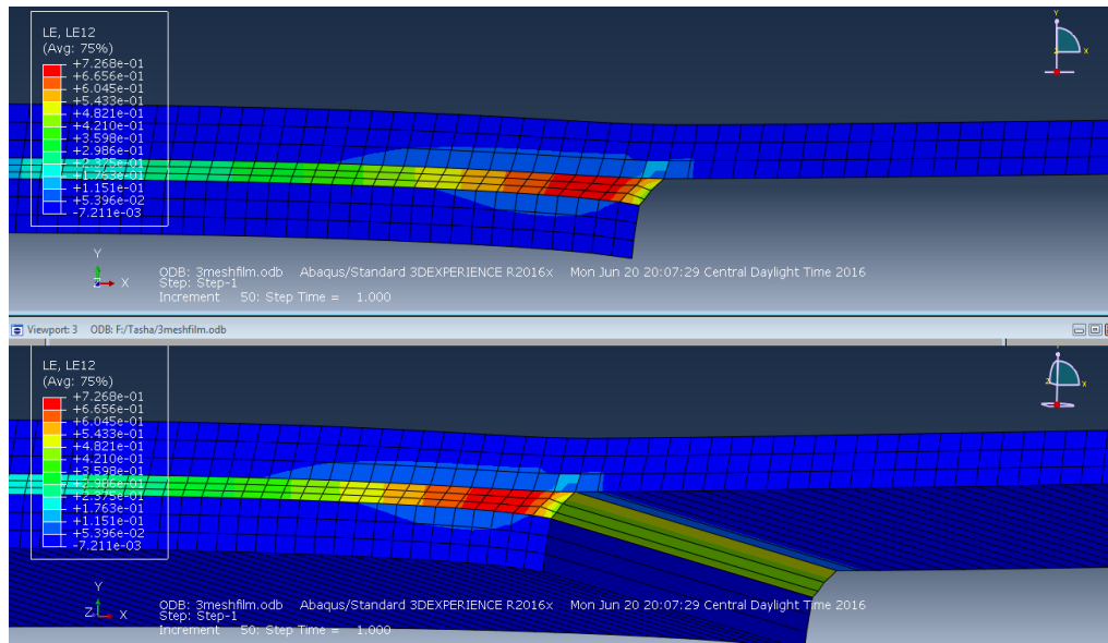
Figure 5.4: Shear strain distribution for film adhesive
