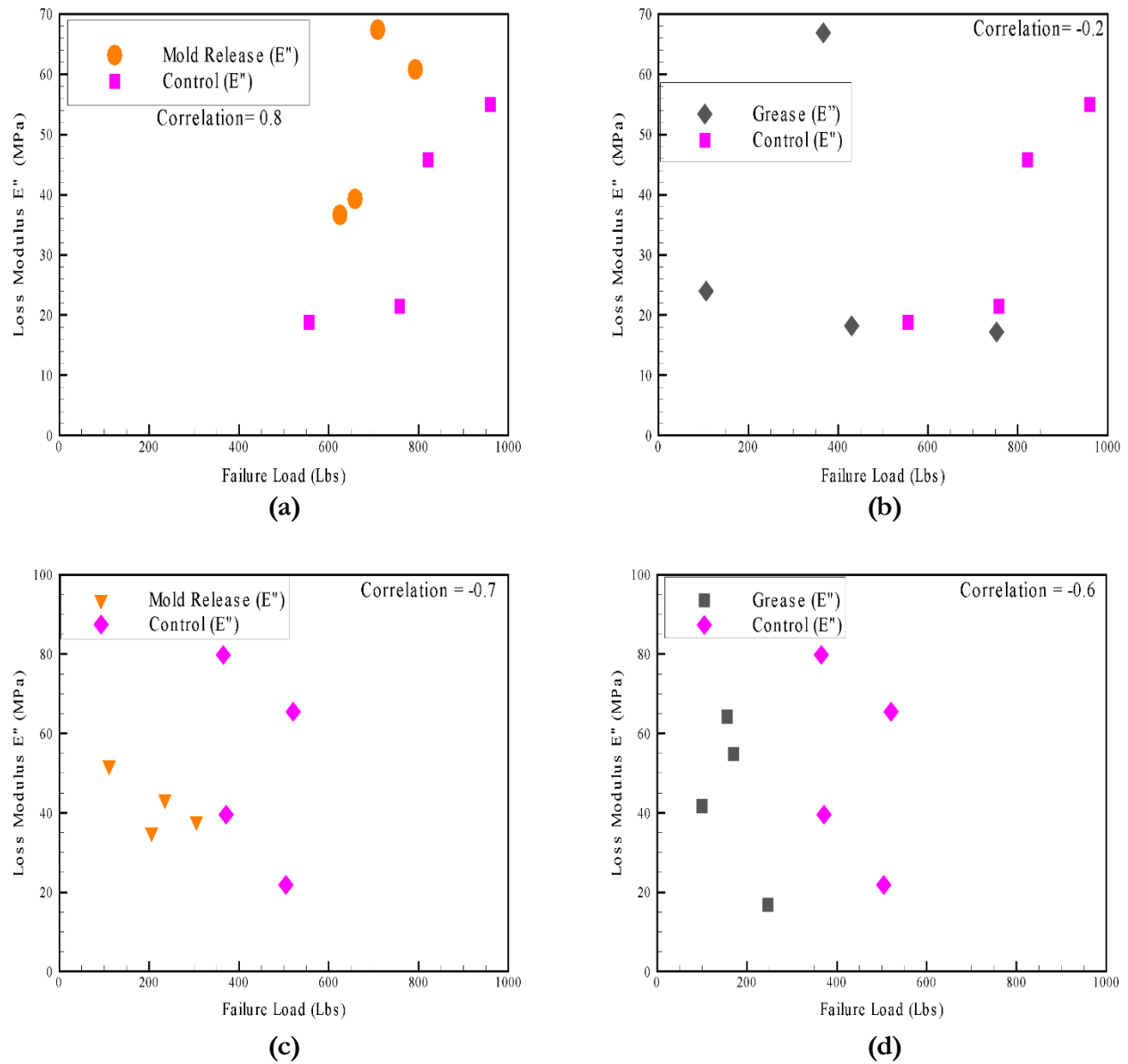
Figure 4.10: Loss Modulus vs Failure load for (a) Mold release film sample (b) Grease contamination film sample (c) Paste mold release sample, (d) Paste grease contamination
