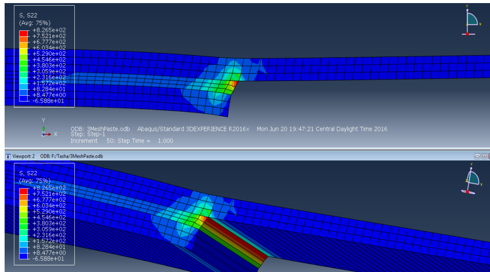
Figure 5.7: Peel stress distribution for paste
