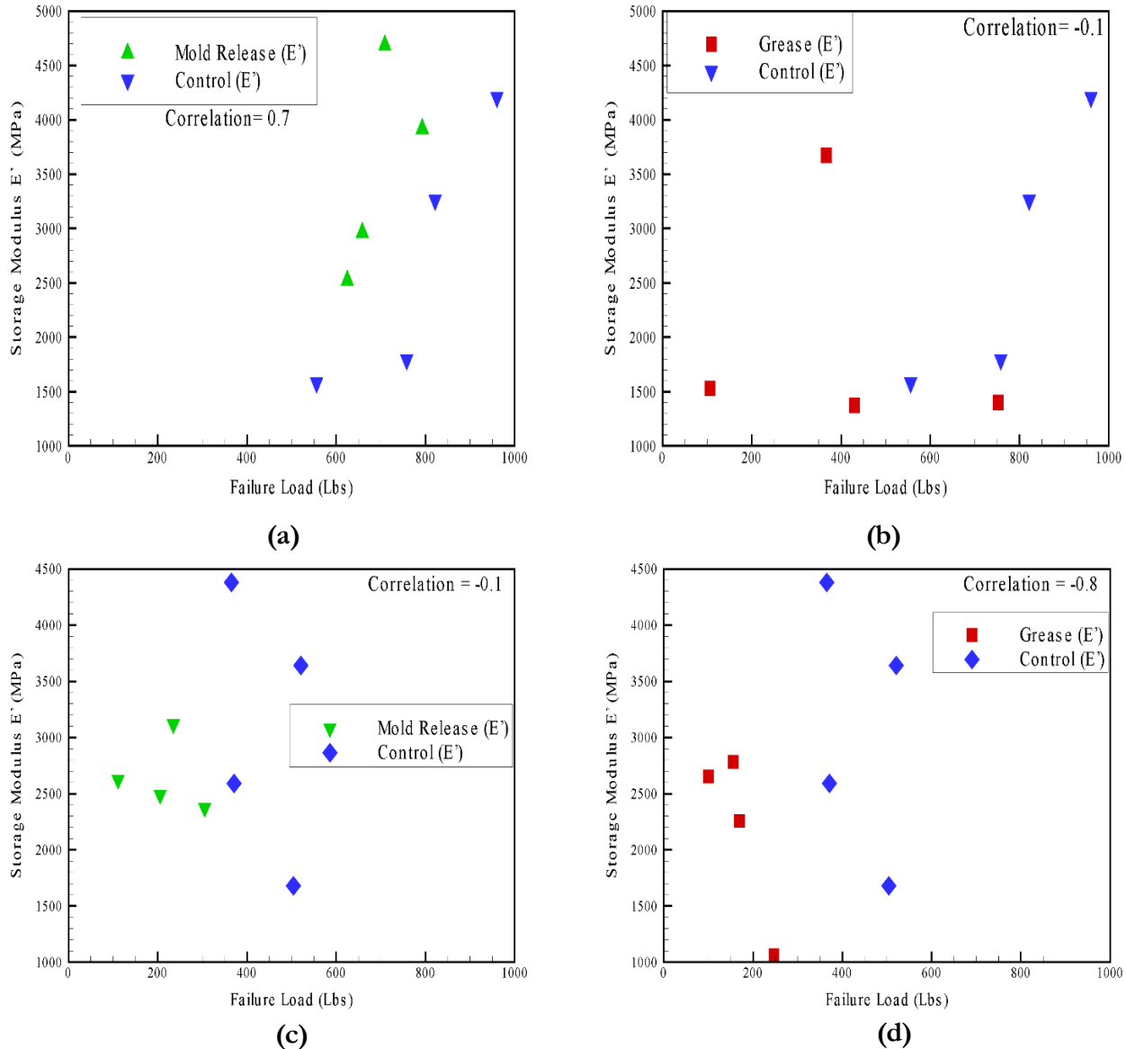
Figure 4.9: Storage Modulus E' vs Failure load for (a) Mold release film samples (b) Grease film samples (c) Paste mold release, (d) Paste grease contamination
