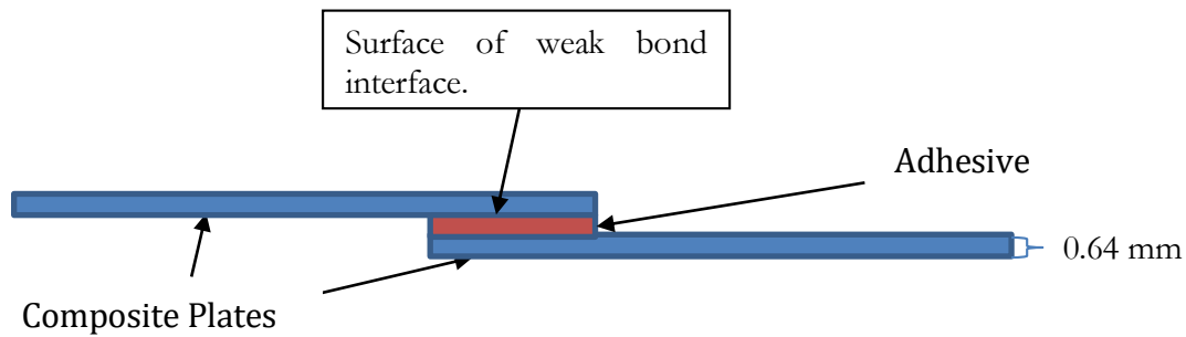
Figure 3.1: Schematic of Single Lap Joint Specimen
