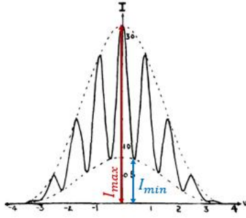
Figure 13 Fringe pattern of a Yong's double slit
