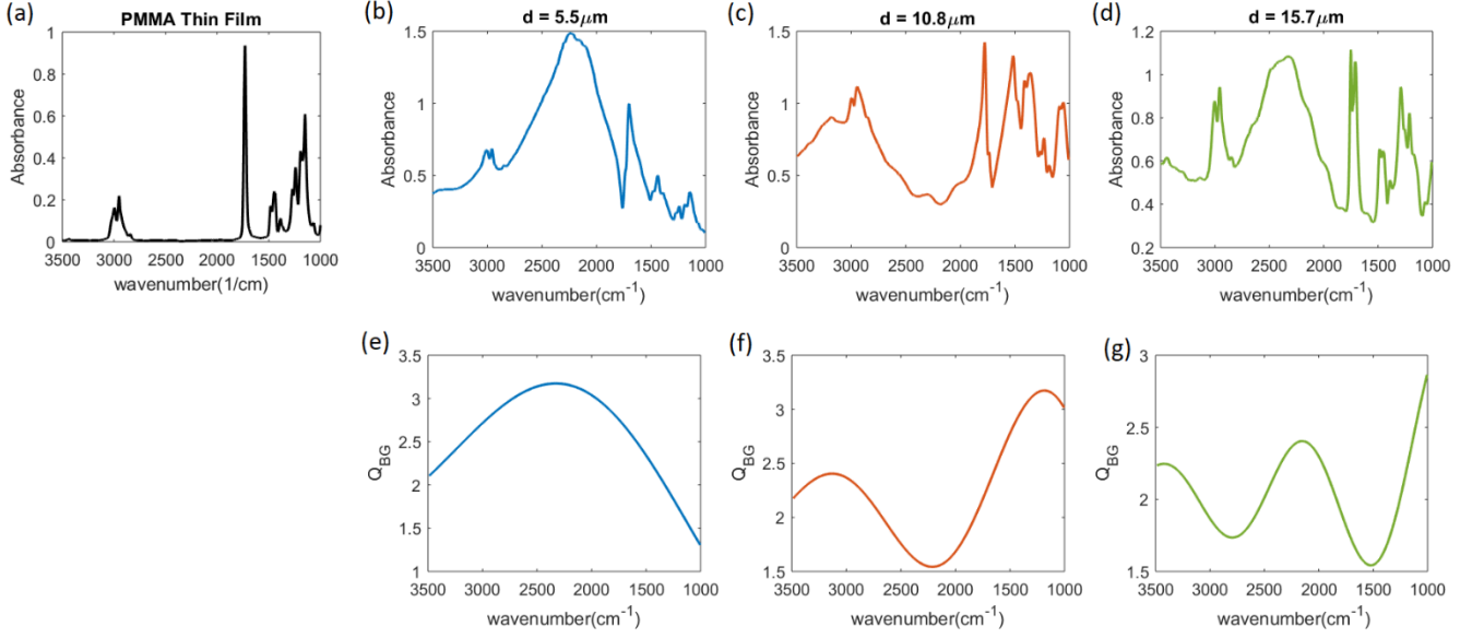
Figure 6 (a) shows absorbance spectra of a PMMA thin film, while Figure 5 (b) to (d) show spectra of PMMA beads with diameters of 5.5 \mu\text{m} , 10.8 \mu\text{m} , and 15.7 \mu\text{m} for a single detector.
