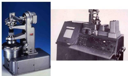
Figure 2 (a) One of the First Infrared spectrometers, Prototype Model 12 (1943) (Tisinger, 2018) (b) The first commercial IR micro spectrometer PE model 85 (1953) (Tisinger, 2018)
