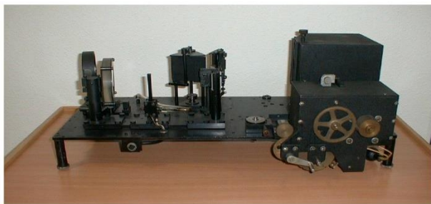
Figure 2 (a) One of the First Infrared spectrometers, Prototype Model 12 (1943) (Tisinger, 2018) (b) The first commercial IR micro spectrometer PE model 85 (1953) (Tisinger, 2018)
