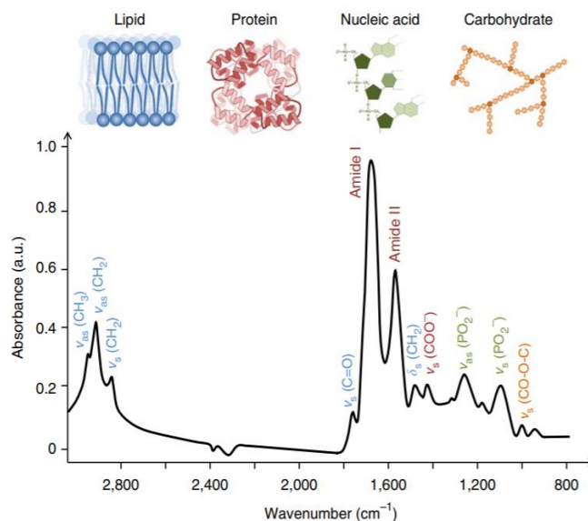
Figure 1 | Typical biological spectrum showing biomolecular peak assignments from 3,000–800 \text{cm}^{-1} , where \nu = stretching vibrations, \delta = bending vibrations, s = symmetric vibrations and as = asymmetric vibrations. The spectrum is a transmission-type micro-spectrum from a human breast carcinoma (ductal carcinoma in situ). The sample was cryosectioned (8 \mu\text{m} thick) and mounted on BaF2 slides (1 mm thick) before IR microspectroscopy. Equipment: Bruker IR scope II, circular diameter of aperture \sim 60 \mu\text{m} ; a.u., arbitrary units. (Baker, et al., Using
