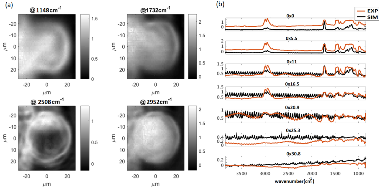
Figure 27 Measurement VS simulation, 25μm radius PMMA bead. (a) Projection Images measure at of 1148 \text{cm}^{-1} , 1732 \text{cm}^{-1} , 2508 \text{cm}^{-1} and 2952 \text{cm}^{-1} . (b) Simulated spectra compare to measure spectra of the 25μm radius PMMA bead. The x-y location of each spectrum is written on the title of the image.
