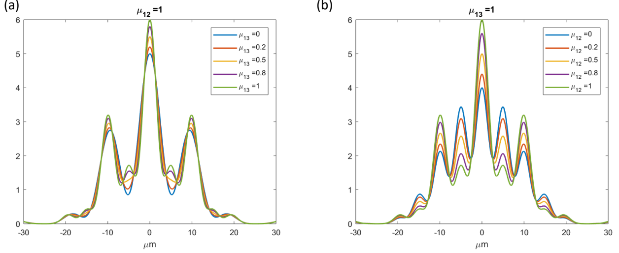
Figure 19 Interference pattern of 3 slits for slit width of 1.95 \mu\text{m} at \lambda = 4 \mu\text{m} . (a) 100% coherence between slit 1 and 2, while the coherence between slit 1 and 3 is increasing. (b) 100% coherence between slit 1 and 3, while the coherence between slit 1 and 2 is increasing.
