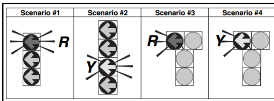
Figure 2-5. Scenarios Evaluated in Previous Research Study Conducted to Analyze Impacts of FYA at Intersections with Wide Medians [12]
