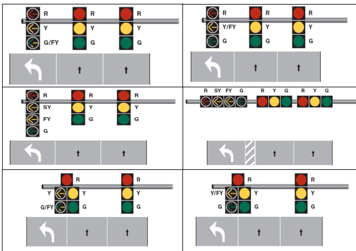
Figure 3-1. FYA Signal Displays to be Evaluated
