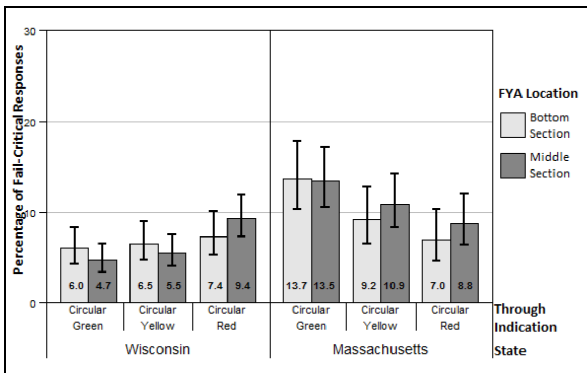
Figure 4-4. Percentage of Fail-Critical Responses for FYA Location Comparisons based on Through Indication
