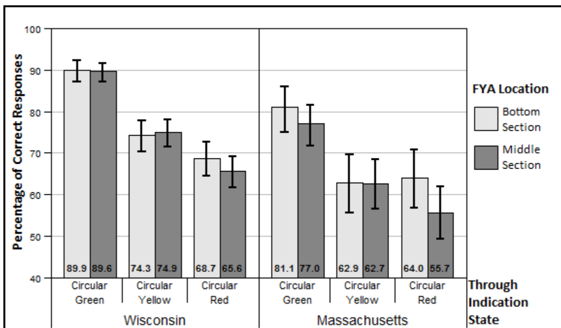
Figure 4-3. Percentage of Correct Responses for FYA Location Comparisons based on Through Indication
