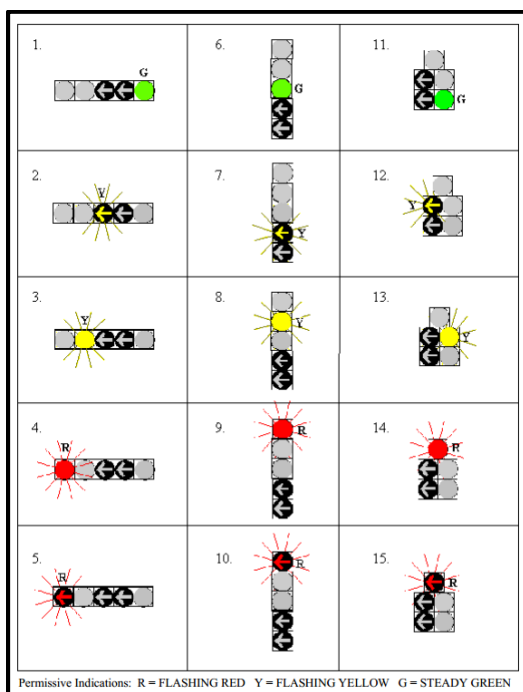
Figure 2-4. Scenarios Evaluated in Previous Research Study Conducted to Analyze Impacts of Various FYA Arrangements [11]
