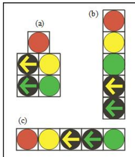
Figure 2-1. Five-Section PPLT Signal Displays (a) Five-Section Cluster, (b) Five-Section Vertical, and (c) Five-Section Horizontal Signal Displays
