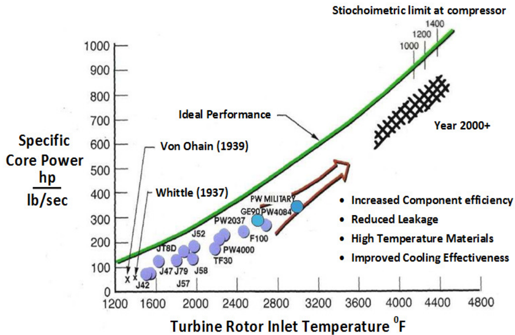
Figure 2.2: Specific core power with turbine rotor inlet temperature Reference: http://mit.edu/16.unified/www/FALL/thermodynamics/notes/node28.html
