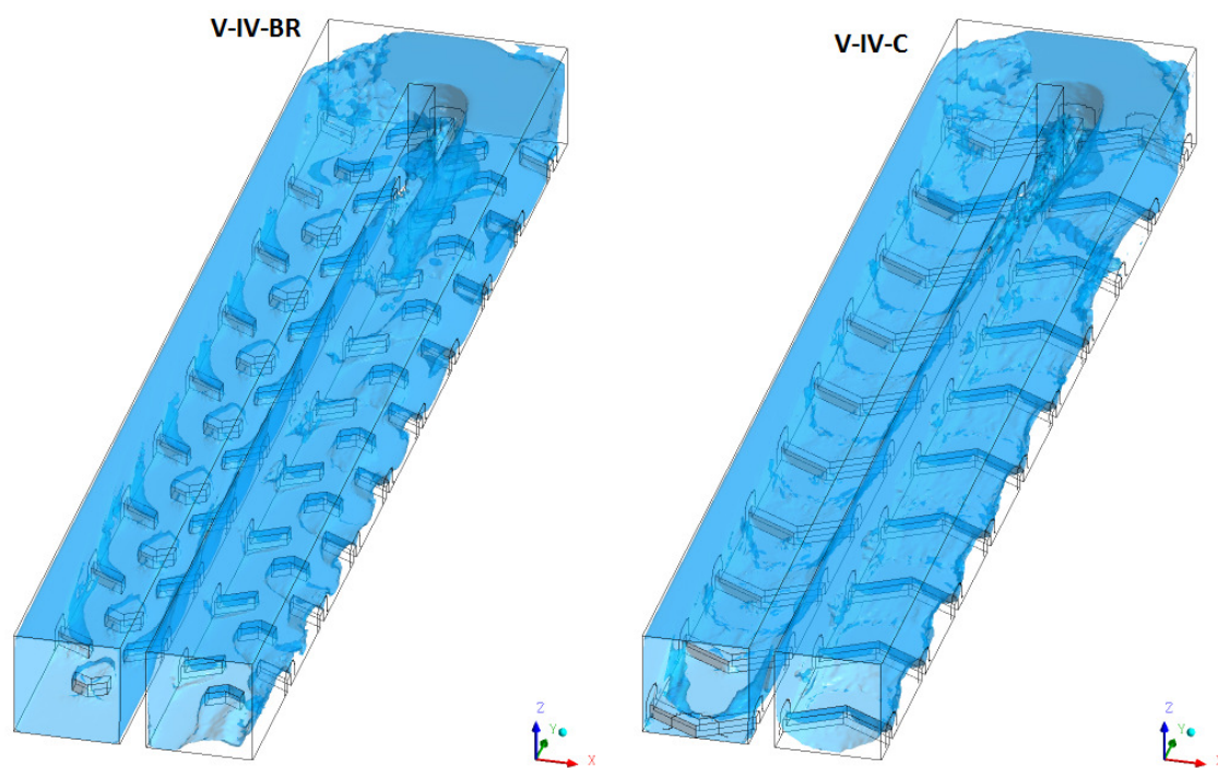
Figure 7.23: Isosurface for Velocity: 8.2 \text{ m/s} ( Re = 56000 )
