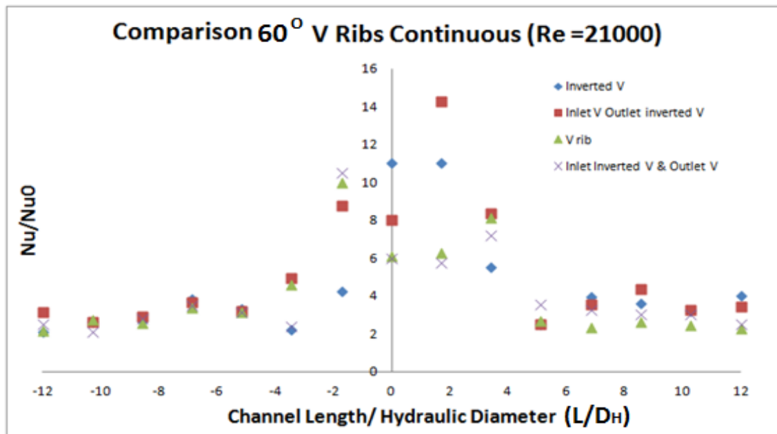
Figure 5.5 Comparison of continuous rib Nusselt Number @ Re =21000
