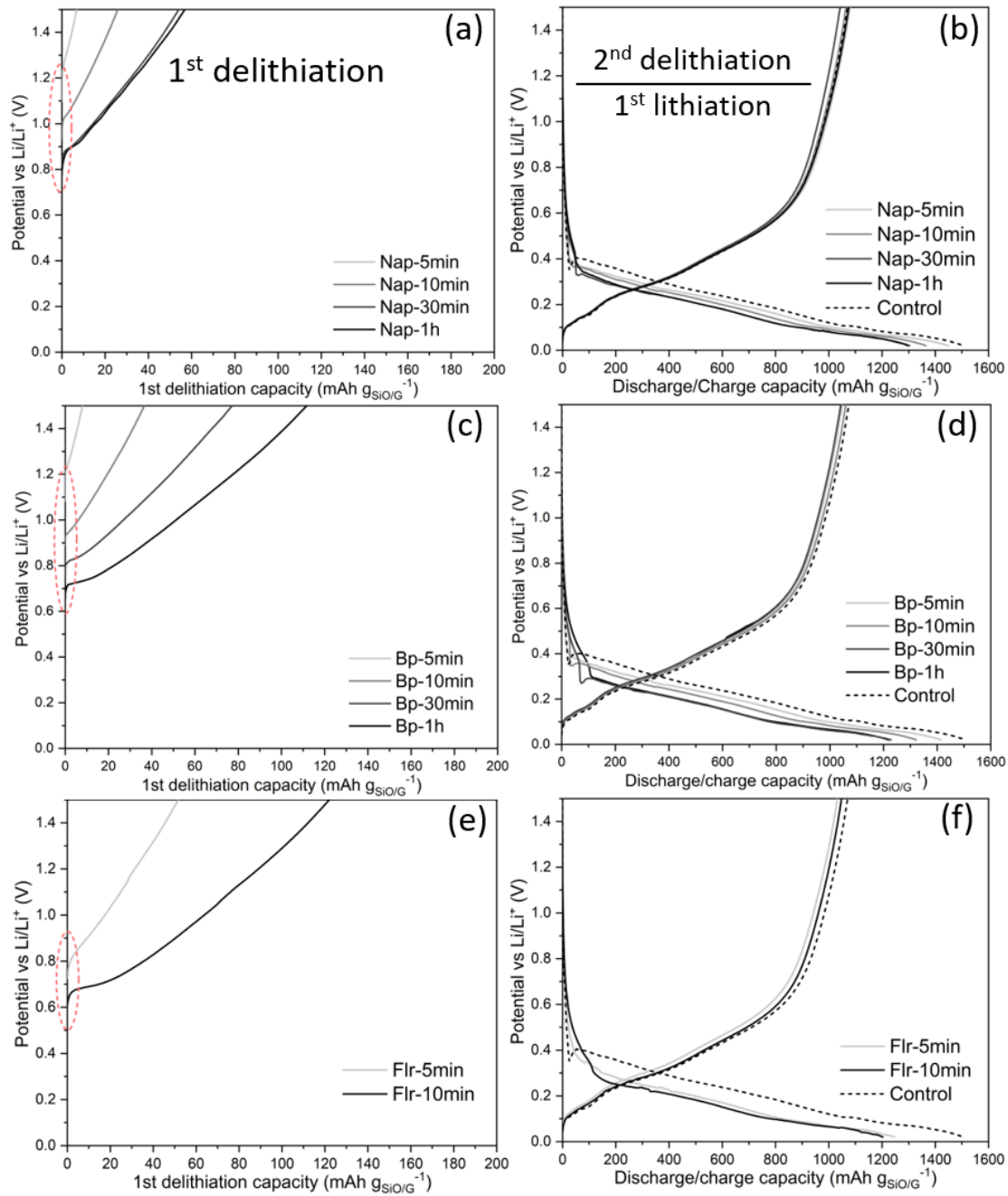
Figure 3-18. 1 st delithiation and following lithiation/delithiation curves of SiO/G electrodes in half-cell format prelithiated using Li–Nap–THF (a, b), Li–Bp–THF (c, d), and Li–Flr–THF (e, f) with different immersion time. 1 st lithiation/delithiation curves of control sample are shown in b, d, and f for comparison. The OCPs are circled with a dashedline in a, c and e.
