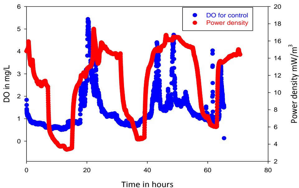
Figure 13: Effect of DO for Control SMFC
