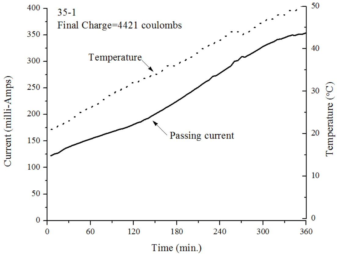
Figure A.31: The picture and graph of passing current/temperature vs. time for sample35-1.
