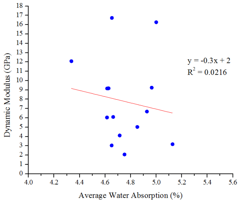
Figure 4.20: The relationship between dynamic modulus and average water absorption of disc.
