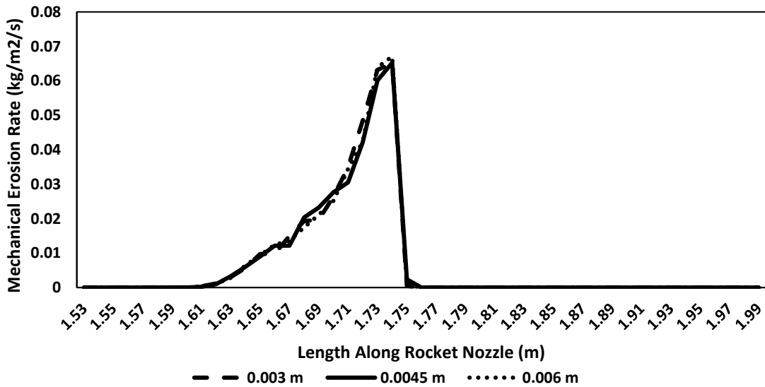
Figure 5-5: Mechanical Erosion Rate Using Neilson Correlation for different cell sizes in the radial direction
