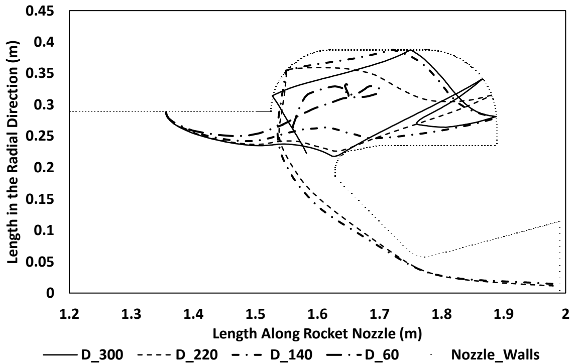
Figure 7-17: Parcel No. 700 trajectories within the chamber at different droplet's sizes.
