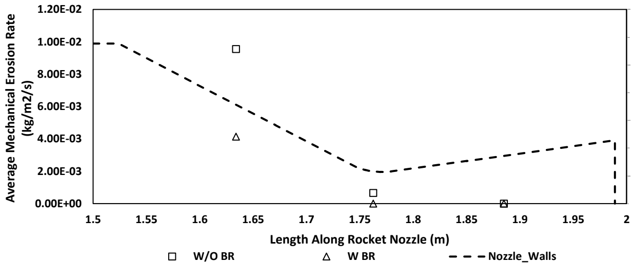
Figure 6-1: Mechanical erosion rate comparison with Thakre et al [41] results.
