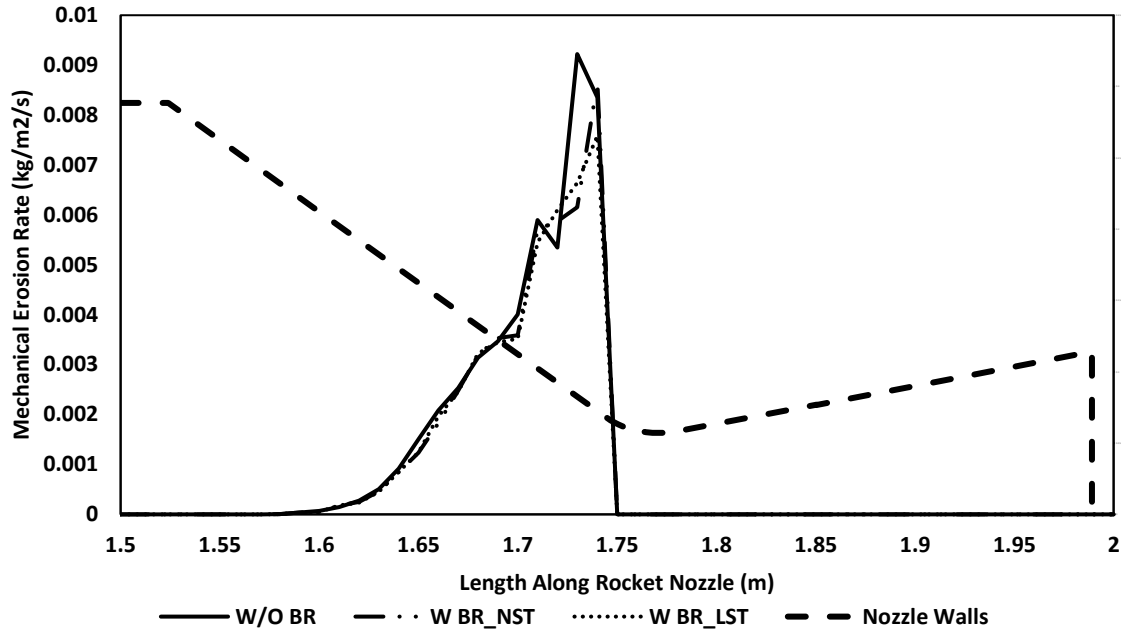
Figure 5-31: Erosion rate at different conditions for 60 μm droplet size
