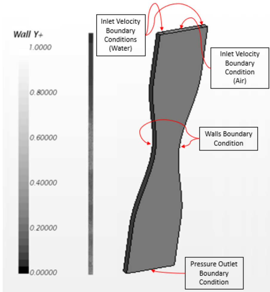
Figure 4-1: The numerical model computational domain (C-D Nozzle) and Y+ distribution over the wall
