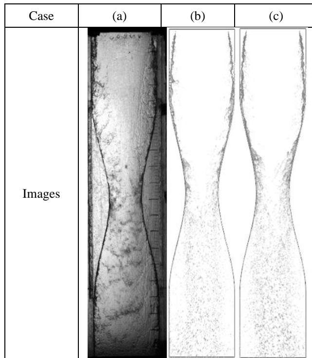
Figure 4-14: The breakup shape pattern at air velocity of 40 m/s, (a) Experiment with NWST, (b) Simulation with NWST and (c) Simulation with RWST
