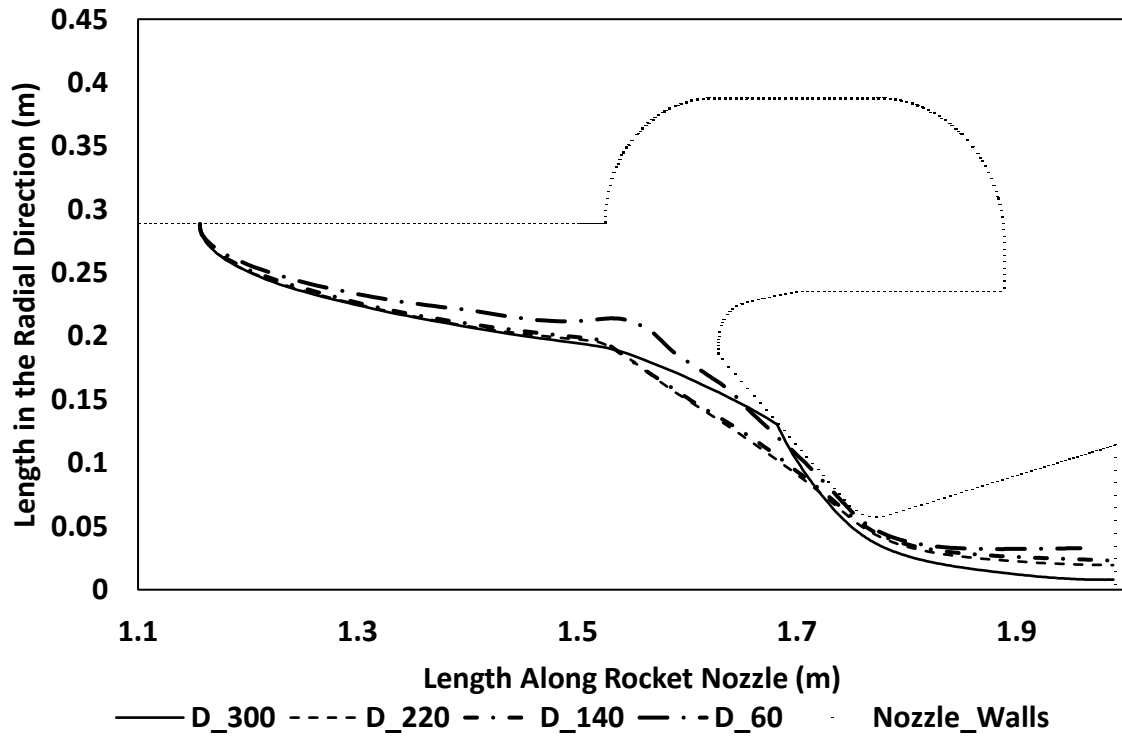
Figure 7-19: Parcel No. 1500 trajectories within the chamber at different droplet's sizes.
