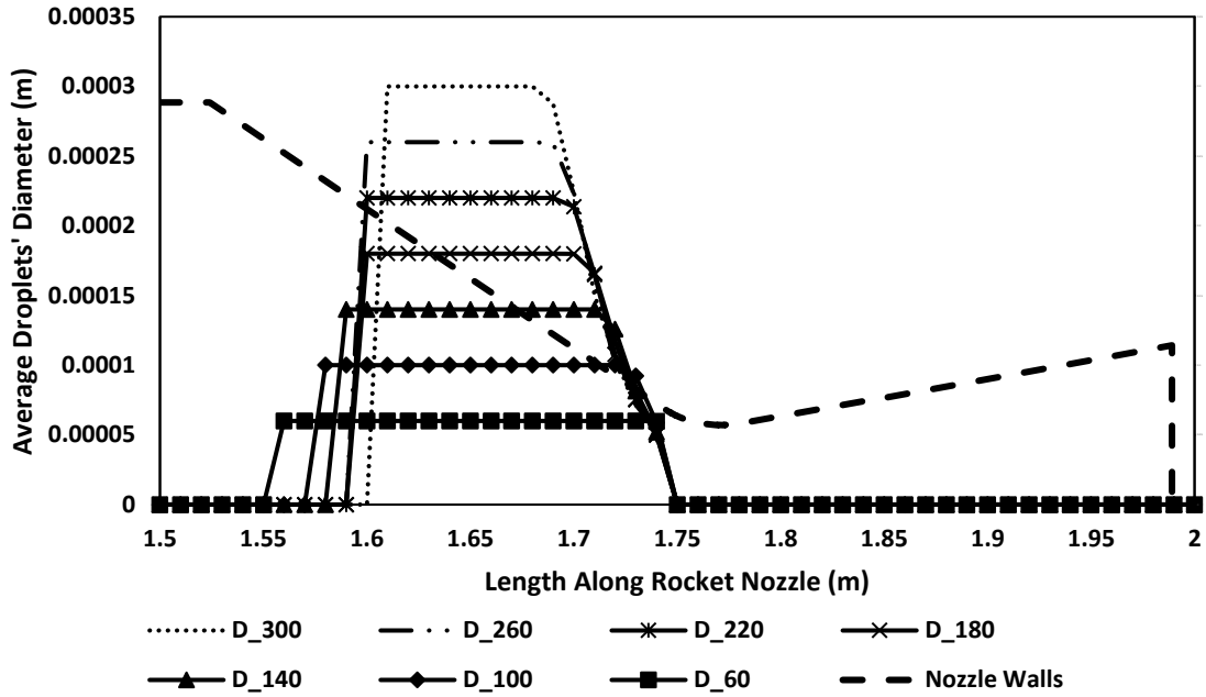
Figure 5-27: Average droplets' diameter at different droplet's sizes after applying the break-up model
