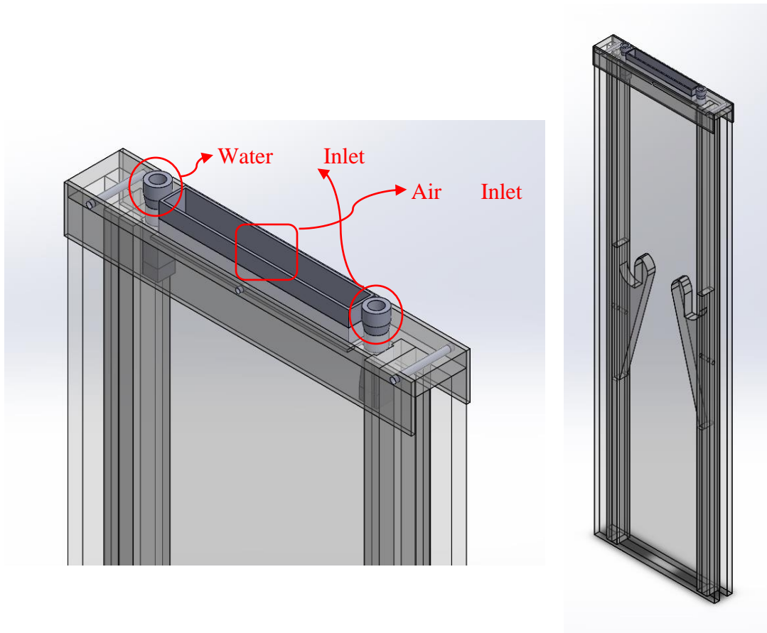
Figure 3-7: New experimental set-up with the submerged nozzle configuration
