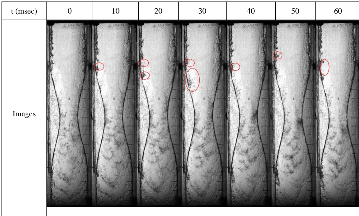
Figure 4-5: Experimental results for air velocity, 30 m/s and normal water (surface tension 0.072 N/m)
