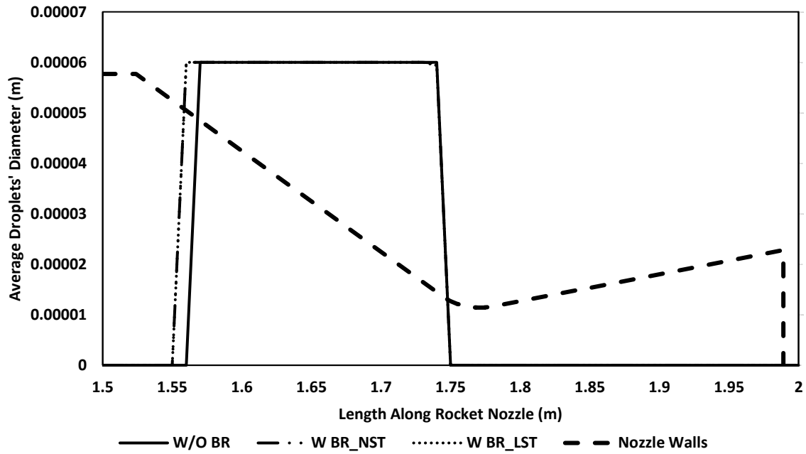
Figure 5-32: Average droplets' diameter at different conditions for 60 μm droplet size
