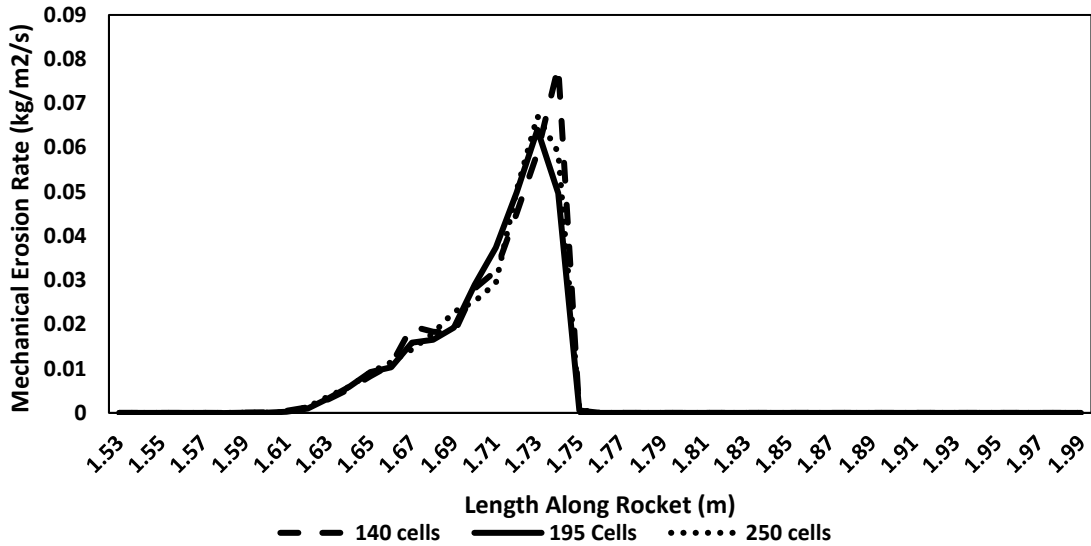
Figure 5-4: Mechanical Erosion Rate Using Neilson Correlation for different cells count in the axial direction
