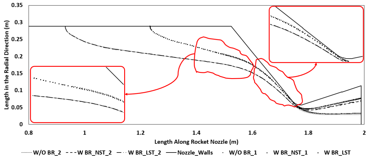
Figure 5-34: Two different parcels trajectories within the chamber for 60 \mu\text{m} droplet size
