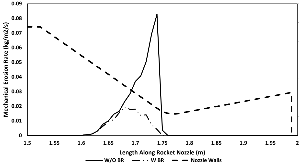
Figure 6-9: Erosion rate over the nozzle length at the 27% propellant aluminum content case
