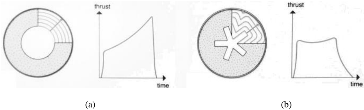
Figure 1-2: Propellant grain cross sections, [2].
