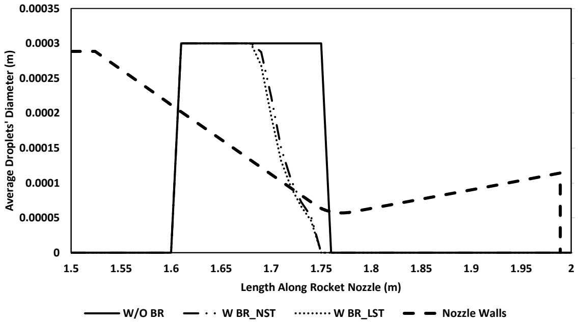
Figure 5-30: Average droplets' diameter at different conditions for 300 μm droplet size
