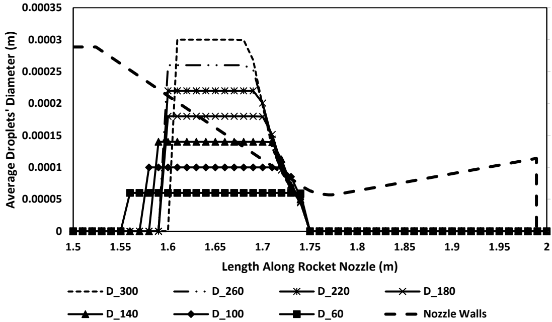
Figure 5-36: Average droplets' diameter at droplet's different sizes and lower surface tension
