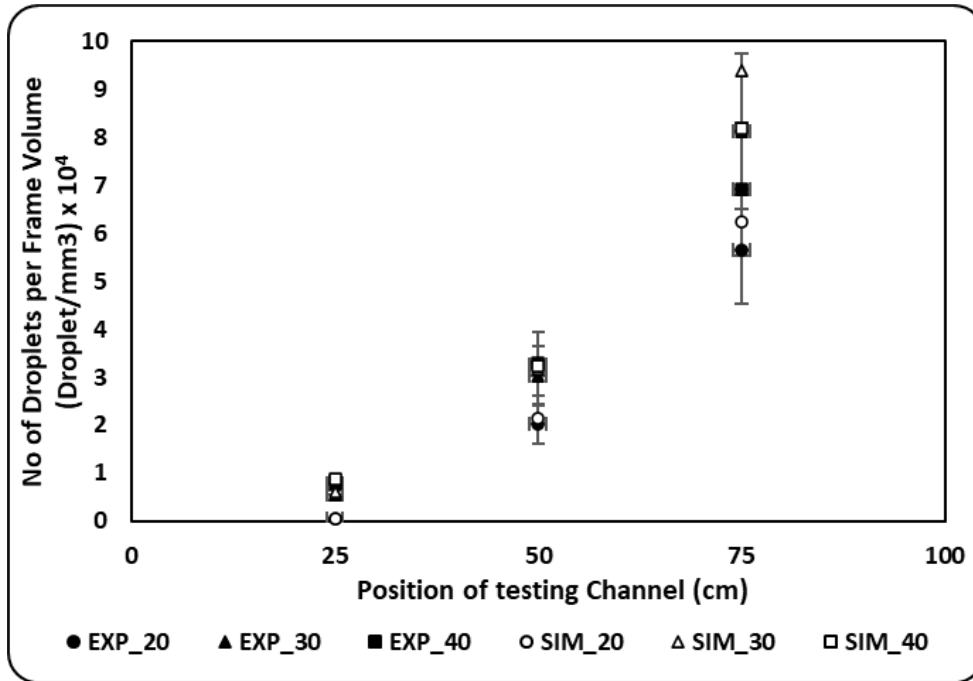
Figure 4-10: Experimental and numerical number of droplets at different sections of the testing channel and different air velocities.
