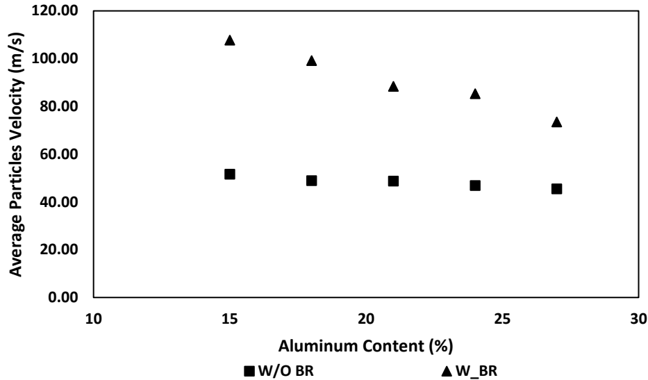
Figure 6-5: Average droplets' relative velocity at different propellant aluminum contents
