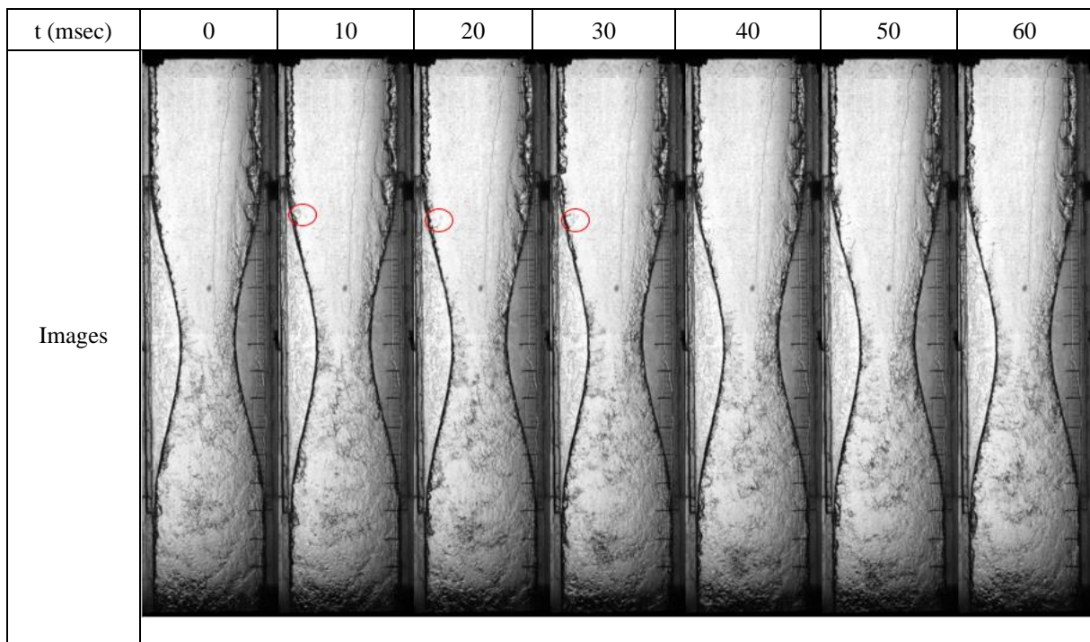
Figure 4-4: Experimental results for air velocity, 20 m/s and normal water (surface tension 0.072 N/m)
