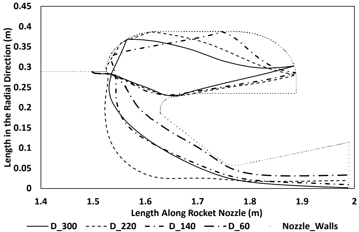
Figure 7-16: Parcel No. 200 trajectories within the chamber at different droplet's sizes.
