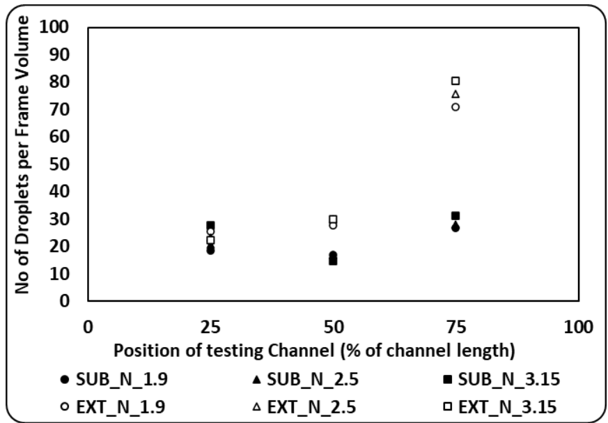
Figure 4-40: Droplets' number at different water flow rates and different sections through the testing channel
