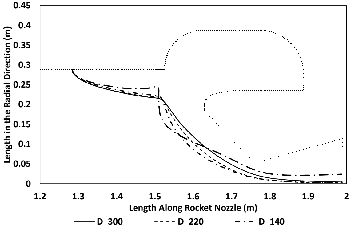
Figure 7-18: Parcel No. 1200 trajectories within the chamber at different droplet's sizes.
