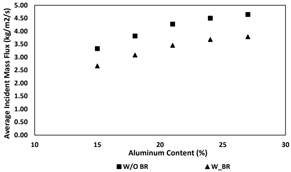
Figure 6-4: Average incident mass flux at different propellant aluminum contents
