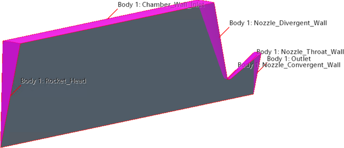
Figure 5-2: Numerical Computational Domain
