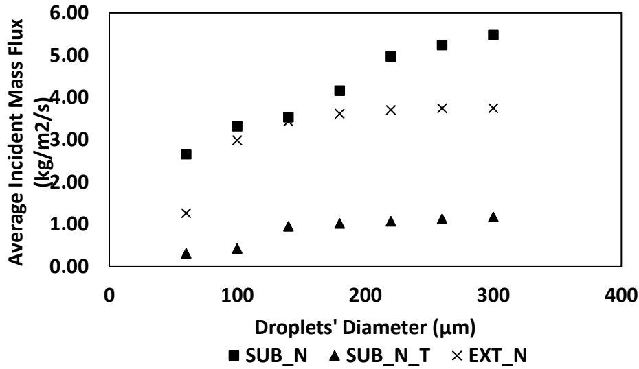
Figure 7-11: Average incident mass flux at different droplet's sizes
