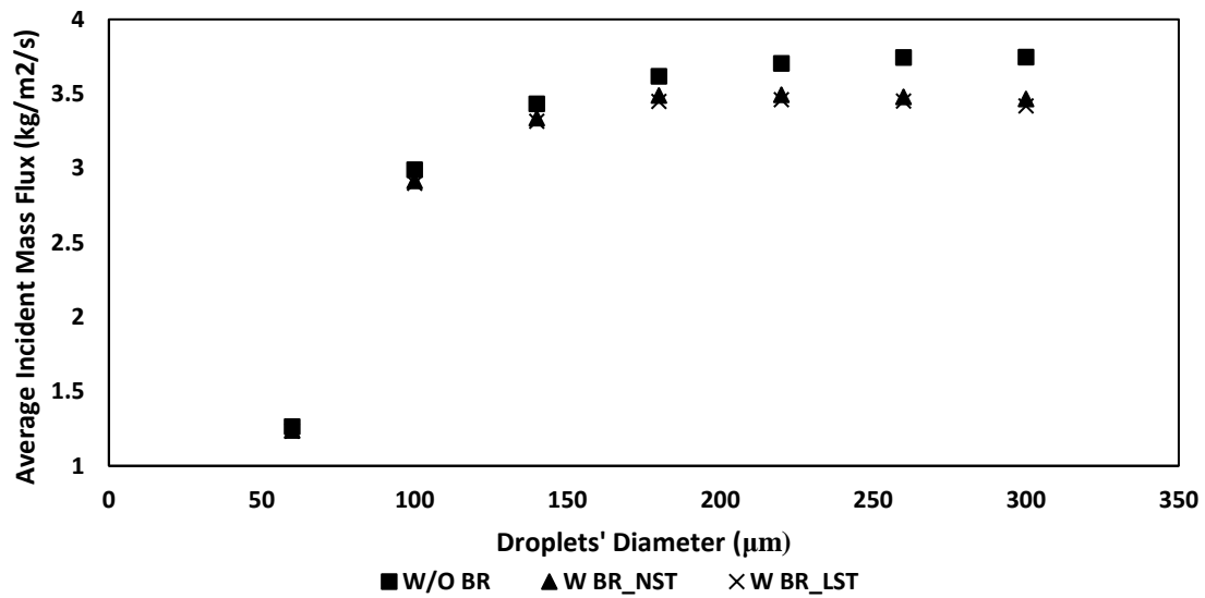
Figure 5-20: Average incident mass flux on the nozzle's convergent section at different droplet's sizes
