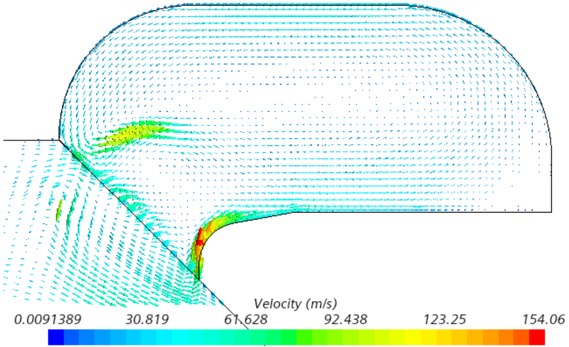
Figure 7-6: Combustion chamber pocket region velocity vectors
