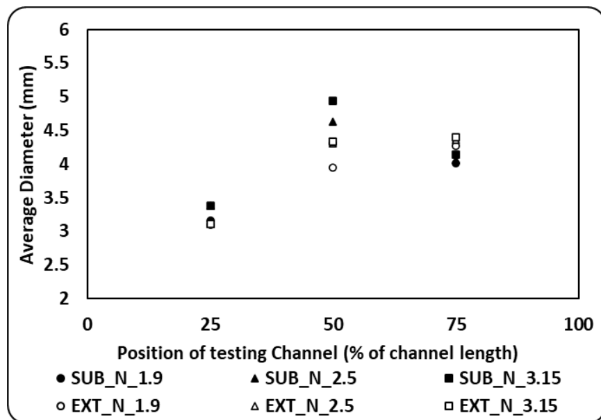
Figure 4-39: Droplets' average diameter at different water flow rates and different sections through the testing channel
