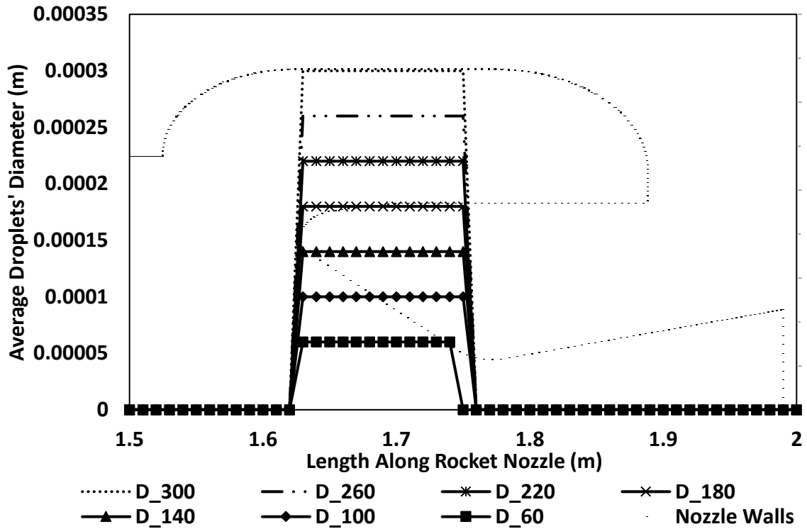
Figure 7-14: Average droplets' diameter at different droplet's sizes
