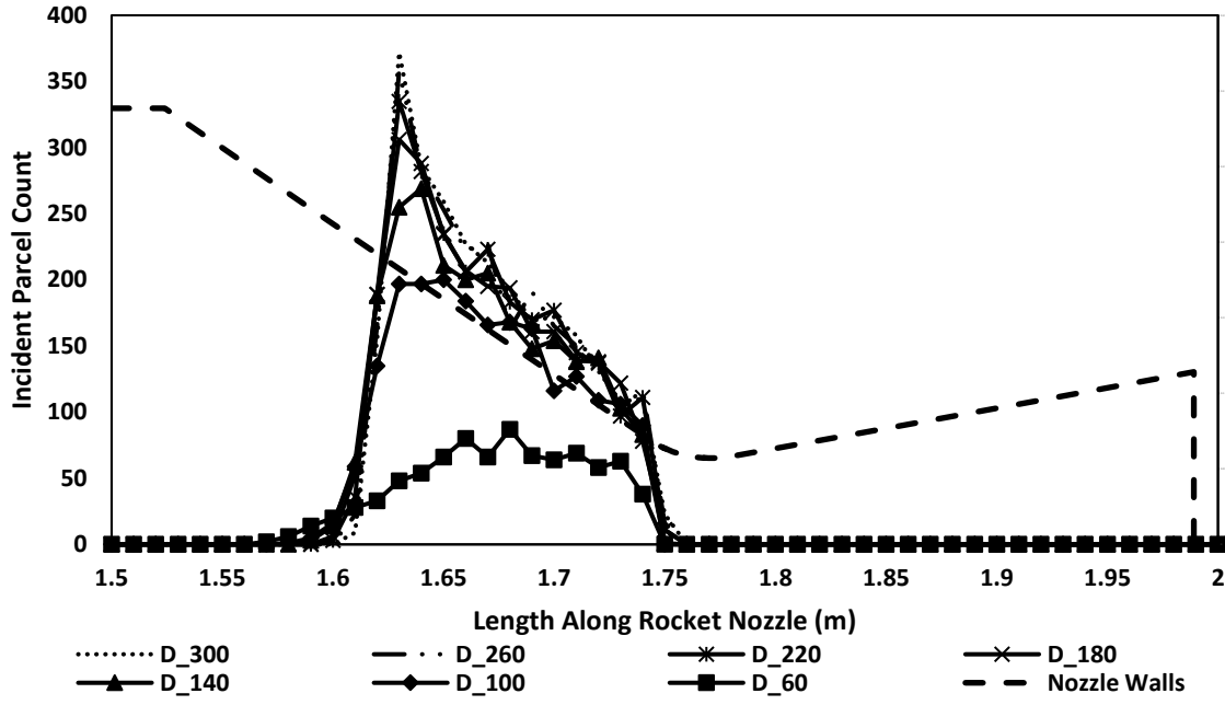
Figure 5-25: Incident parcels count at different droplet's sizes before applying the break-up model
