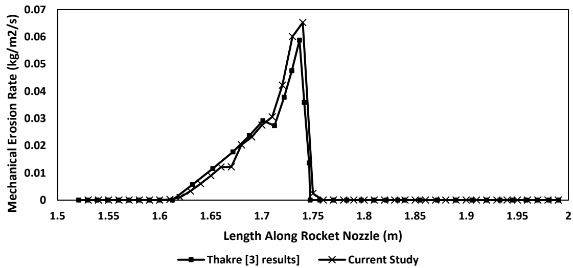
Figure 5-16: Mechanical erosion rate validation against Thakre et al [41].
