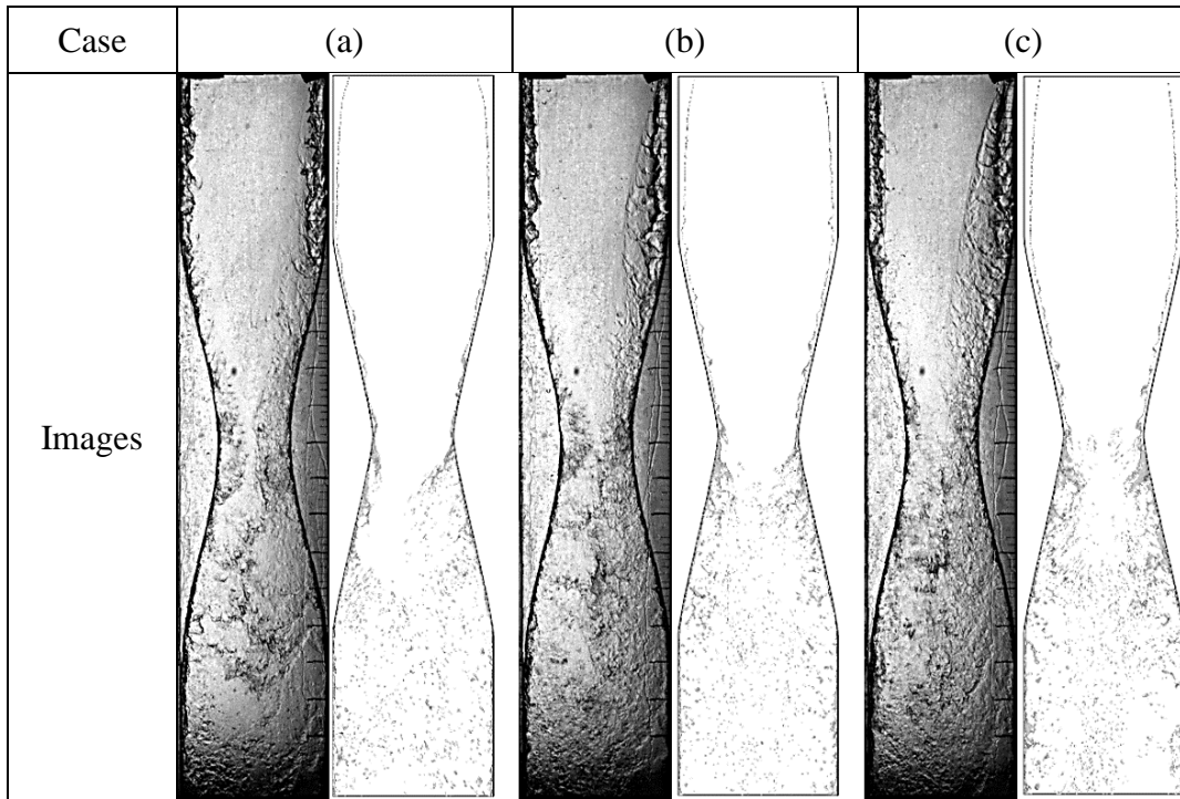
Figure 4-22: Comparison between the experimental (left) and numerical (right) break-up pattern shapes for different water flow rate, (a) 1.9 * 10^{-4} \text{ m}^3/\text{s} , (b) 2.5 * 10^{-4} \text{ m}^3/\text{s} , and (c) 3.15 * 10^{-4} \text{ m}^3/\text{s}
