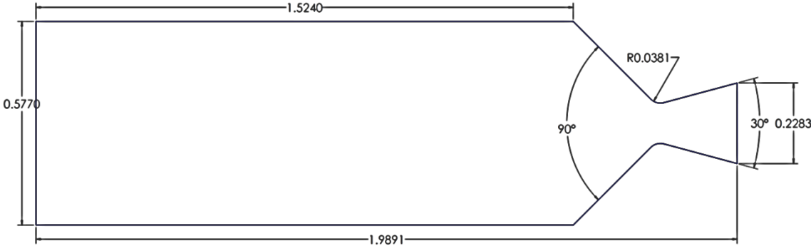
Figure 5-1: BATES geometry schematic
