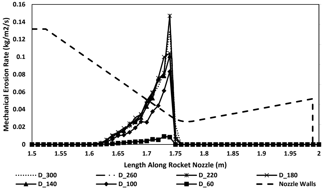
Figure 5-23: Mechanical erosion rate at different droplet's sizes before applying the break-up model
