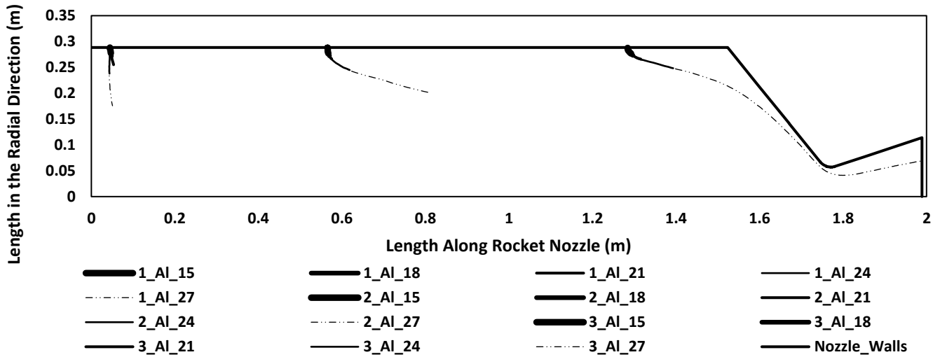
Figure 6-6: Three different parcels trajectories within the chamber at different propellant aluminum contents.
