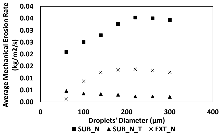
Figure 7-10: Average erosion rate at different droplet's sizes
