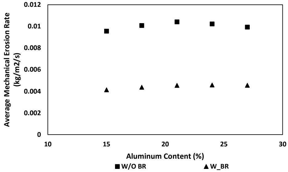
Figure 6-3: Average erosion rate at different propellant aluminum contents
