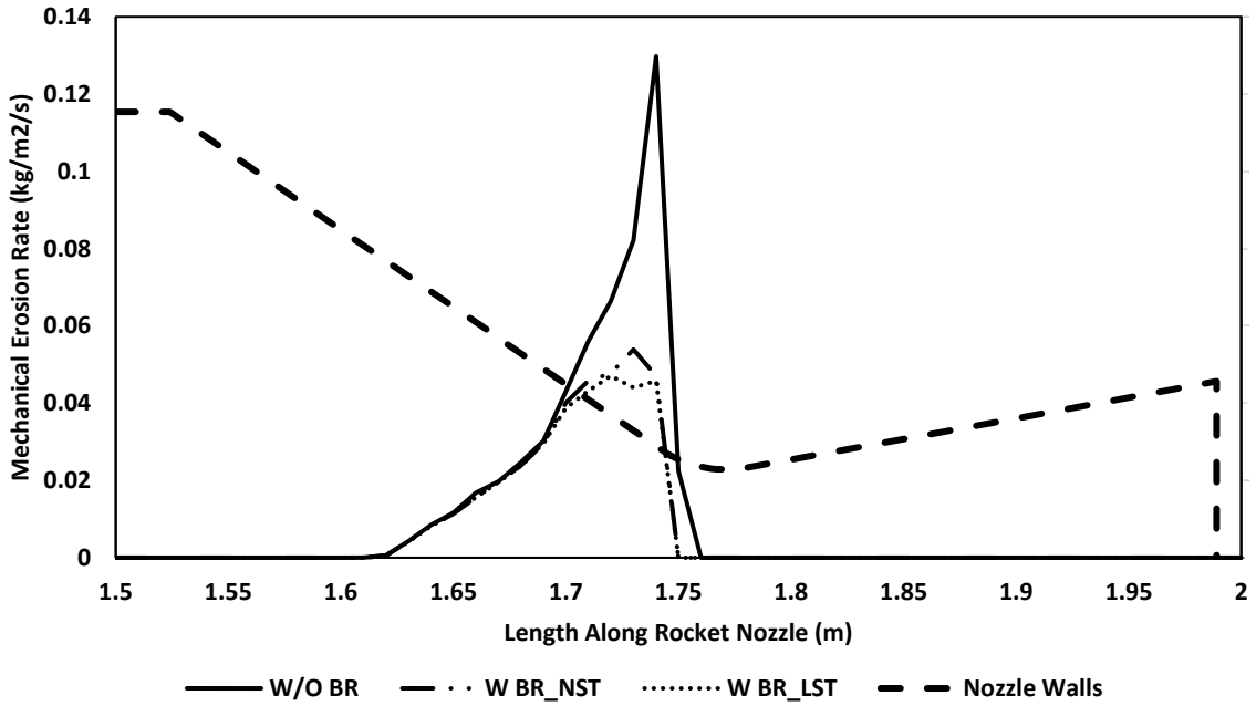
Figure 5-29: Erosion rate at different conditions for 300 μm droplet size
