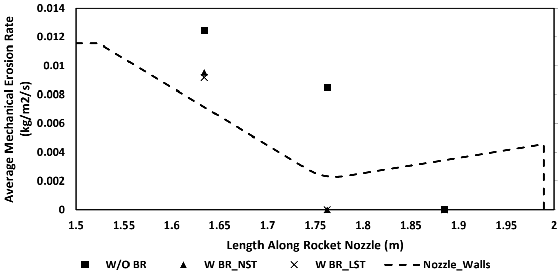
Figure 5-18: Average erosion rate over different sections of the nozzle for 300 μm droplet size
