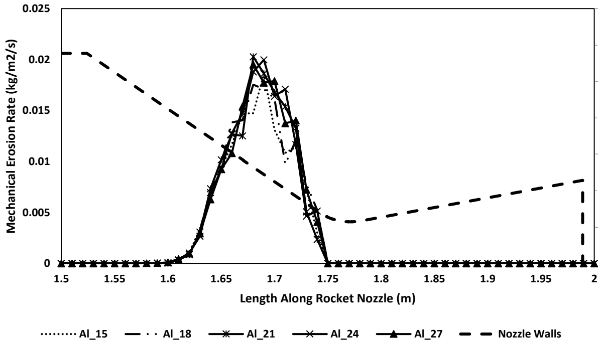
Figure 6-7: Mechanical erosion rate over the nozzle length at different propellant aluminum contents before applying the break-up model
