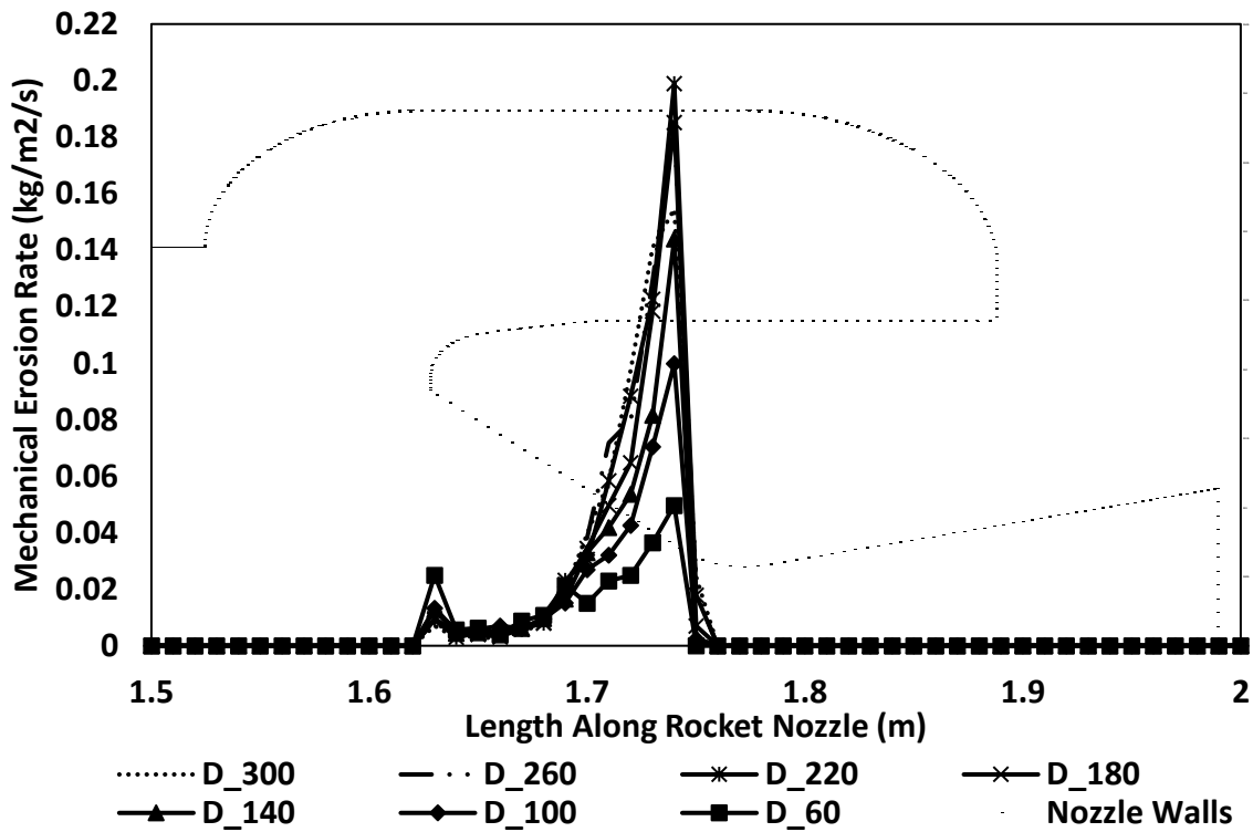
Figure 7-13: Local mechanical erosion rate at different droplet's sizes
