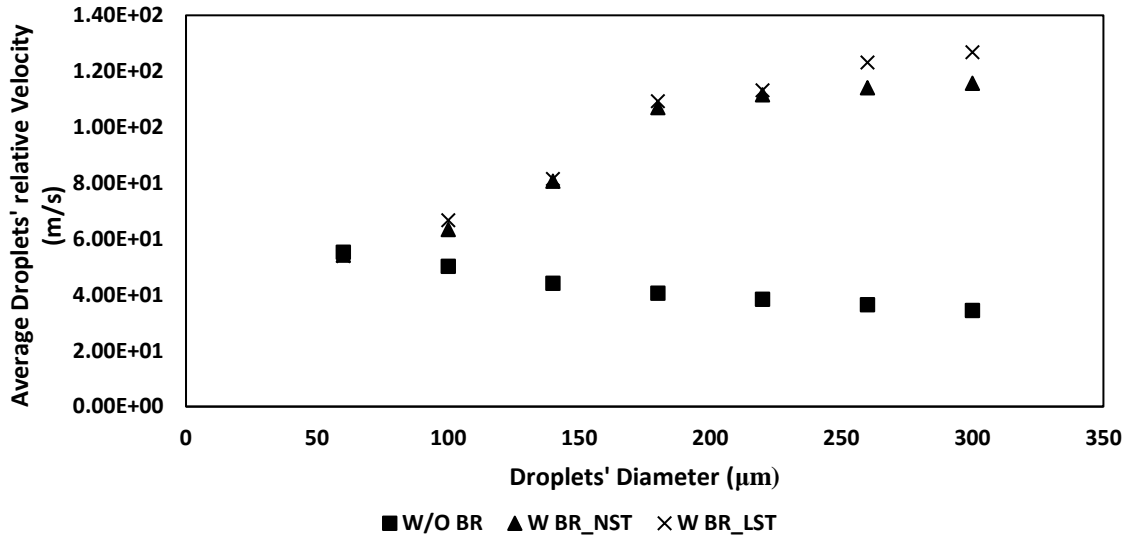
Figure 5-21: Average droplets' relative velocity on the nozzle's convergent section wall at different droplet's sizes
