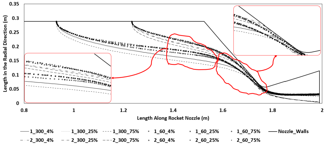
Figure 6-13: Two different parcels trajectories within the chamber for 300 μm, 60 μm droplet sizes and different injection velocities before applying the breakup model.
