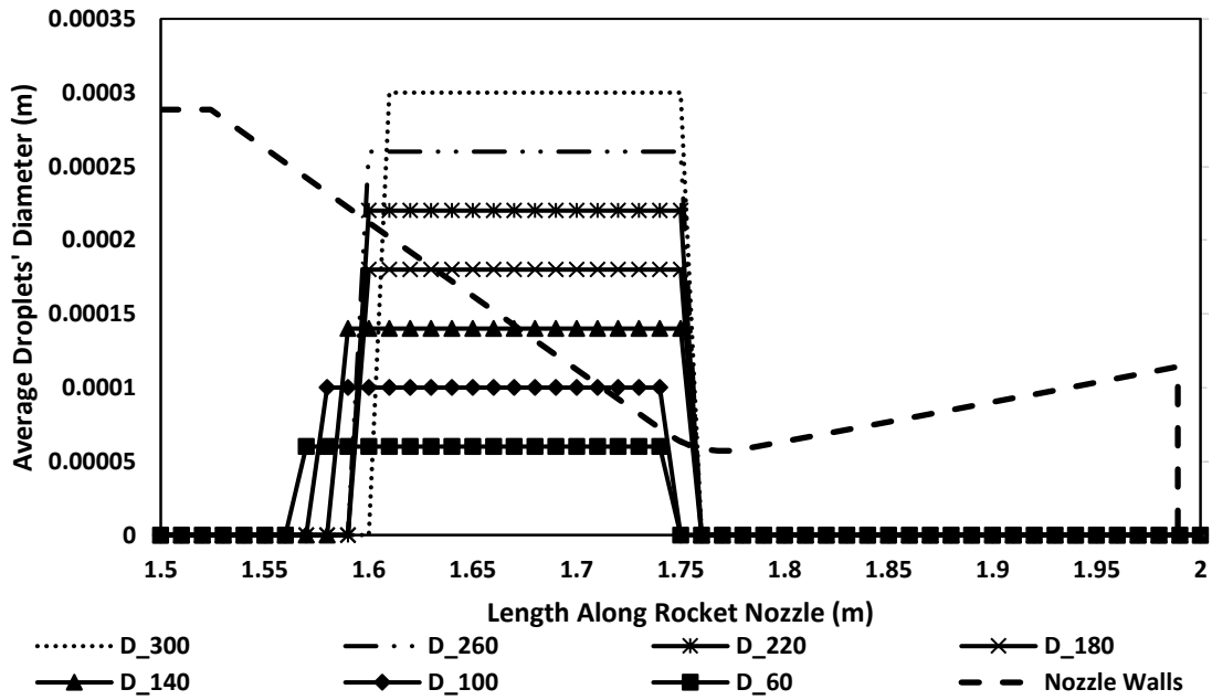
Figure 5-24: Average droplets' diameter at different droplet's sizes before applying the break-up model
