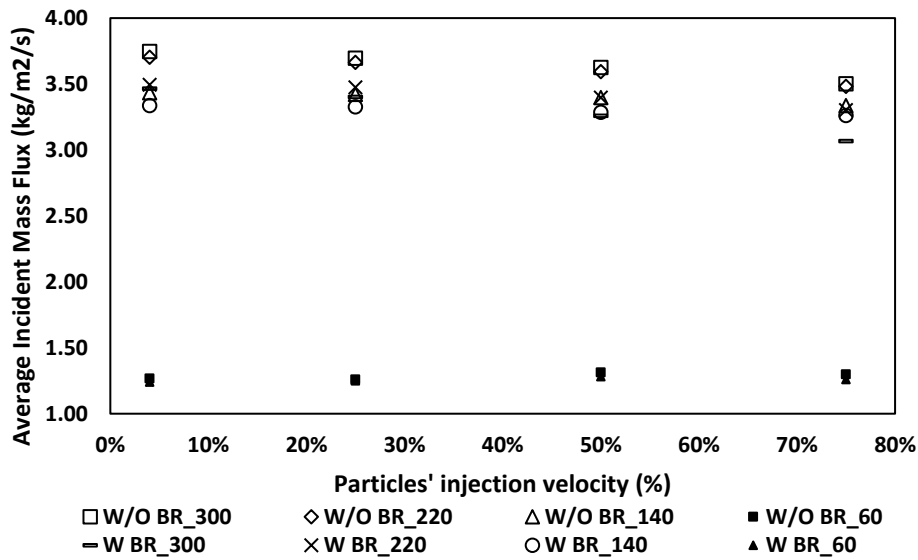
Figure 6-11: Average incident mass flux for variable particles' injection velocity
