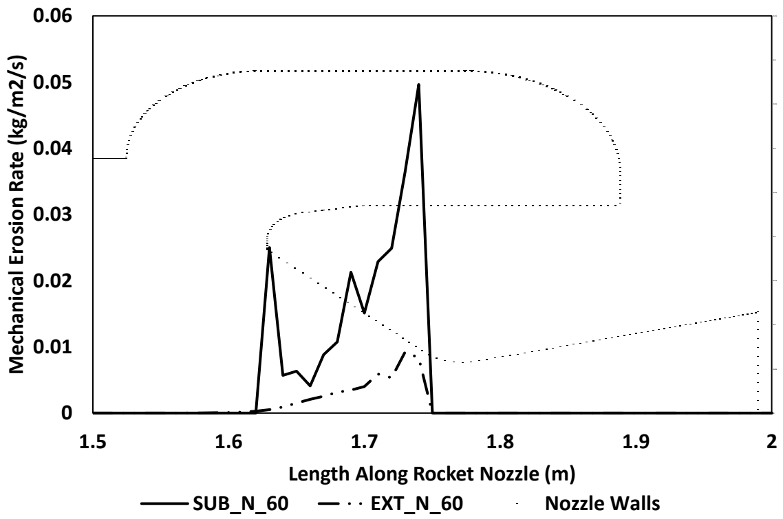
Figure 7-23: Erosion rate at different conditions for 60 μm droplet size
