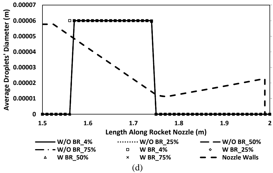
Figure 6-16: Average droplets' diameter over the nozzle length with and without applying the breakup model for different particle diameters (a) 300 \mu\text{m} , (b) 220 \mu\text{m} , (c) 140 \mu\text{m} , and (d) 60 \mu\text{m}
