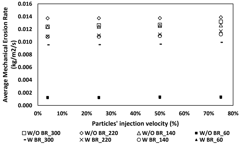
Figure 6-10: Average erosion rate for variable particles' injection velocity
