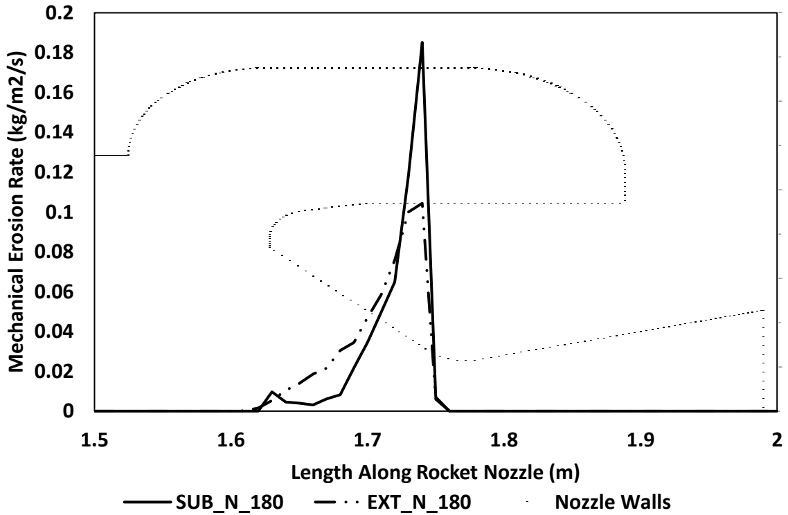
Figure 7-22: Erosion rate at different conditions for 180 μm droplet size
