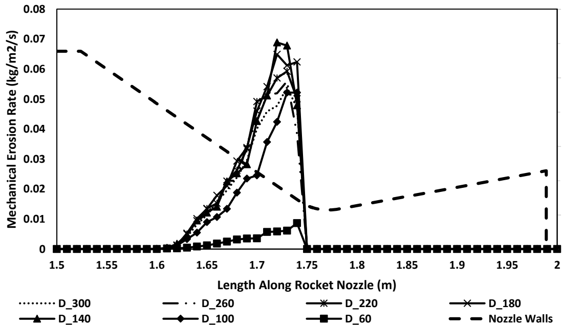
Figure 5-26: Mechanical erosion rate at different droplet's sizes after applying the break-up model
