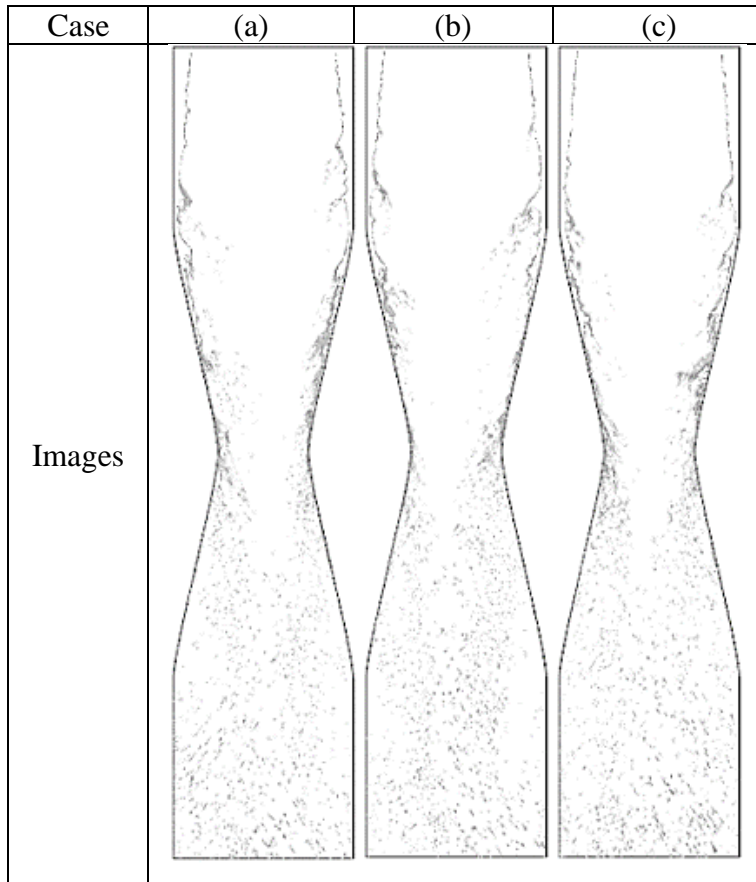
Figure 4-28: Numerical break-up pattern shapes at different air flow acceleration, a) 20 m/s 2 , b) 30 m/s 2 , c) 60 m/s 2
