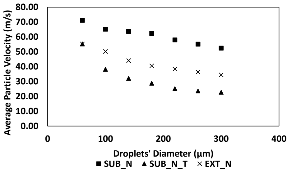
Figure 7-12: Average droplets' relative velocity at different droplet's sizes
