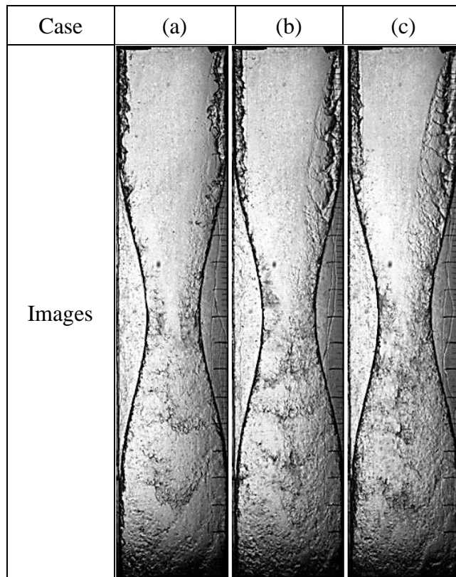
Figure 4-21: Experimental break-up pattern shapes at different water flow rates, (a) 1.9 \times 10^{-4} m 3 /s, (b) 2.5 \times 10^{-4} m 3 /s, and (c) 3.15 \times 10^{-4} m 3 /s.
