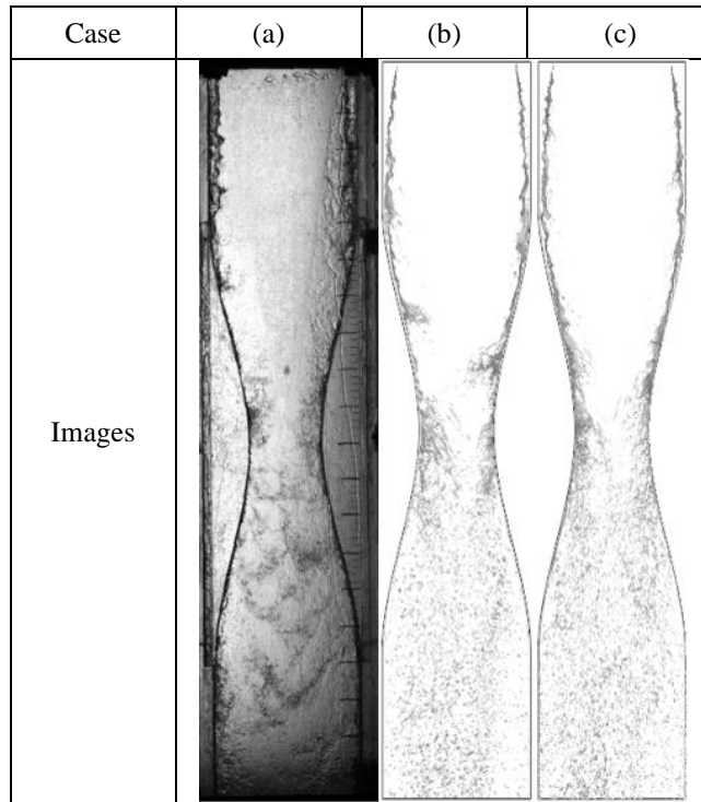
Figure 4-13: The breakup shape pattern at air velocity of 30 m/s, (a) Experiment with NWST, (b) Simulation with NWST and (c) Simulation with RWST
