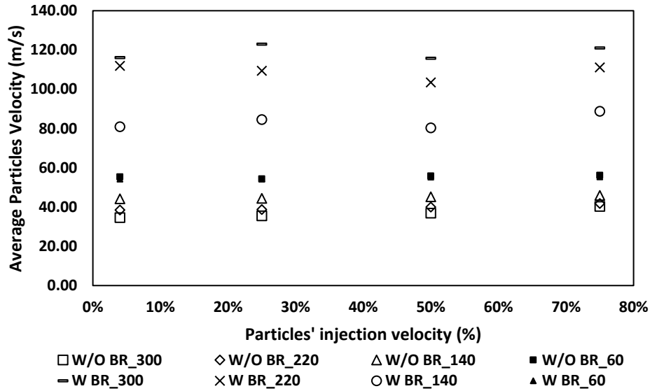
Figure 6-12: Average droplets' relative velocity for variable particles' injection velocity
