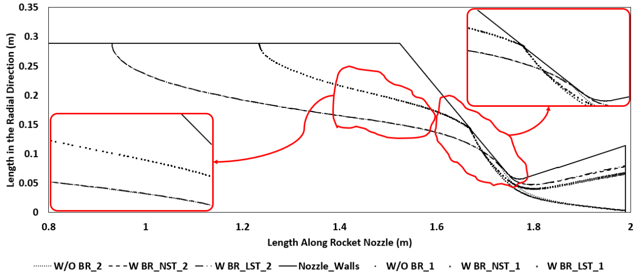
Figure 5-33: Two different parcels trajectories within the chamber for 300 \mu\text{m} droplet size
