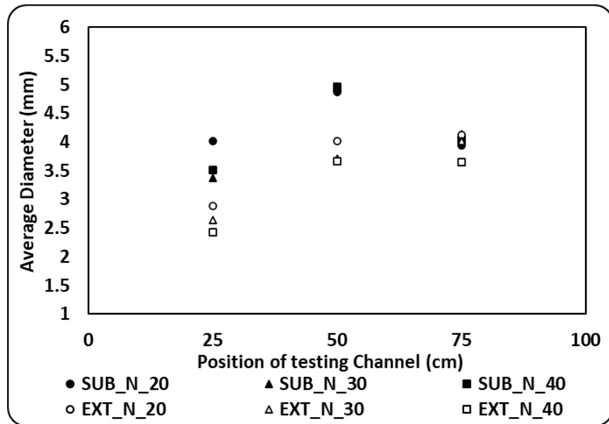
Figure 4-34: Experimental average droplet diameter at different sections of the testing channel and different air velocities
