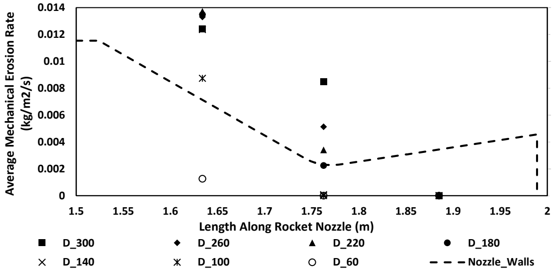
Figure 5-17: Average erosion rate over different sections of the nozzle for different droplets' sizes before applying the breakup model
