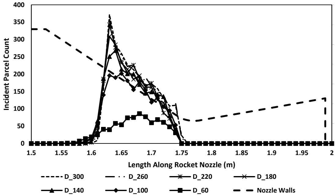
Figure 5-37: Incident mass flux at droplet's different sizes and lower surface tension
