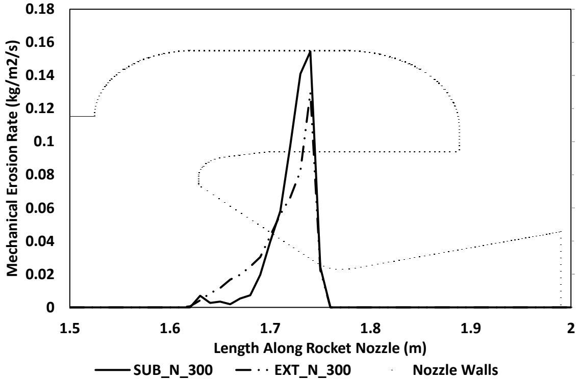
Figure 7-21: Erosion rate at different conditions for 300 μm droplet size
