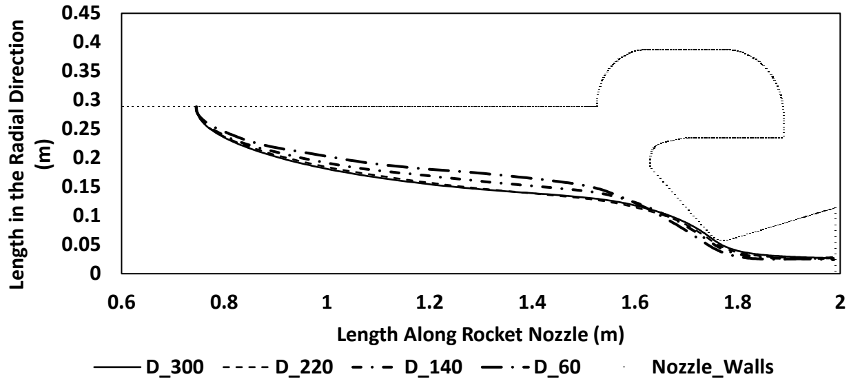
Figure 7-20: Parcel No. 3000 trajectories within the chamber at different droplet's sizes.
