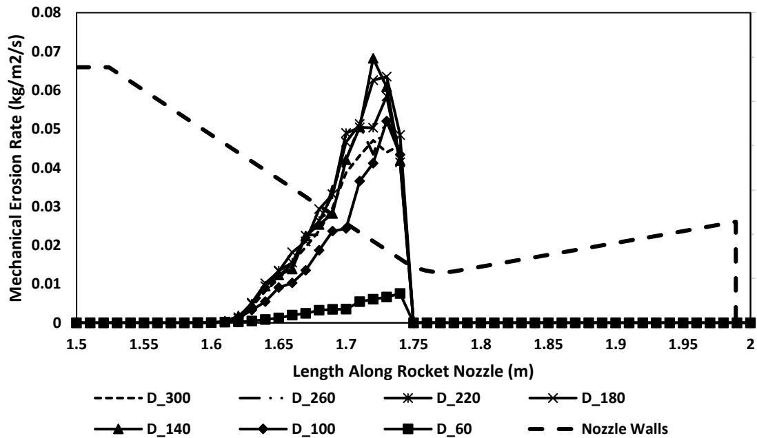
Figure 5-35: Mechanical erosion rate at droplet's different sizes and lower surface tension
