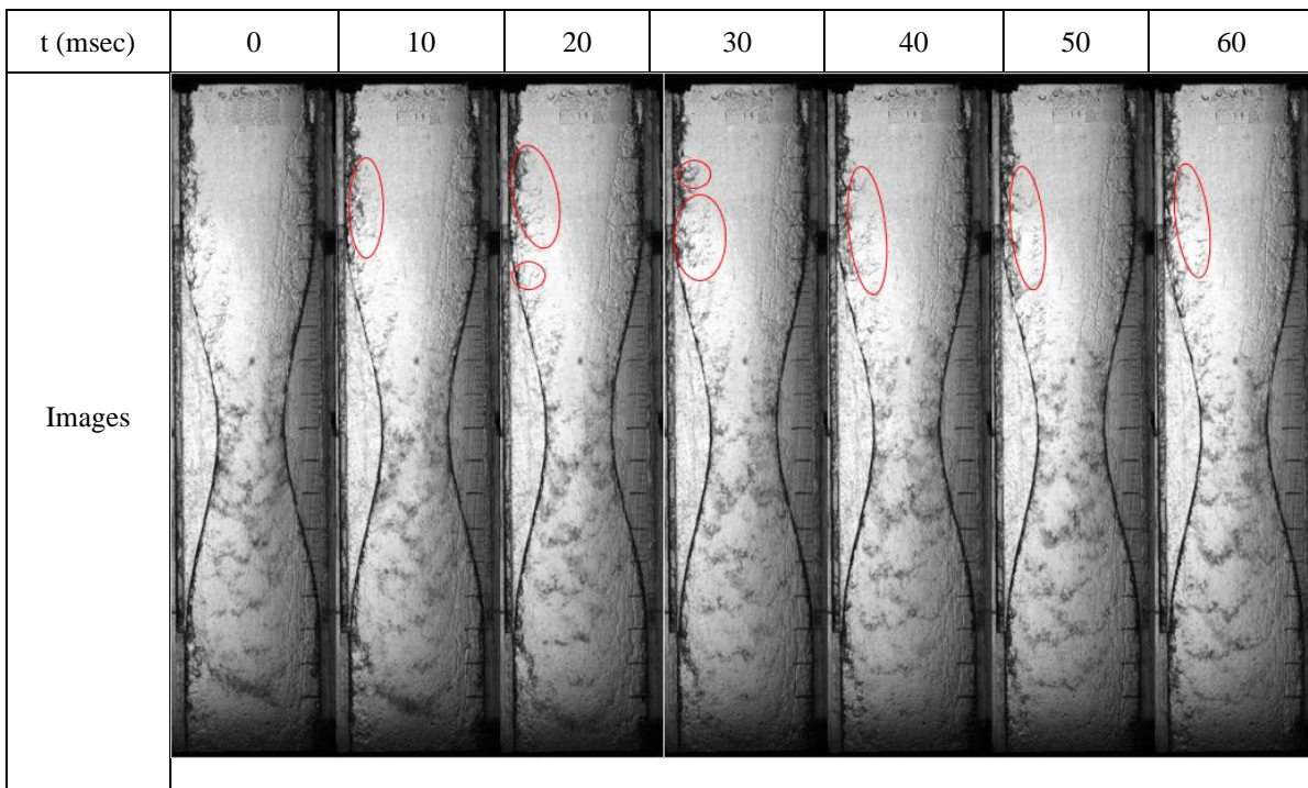
Figure 4-6: Experimental results for air velocity, 40 m/s and normal water (surface tension 0.072 N/m)
