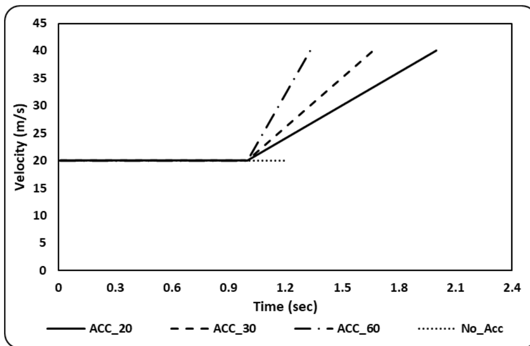
Figure 4-20: Air flow velocity profiles over the time
