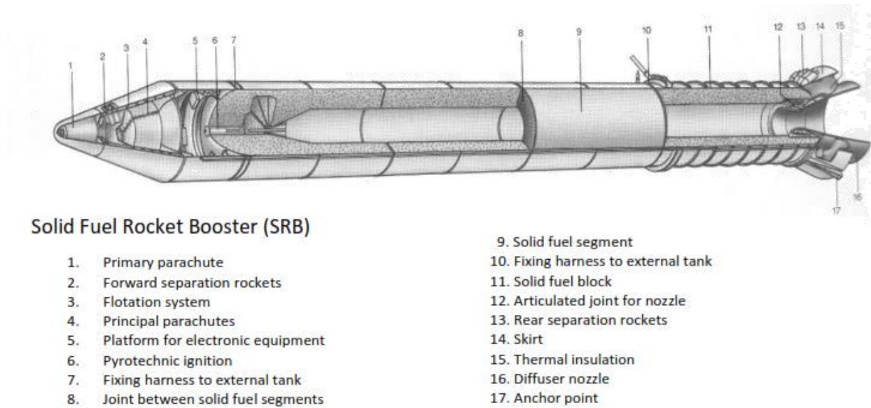
Figure 1-1: Solid rocket booster configuration, [2].
