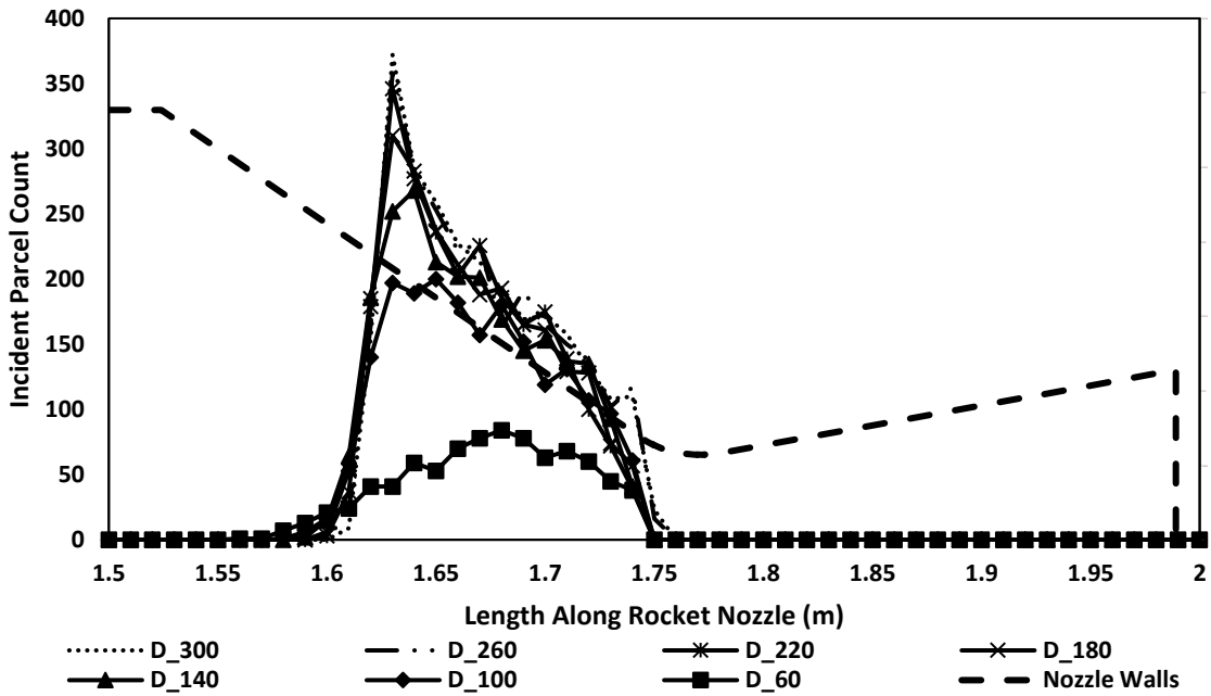
Figure 5-28: Incident parcels count at different droplet's sizes after applying the break-up model
