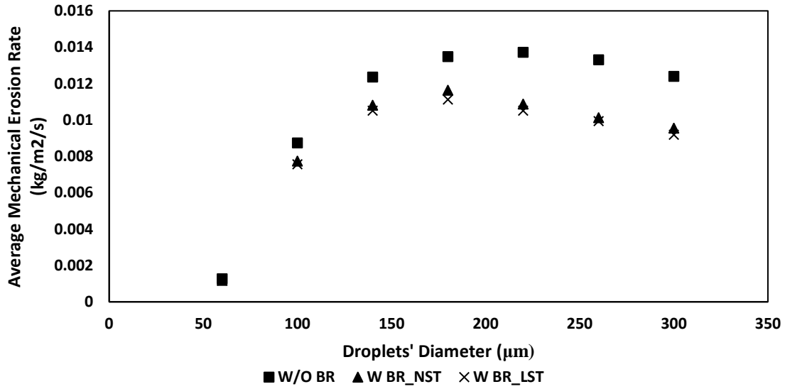
Figure 5-19: Average erosion rate on the nozzle's convergent section at different droplet's sizes
