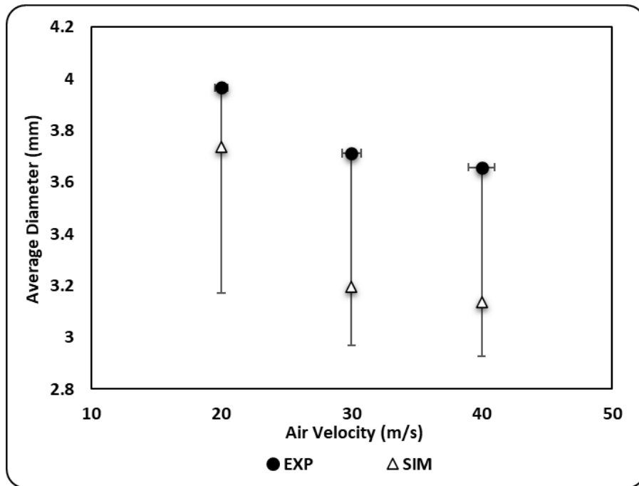
Figure 4-7: Experimental and numerical average droplet diameter throughout the entire testing channel at different air velocities
