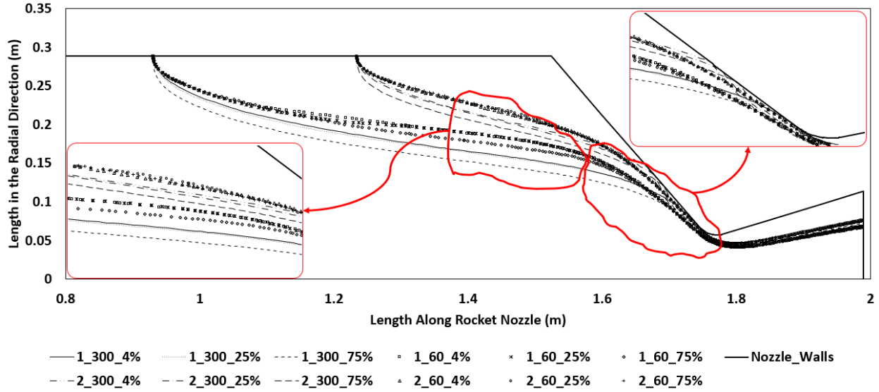
Figure 6-14: Two different parcels trajectories within the chamber for 300 \mu\text{m} , 60 \mu\text{m} droplet sizes and different injection velocities after applying the breakup model.
