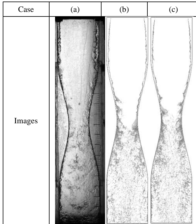
Figure 4-15: The breakup shape pattern at air velocity of 20 m/s, (a) Experiment with NWST, (b) Simulation with NWST and (c) Simulation with RWST
