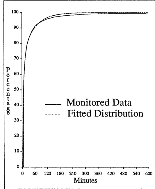
Figure 3. Distribution Of NA State Lengths Of All Stations
