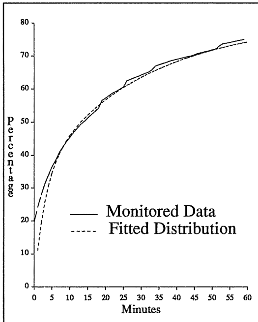
Figure 4. Distribution Of AV State Lengths Of All Stations
