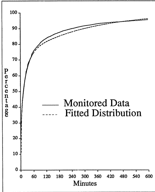
Figure 2. Distribution Of AV State Lengths Of All Stations
