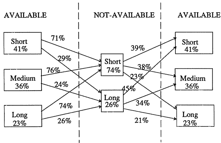
Figure 6. Conditional Probability of AV, NA State Changes
