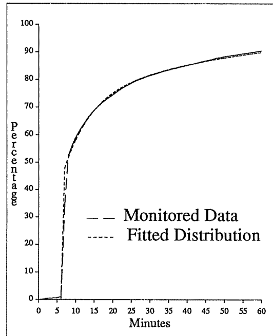
Figure 5. Distribution Of NA State Lengths Of All Stations
