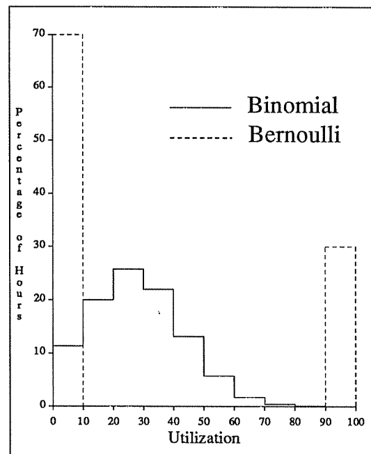
Figure 13. Bernoulli and Binomial Probability Density Functions
