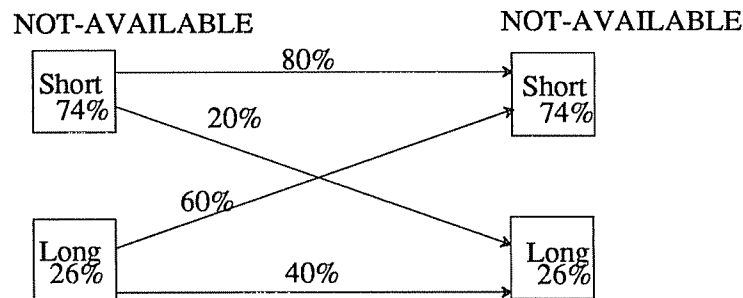
Figure 8. Conditional Probability of NA to NA State Changes
