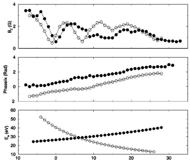
FIG. 10. Wave B_z amplitude, phase, and resonant electron energy ( E_e ) for the uniform magnetic field case at radial positions 0.93 cm ( \circ ) and 0.63 cm ( \bullet ). The 15-cm-long Nagoya type-III antenna is centered at z=0 .
