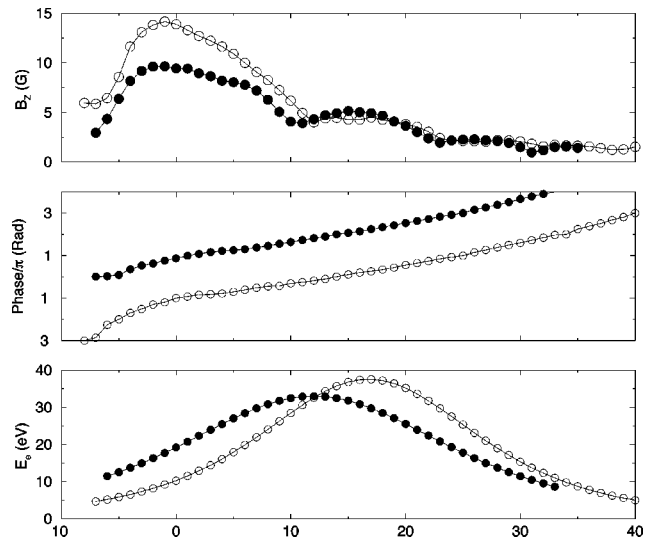
FIG. 9. Wave B_z amplitude, phase, and resonant electron energy ( E_e ) for the nonuniform magnetic field case at radial positions 0.93 cm ( \circ ) and 1.54 cm ( \bullet ). The 15-cm-long Nagoya type-III antenna is centered at z=0 .
