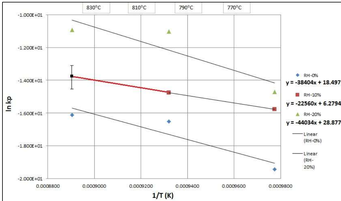
Figure 24. Partial pressures of \text{CeO}_2 coating at 0%, 10% and 20% of relative humidity.
