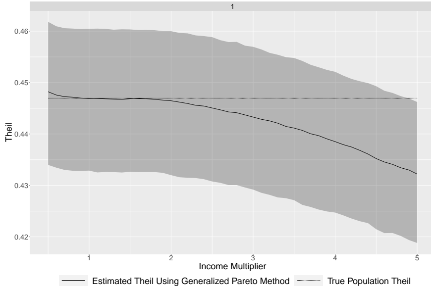
Figure 1.62: Performance of “Generalized Pareto” Method for Estimation of the Theil Index, with Increased Sample Size Theil estimated using the “Generalized Pareto” method on binned data created by random sampling from a population with a lognormal distribution of incomes with a location parameter of 3.5 and a scale parameter varying from 1-1.3. Samples then scaled from one half to five times their original value. Line is median estimate, bands represent the central 90% of estimates from random sampling from the distribution. Using 10% sample.
