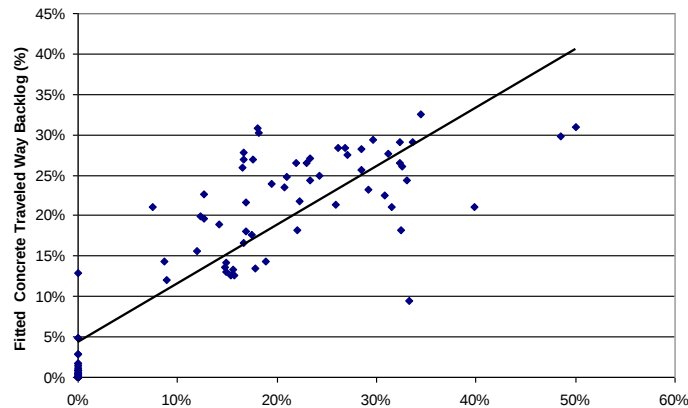
Figure 27. Observed versus fitted backlog for concrete traveled ways
