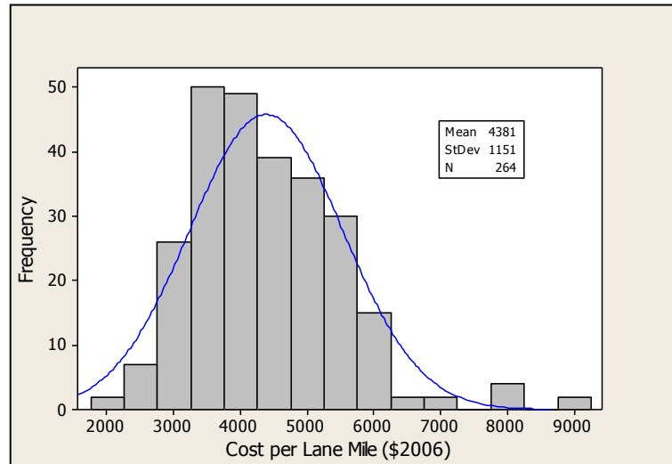
Figure 5. Histogram of non-normalized cost per lane mile.
