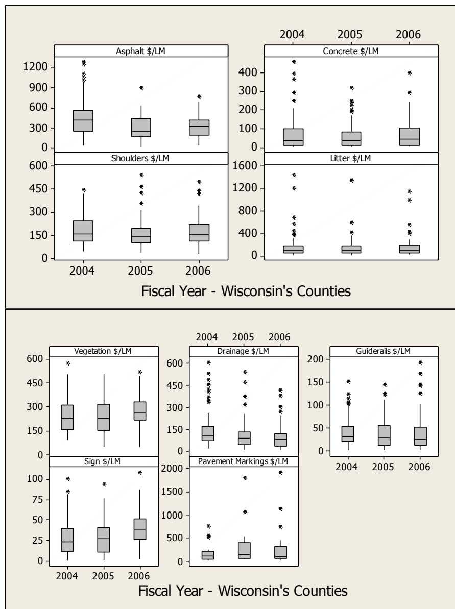
Figure 22. Annual trends for cost per lane mile for contracts with Wisconsin's counties.
