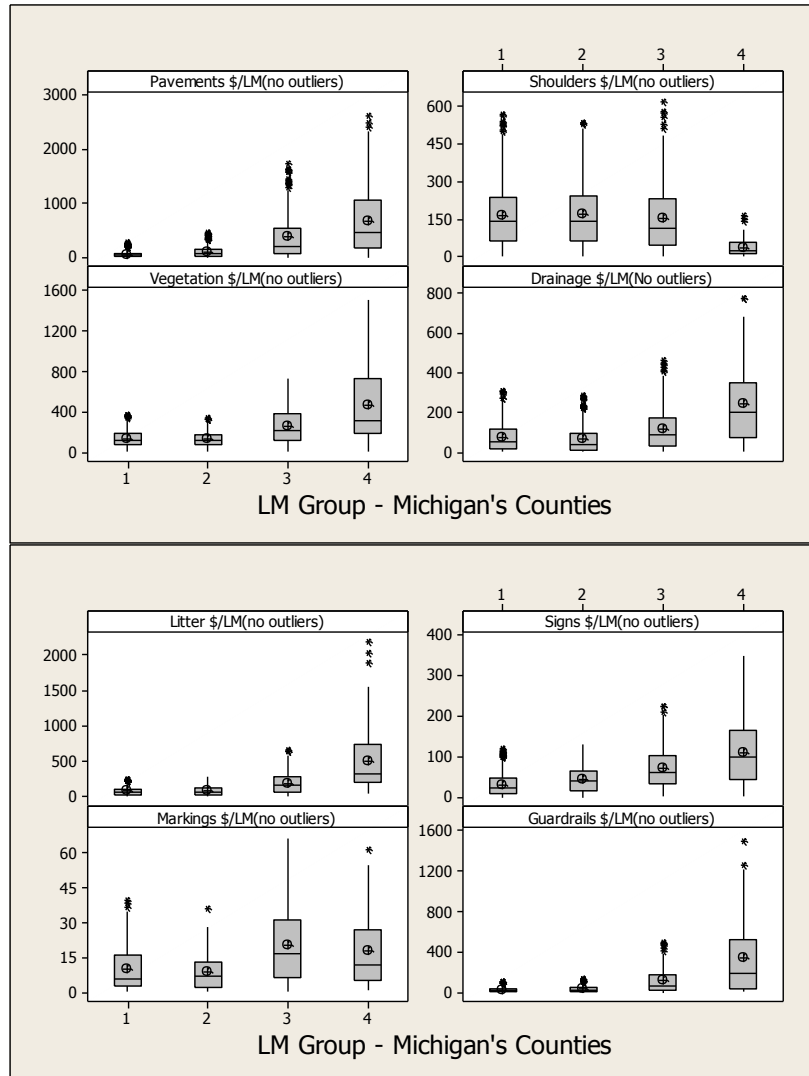
Figure 12. CPLM trends for LM groups – contracts with Michigan's counties
