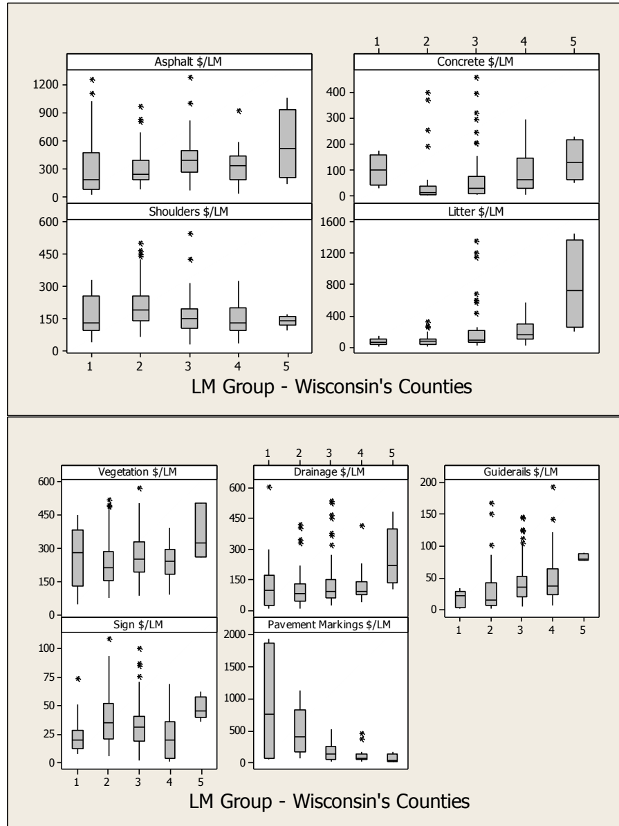
Figure 21. Wisconsin's cost per lane mile for maintenance categories and lane mile groups
