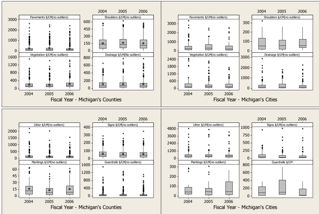
Figure 14. Annual CPLM trends - contracts with Michigan's counties
