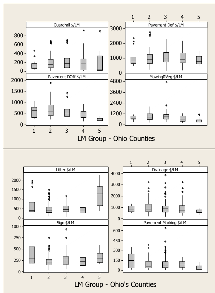
Figure 17. County lane mile (LM) groups - Ohio
