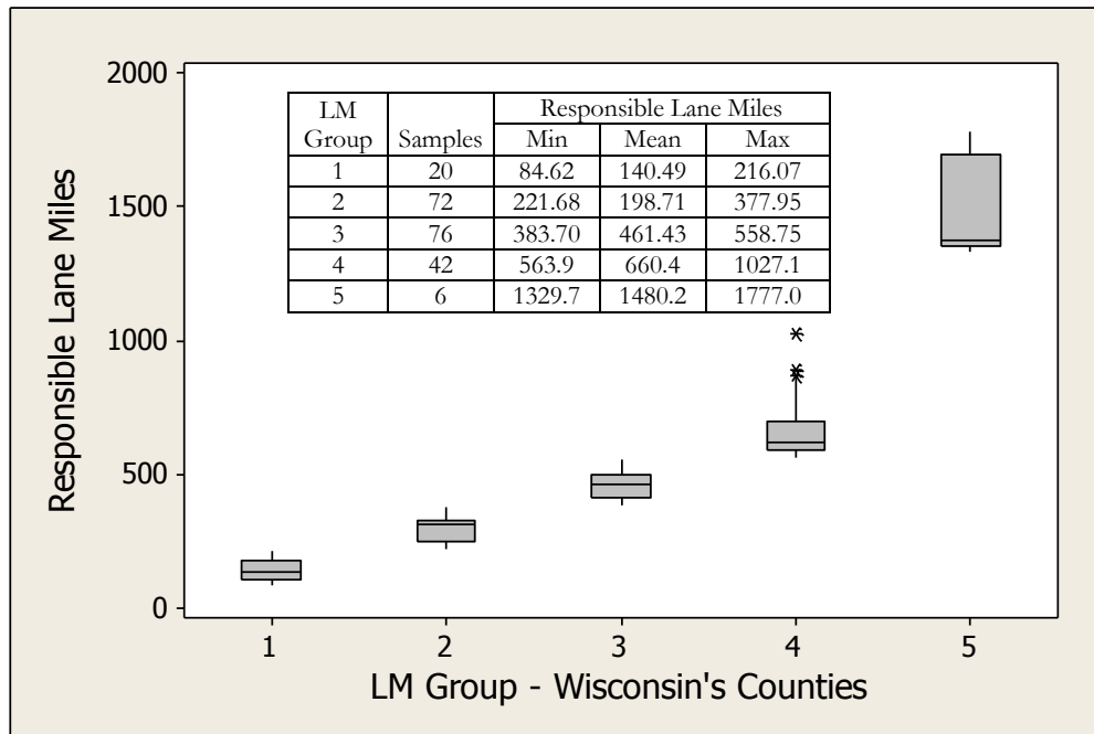
Figure 20. Lane mile (LM) groups – Wisconsin's counties
