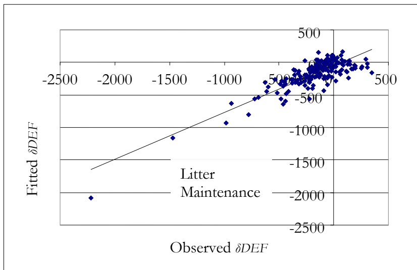
Figure 23. Observed deficiencies versus fitted models for Ohio
