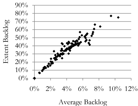
Figure 24. %Backlog for asphalt pavements in Wisconsin
