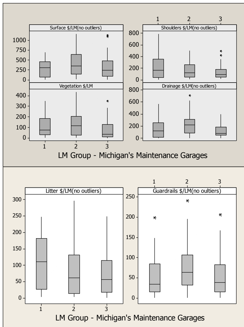
Figure 13. CPLM trends for LM groups – direct forces at Michigan's maintenance garages.
