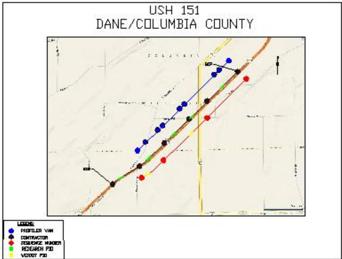
Figure 3.6 Test Sections for USH 151 Dane and Columbia Counties
