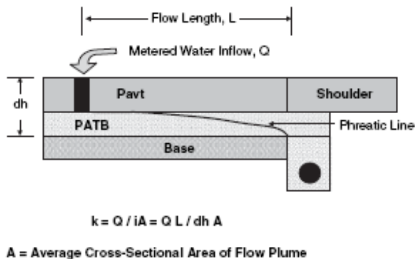
Figure 4.4 Measurement of In-Place Permeability
