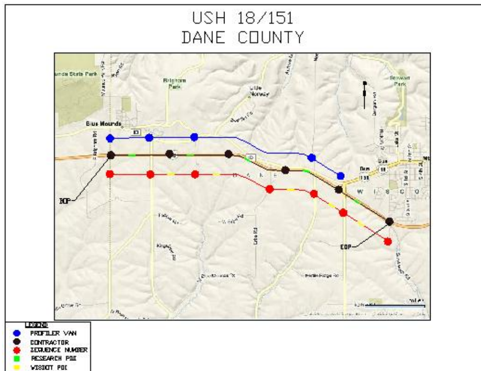
Figure 3.3 Test Sections for USH 18/151 in Dane County
