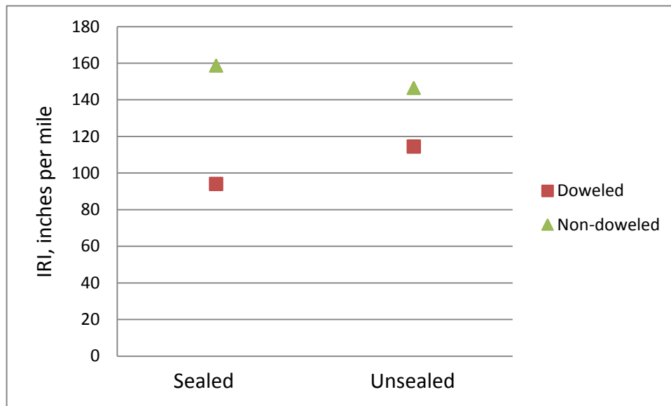
Figure 5.15 IRI for Sealed/Unsealed Doweled/Non-Doweled Joints on STH 29
