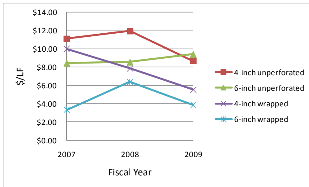
Figure 7.4 Unit Prices for Underdrain Pipe
