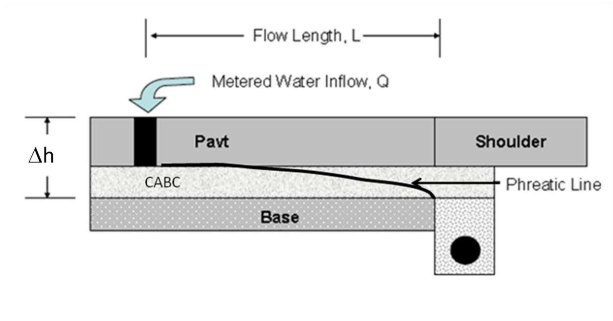
Figure 6.1 Flow Conditions During Permeability Testing
