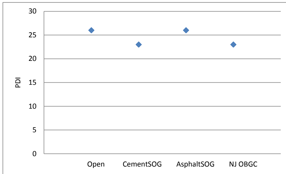
Figure 5.4 PDI variation for Unsealed Doweled Transverse Joints on USH 151
