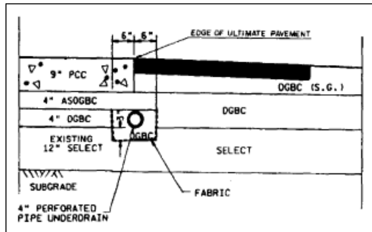
Figure B.3 USH 18/151 Sections 5, 6, and 12 with Asphalt-Stabilized OGBC
