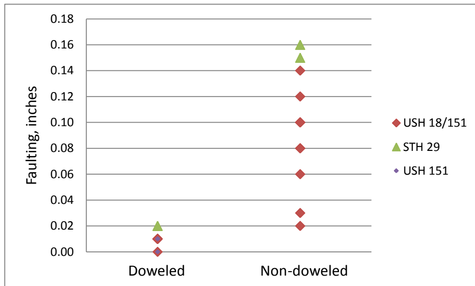
Figure 5.9 Faulting variation with Transverse Joint Dowel Treatment (all segments)
