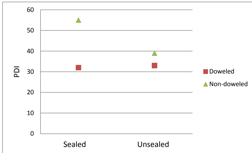
Figure 5.14 PDI for Sealed/Unsealed Doweled/Non-Doweled Joints on STH 29
