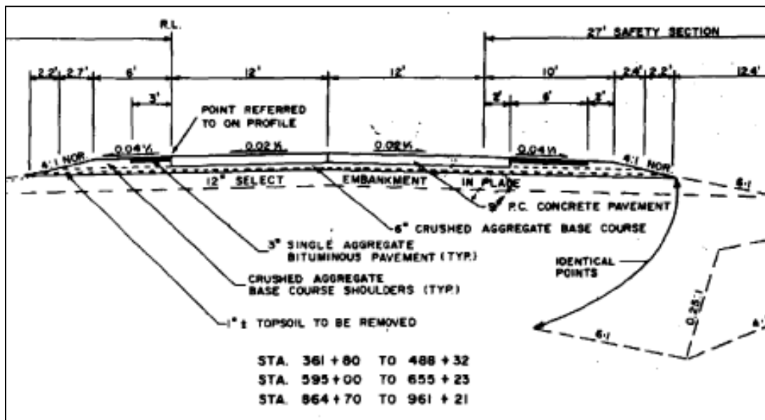
Figure B.5 USH 18/151 Sections 8, 9, 14 and 15 with Dense Graded Base Course
