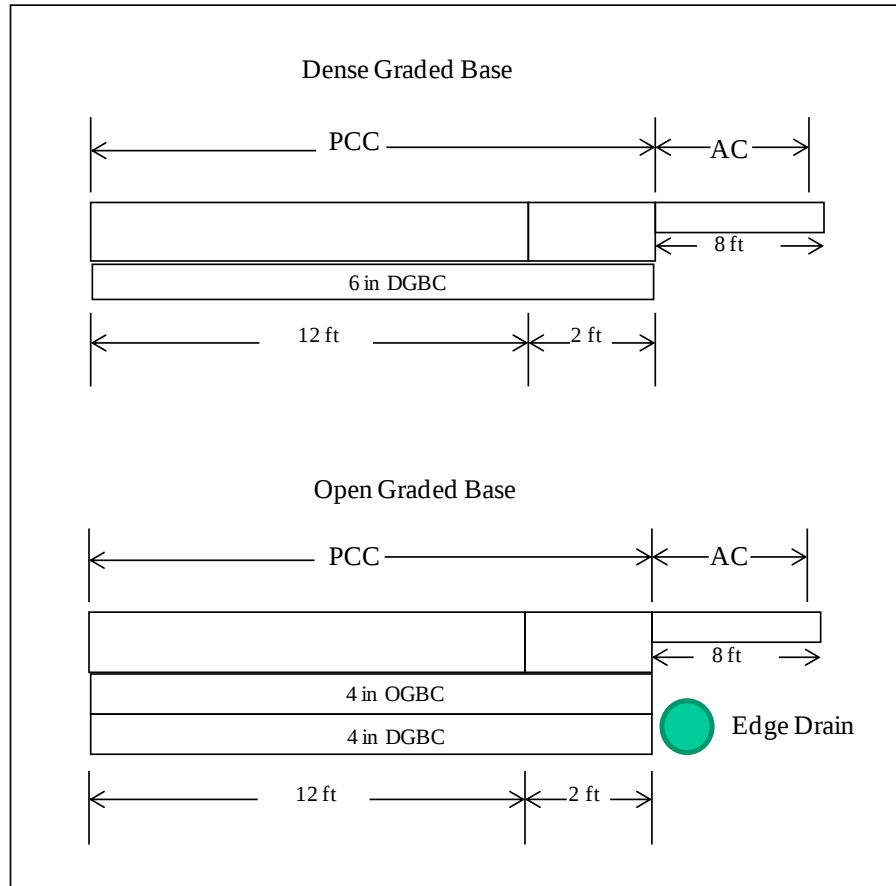
Figure 7.1 Pavement Cross Sections for LCCA
