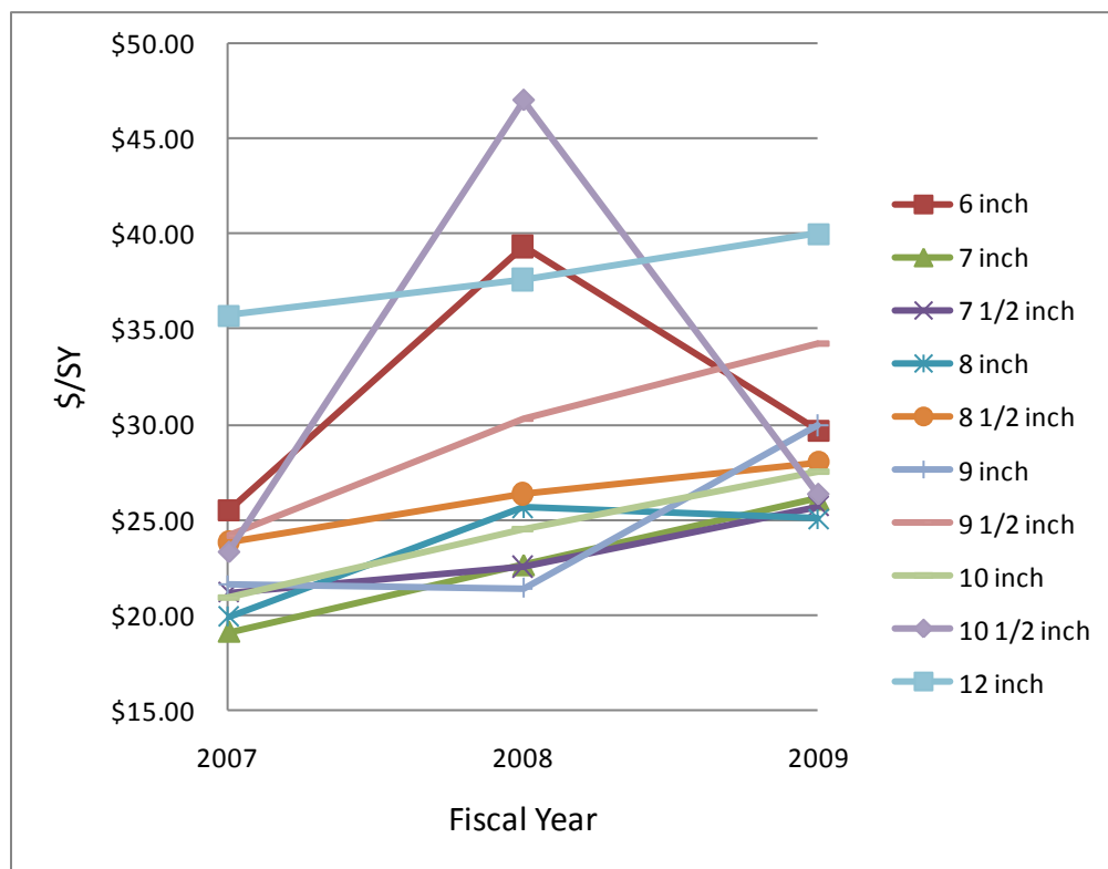
Figure 7.3 Unit Prices for Concrete Pavement Thickness
