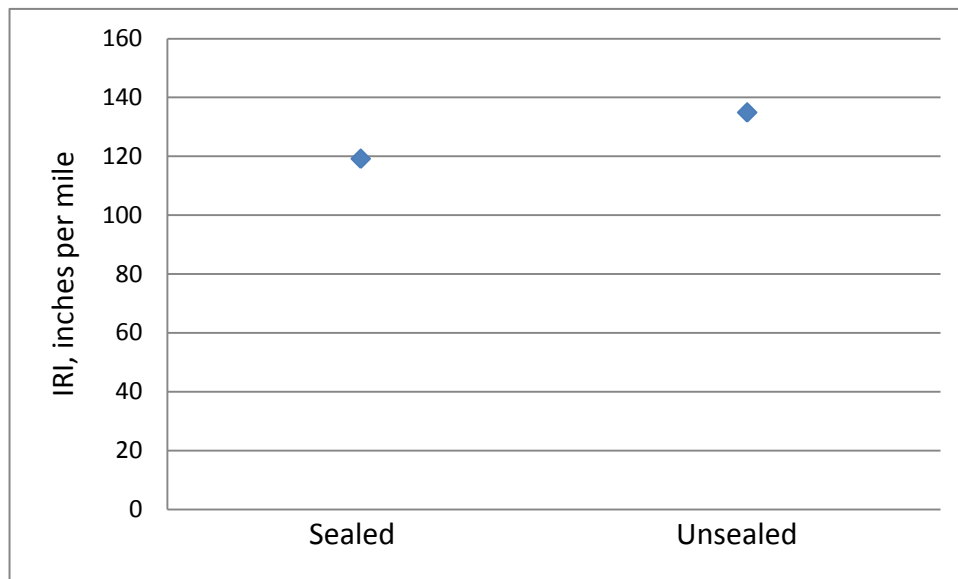
Figure 5.13 IRI for Sealed/Unsealed Doweled Joints on Dense Base (USH 18/151)
