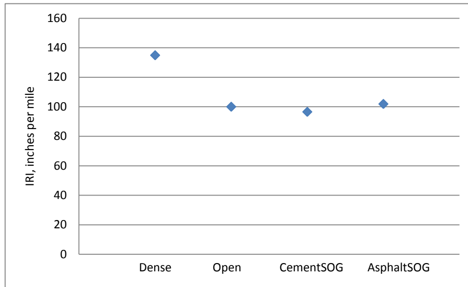
Figure 5.3 IRI variation for Unsealed Doweled Transverse Joints on USH 18/151
