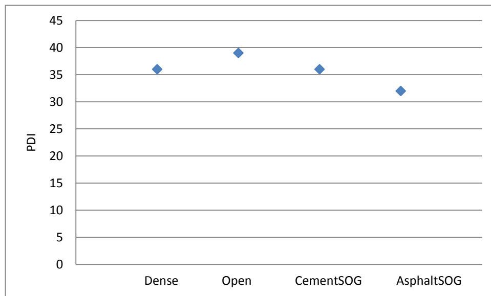
Figure 5.2 PDI variation for Unsealed Doweled Transverse Joints on USH 18/151
