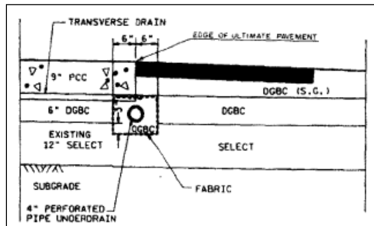
Figure B.4 USH 18/151 Sections 7 and 10 with TIC Drain
