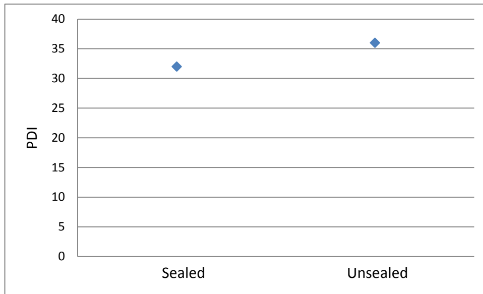
Figure 5.12 PDI for Sealed/Unsealed Doweled Joints on Dense Base (USH 18/151)
