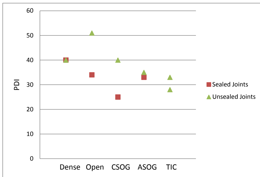
Figure 5.6 PDI variation for Base Type on Non-doweled Sections on USH 18/151
