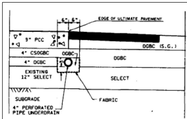
Figure B.2 USH 18/151 Sections 3, 4, and 11 with Cement-Stabilized OGBC
