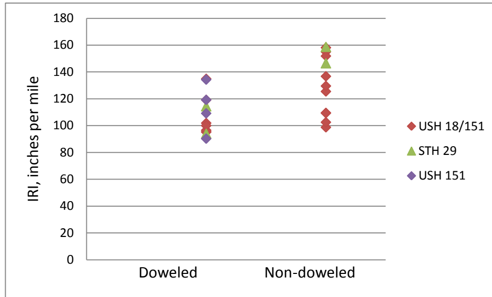
Figure 5.10 IRI variation with Transverse Joint Dowel Treatment (all segments)
