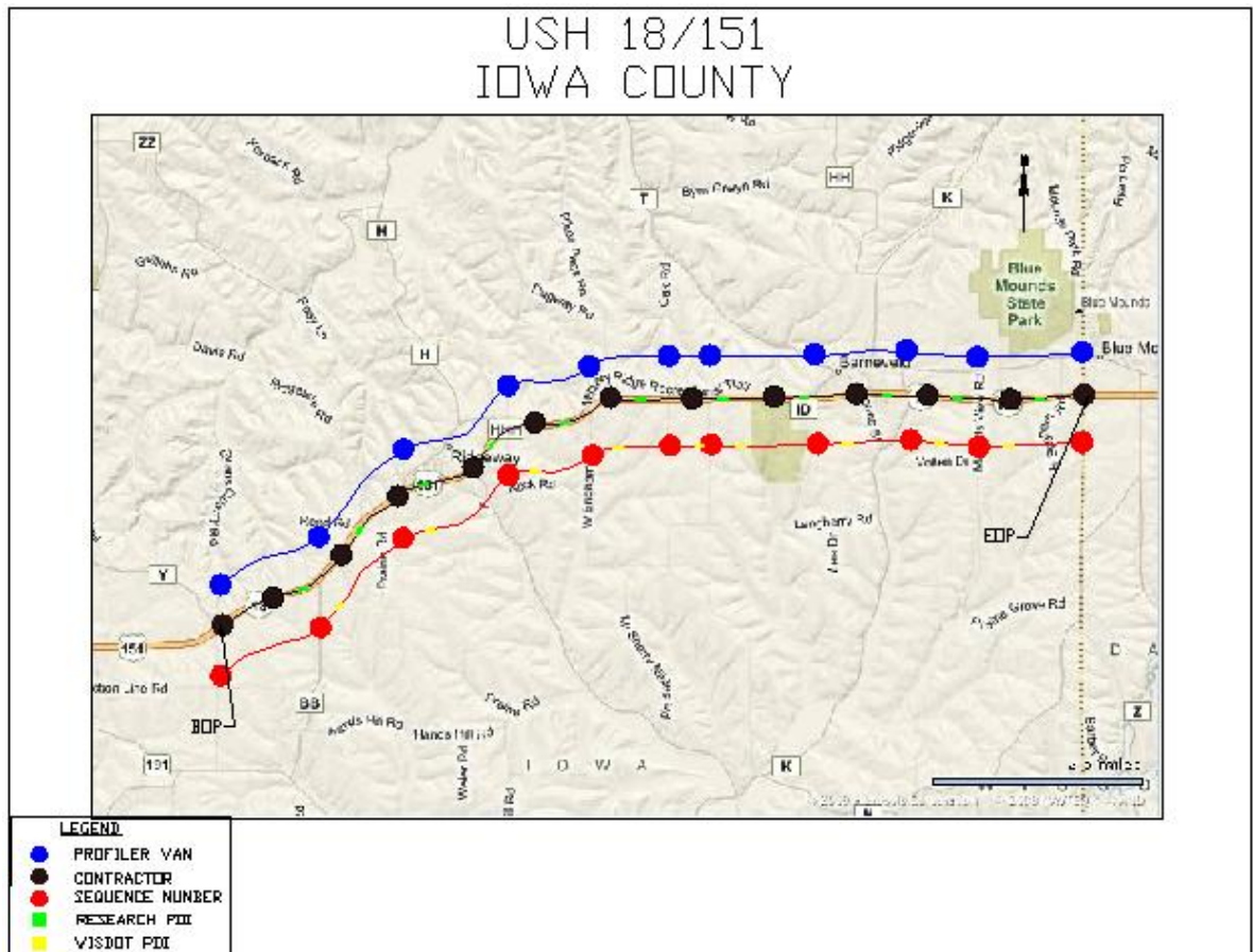
Figure 3.2 Test Sections for USH 18/151 in Iowa County
