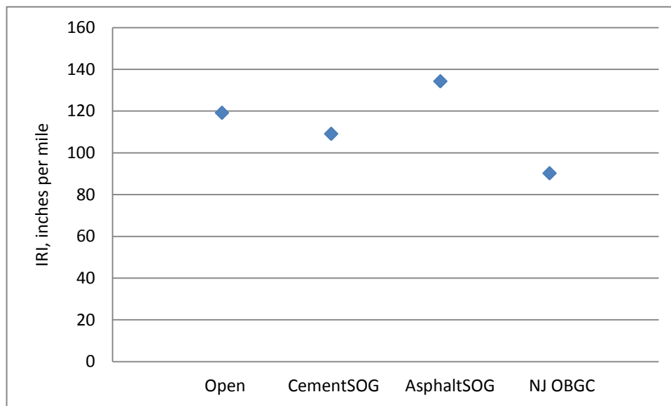
Figure 5.5 IRI variation for Unsealed Doweled Transverse Joints on USH 151
