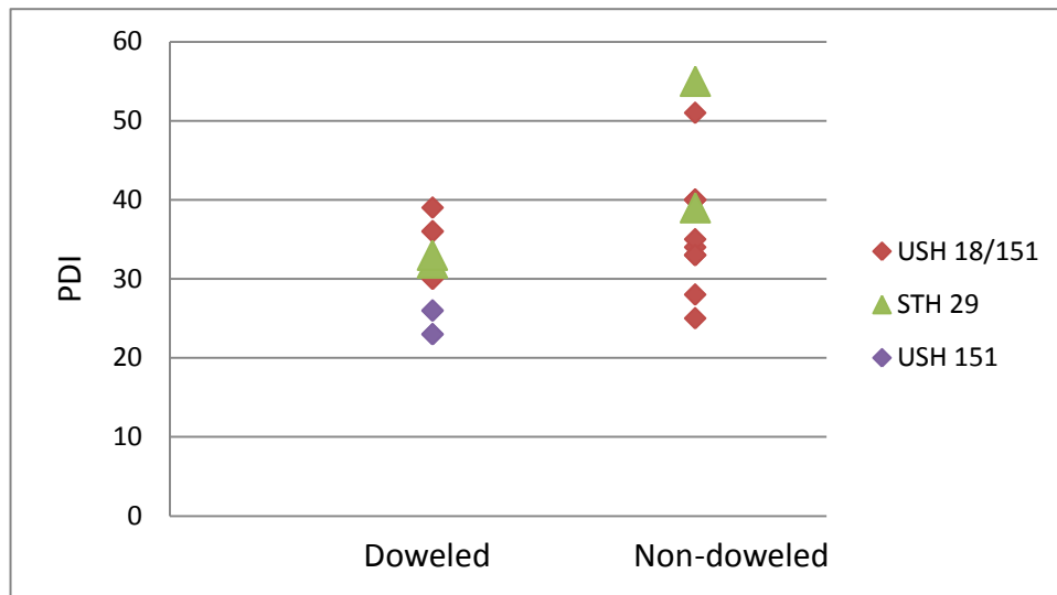
Figure 5.8 PDI variation with Transverse Joint Dowel Treatment (all segments)
