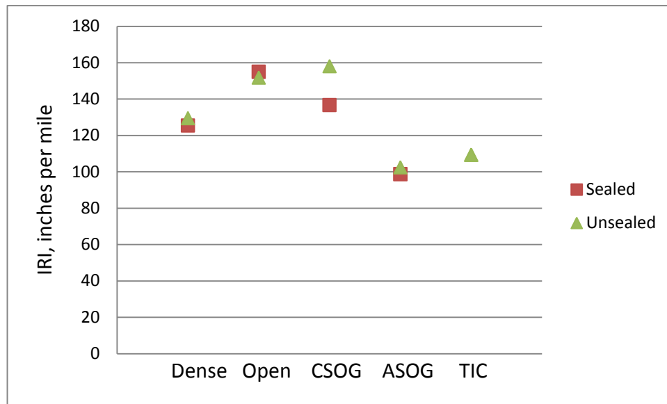
Figure 5.7 IRI variation for effect of Base Type on Non-doweled Sections on USH 18/151
