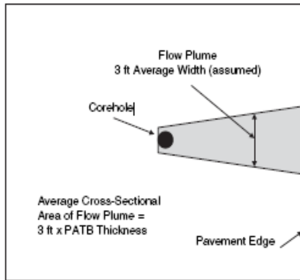
Figure 4.5 Illustration of plume of water from core hole to pavement edge
