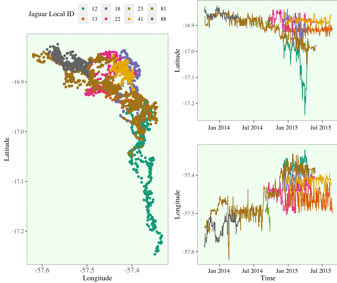
Figure 6.1: Visualization of Jaguar Movement in the Taiamã Ecological Station. (Left) The spatial distribution of GPS recordings is plotted and colored by Jaguar ID. (Right) The temporal change in each Jaguar's latitudinal and longitudinal position [73, 74]. A terrain map of this region is provided in the published work [40]
