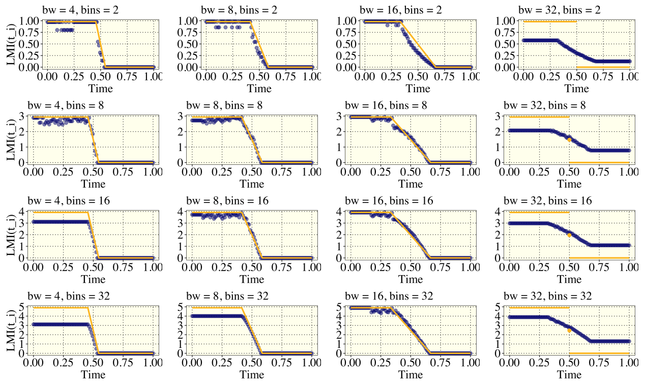
Figure 7.1: Implementation of Simulation 1 from Section 5.2.2 using Equal Width Binning . As is depicted the decline in LMI matches the timing of the decline from the analytic evaluation.
