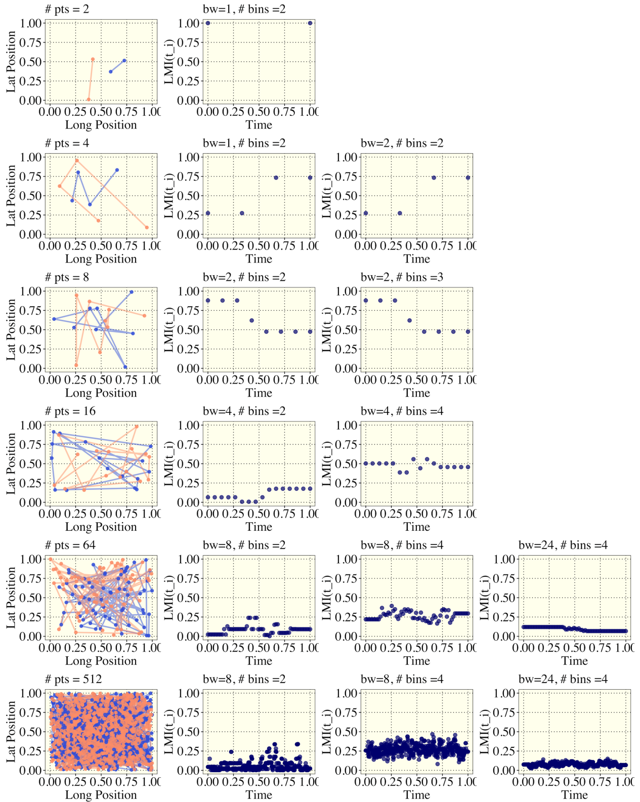
Figure 5.18: LMI Sensitivity to low temporal resolution for Brownian particle movement. The first column is the animal movement path in \mathbb{R}^2 , and the remaining columns are the computed LMI functions for an array of bandwidths and bins.
