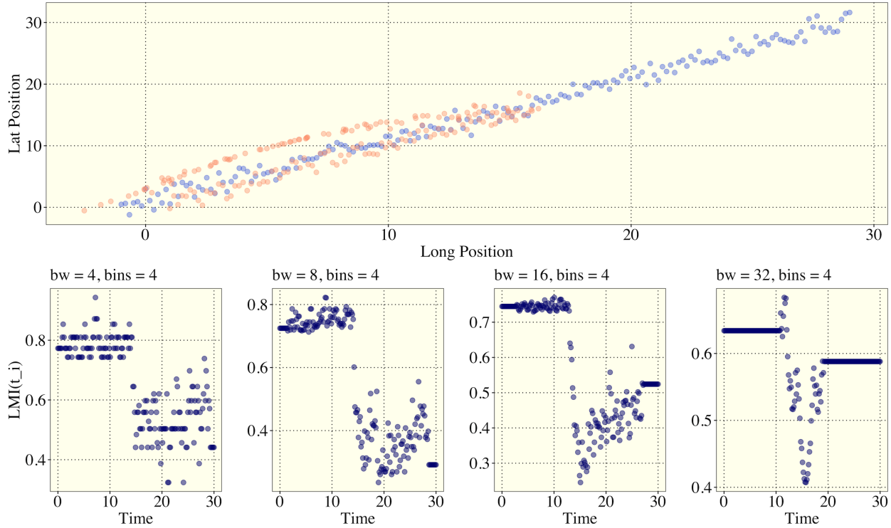
Figure 5.12: (Upper) Simulation 2 movement with \epsilon_{t_i} = 0 . (Lower) LMI functions with various bandwidths (bw) and number of bins (bins) set to 4 for the discretized estimation of the pmf for each time window surrounding t_i .
