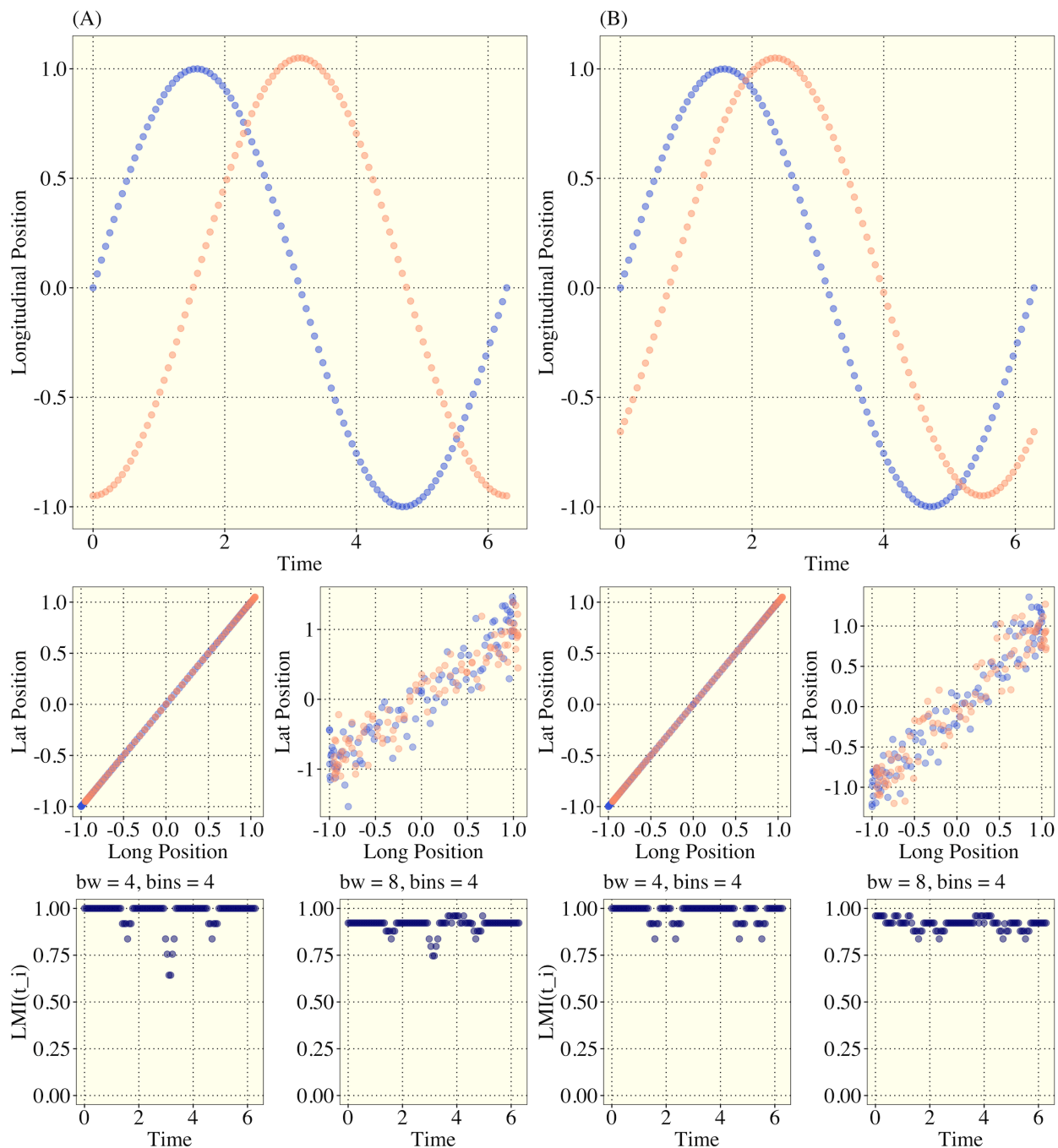
Figure 5.16: Simulation 4 Linear Tracing Movement Paths. (A) [Upper] plot show the induced temporal phase shift of \varphi = \pi/2 for the Longitudinal component. [Center] The generated movement paths in \mathbb{R}^2 with \epsilon = 0, 0.2 . [Lower] The LMI functions for each of the respective errors. (B) Same as detailed for (A) but with \varphi = \pi/4 .
