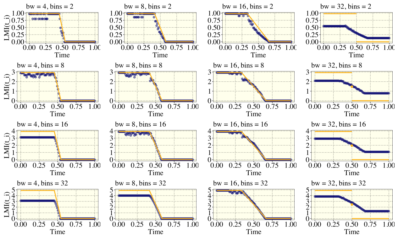
Figure 7.2: Implementation of Simulation 1 from Section 5.2.2 using Global Equal Width Binning . As is depicted the decline in LMI matches the timing of the decline from the analytic evaluation.
