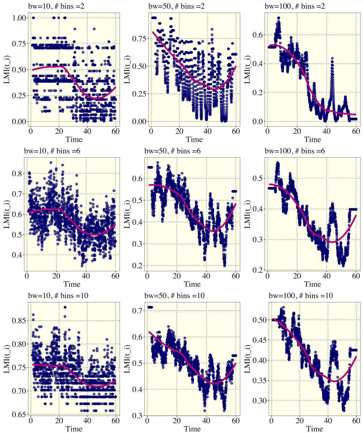
Figure 5.21: LMI function computed for an array of bandwidths and number of bins. The overlaid magenta line in each plot is a LOESS trend line.
