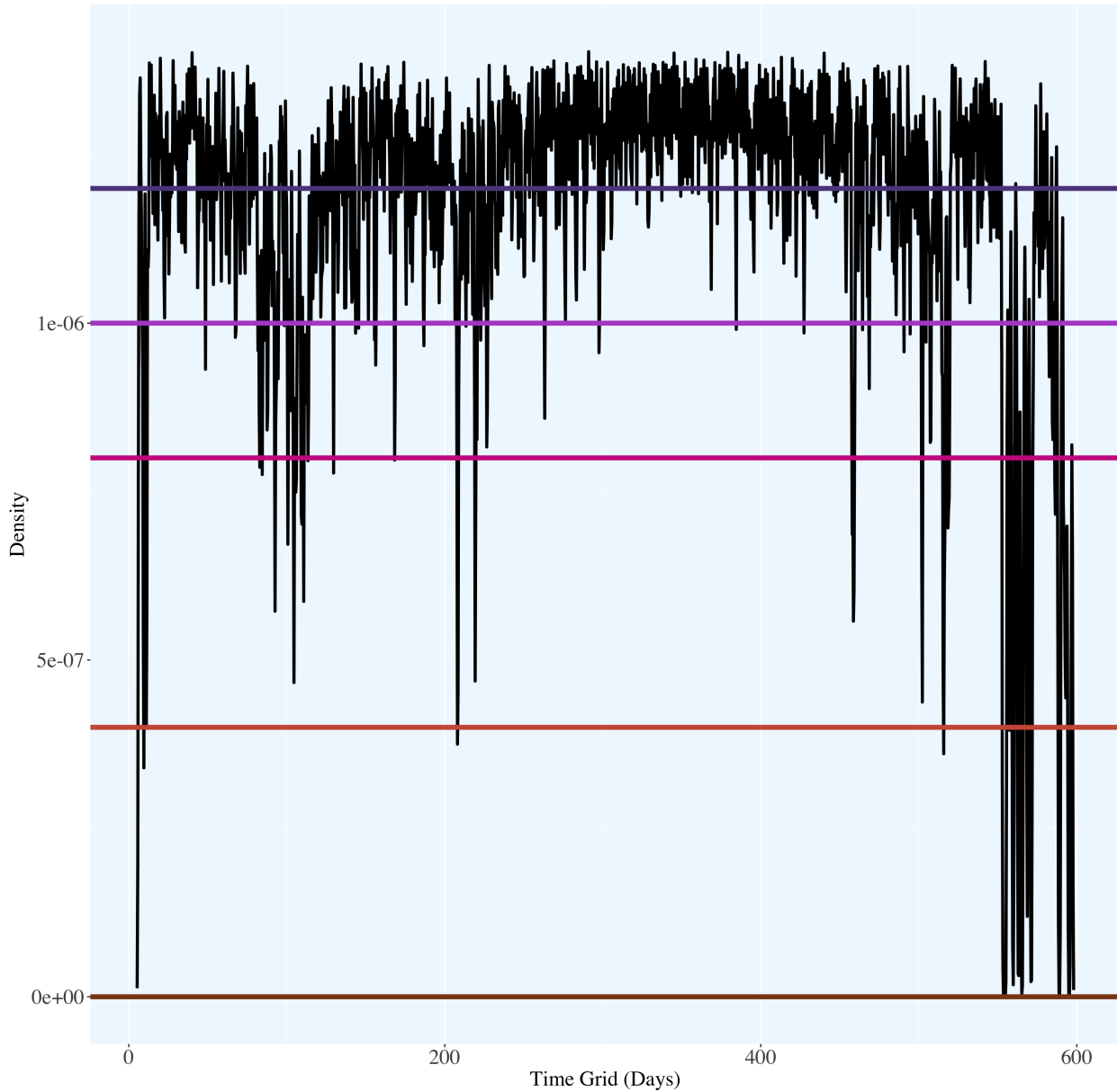
Time Grid Density: Jaguar 81 (M)
