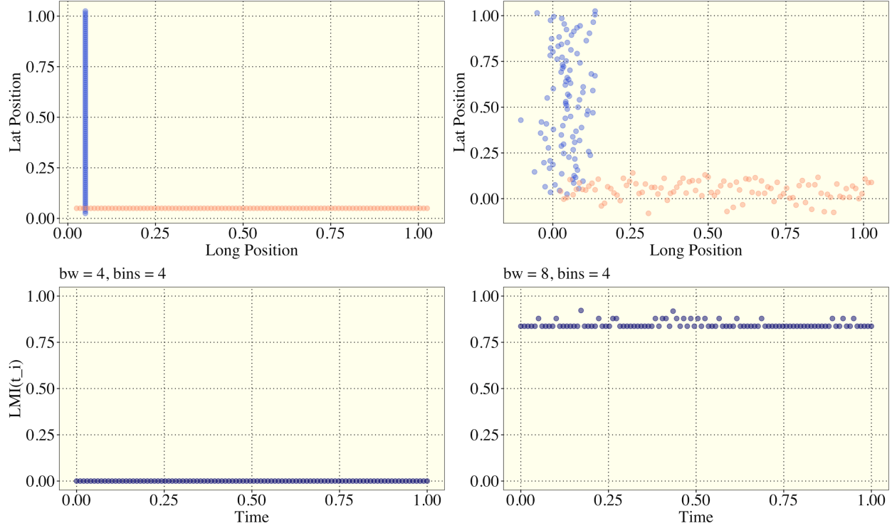
Figure 5.13: (Upper) Simulation 3 movement paths for strict cardinal movement generated with \epsilon_{t_i} = 0 and 0.05 respectively. (Lower) The LMI Functions for the corresponding movement paths from the upper plots.
