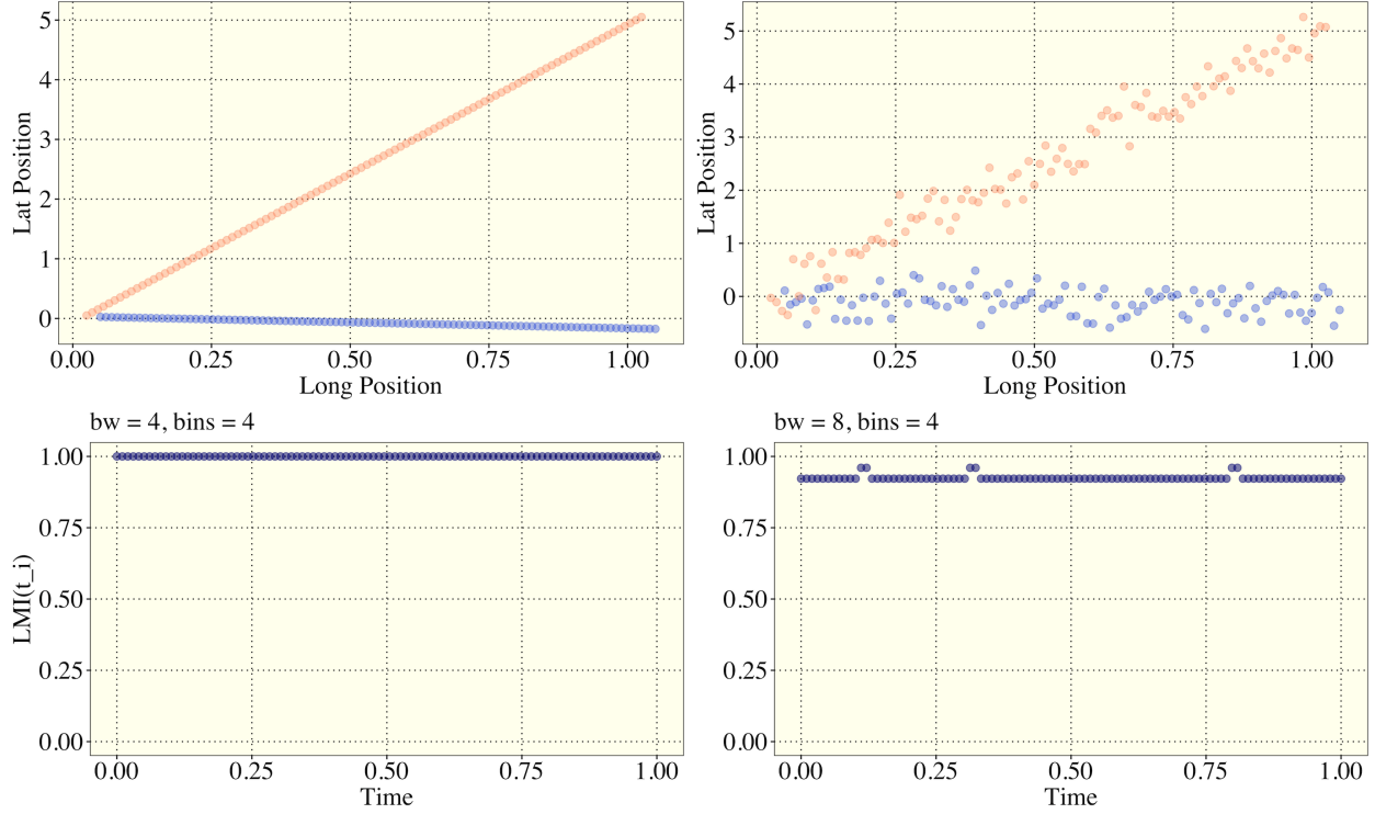
Figure 5.14: (Upper) Simulation 3 movement paths generated with \epsilon_{t_i} = 0 and 0.05 respectively with rotation off the cardinal axes. (Lower) The LMI Functions for the corresponding movement paths from the upper plots.
