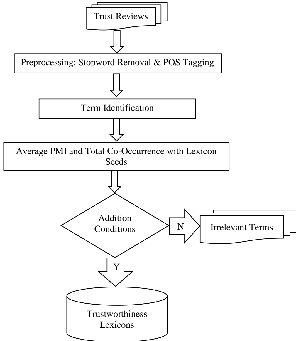
Figure 4.2- The Proposed Method for Extracting and Classifying Trustworthiness Characteristics from Trust Reviews
