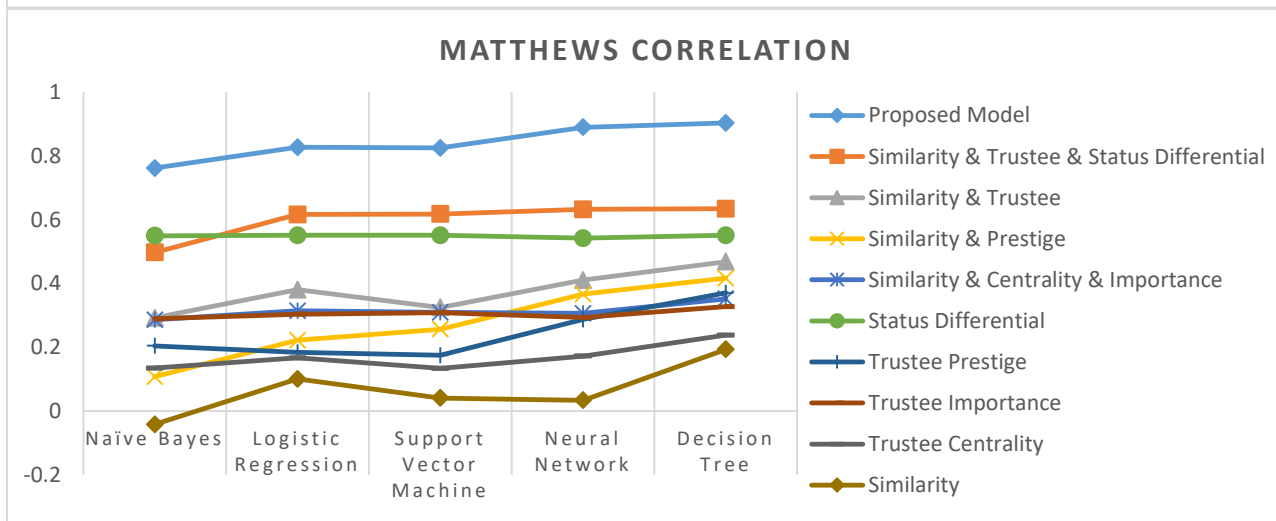
Figure 3.2- Results: Performance of the Proposed Model and Baselines
