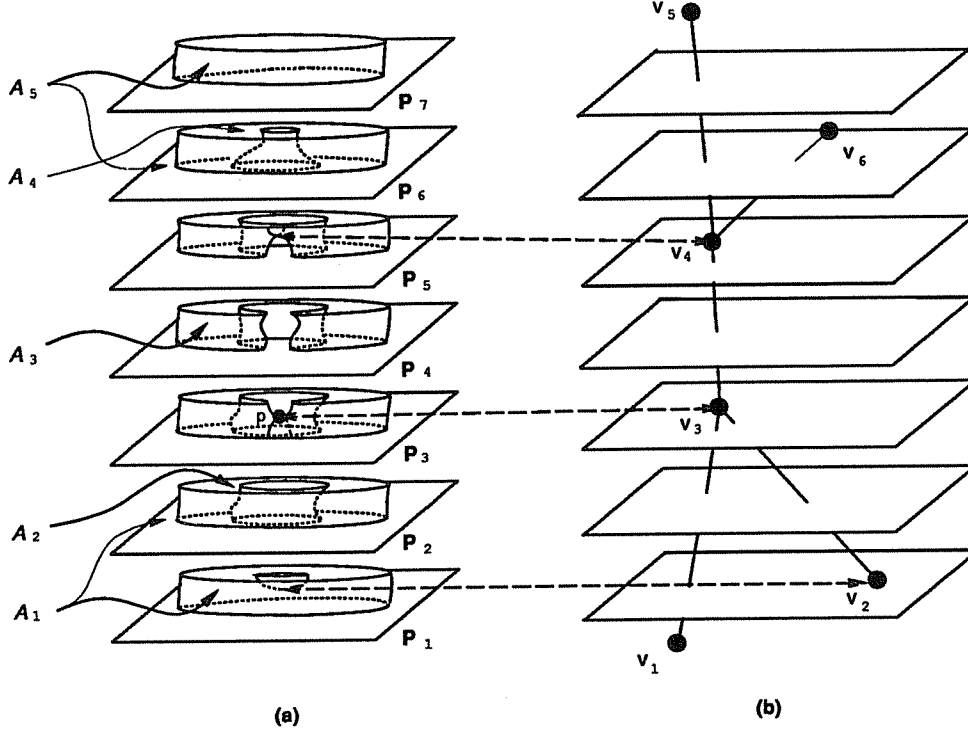
Figure 5: (a) Topological changes in S \cap P_d for a generic cylindrical-shaped surface S with a concavity. The surface can be partitioned into a number of cylindrical-shaped slices of various widths each corresponding to the families \mathcal{A}_1, \dots, \mathcal{A}_5 . (b) The surface graph of S . Nodes in the graph are associated with points of tangency of S with a plane from the family P_{d \in \mathbb{R}} . For example, v_3 corresponds to the (hyperbolic) point p contained in the boundaries of \mathcal{A}_1, \mathcal{A}_2 , and \mathcal{A}_3 . v_2 corresponds to the (elliptic and concave) point where a plane from the family P_{d \in \mathbb{R}} between P_1 and P_2 is tangent to the surface and bounds \mathcal{A}_2 from below. The observer has no information about the structure of the surface graph (i.e., its vertices and their connectivity) when the exploration process is initiated.
