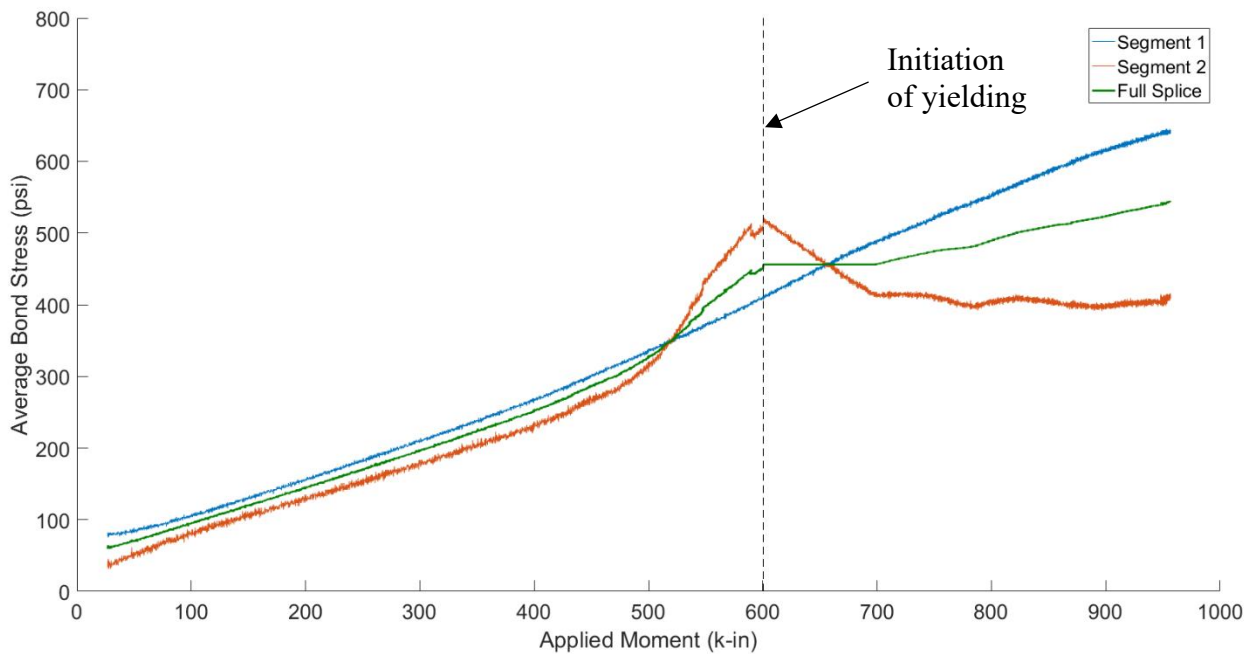
Figure 7.34 – Specimen 2 average bond stress versus applied moment for spliced Stage 1 bottom transverse bars.
