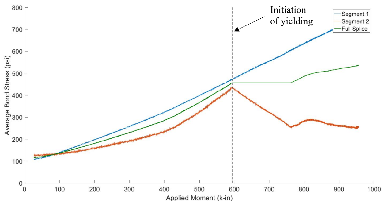
Figure 7.35 – Specimen 2 average bond stress versus applied moment for spliced Stage 2 bottom transverse bars.
