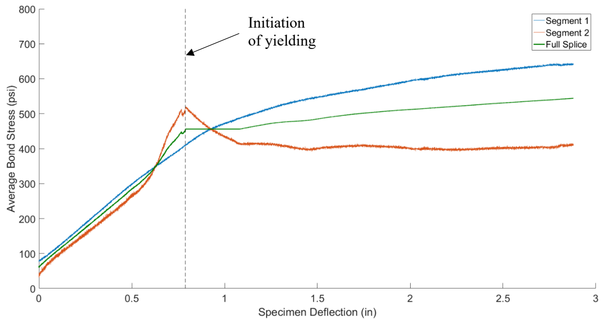
Figure 7.32 – Specimen 2 average bond stress versus specimen deflection for spliced Stage 1 bottom transverse bars.
