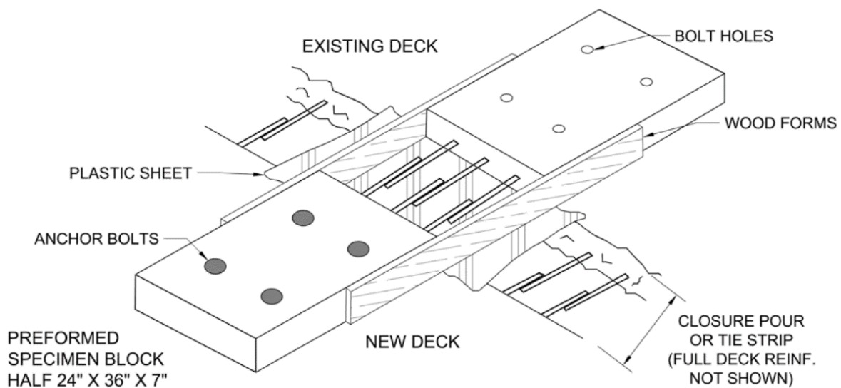
Figure 2.3 – Closure strip field specimens tested in Deaver (1982). (Adapted from Deaver 1982)
