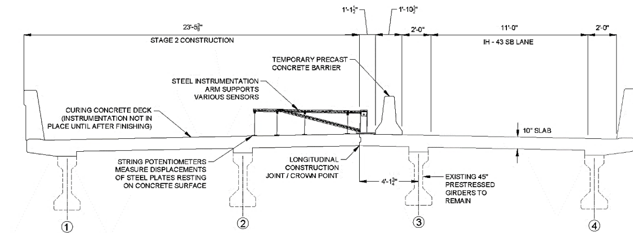
Figure 5.12 - B-64-123 Cross section of bridge B-64-123 during stage 2 construction (looking
