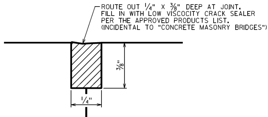
Figure 4.5- WisDOT longitudinal construction joint standard detail (WisDOT 2017)
