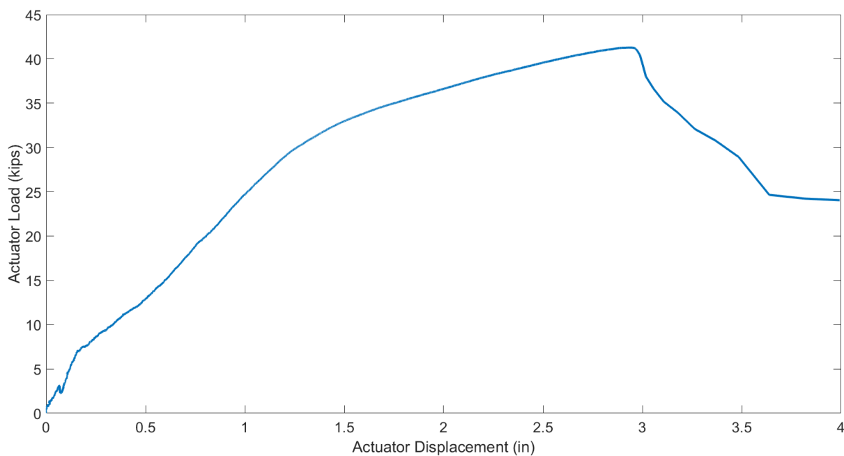
Figure 7.18 - Actuator load versus mid-span displacement response for the ultimate test of Specimen 1.
