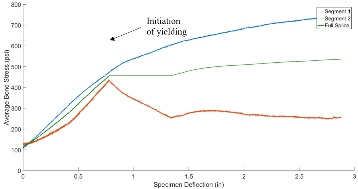
Figure 7.33 – Specimen 2 average bond stress versus specimen deflection for spliced Stage 2 bottom transverse bars.
