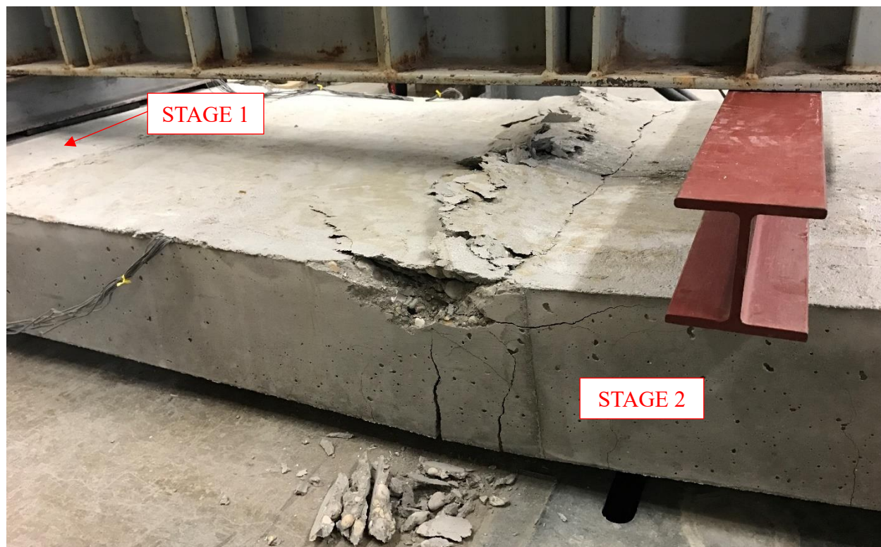
Figure 7.19 – Flexural-compression failure of Specimen 1 at the termination of the transverse reinforcement extending from Stage 1 into Stage 2.
