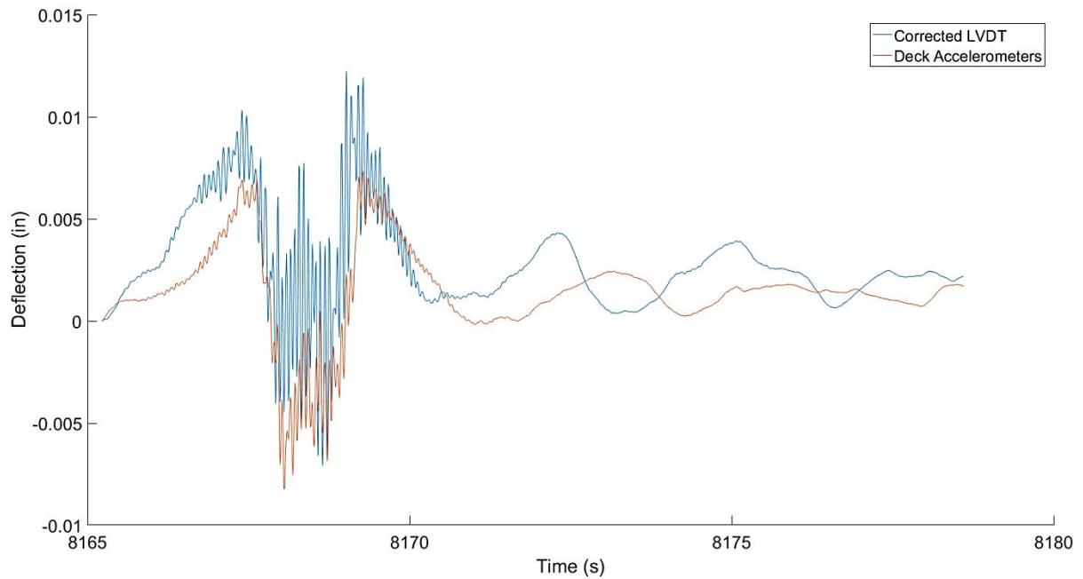
Figure 5.9- Typical trace of differential deflection versus time for bridge B-16-136
