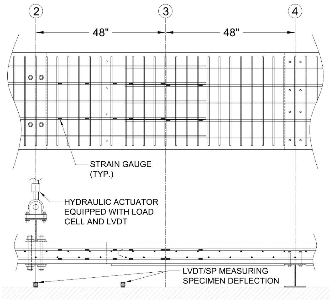
Figure 7.5 – Plan and profile view of instrumentation locations
