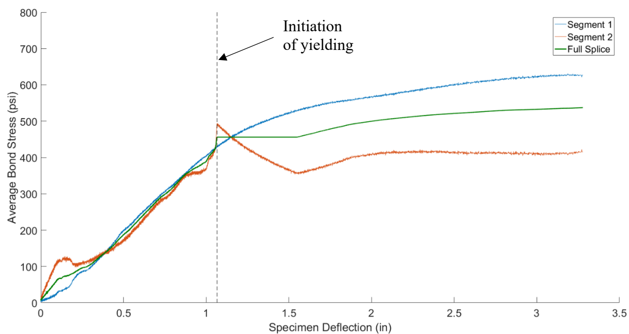
Figure 7.21 - Specimen 1 average bond stress versus specimen displacement for spliced Stage 1 bottom transverse reinforcement.
