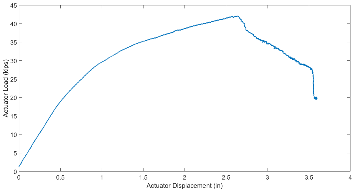
Figure 7.30 - Actuator load versus displacement response for ultimate test of Specimen 2.
