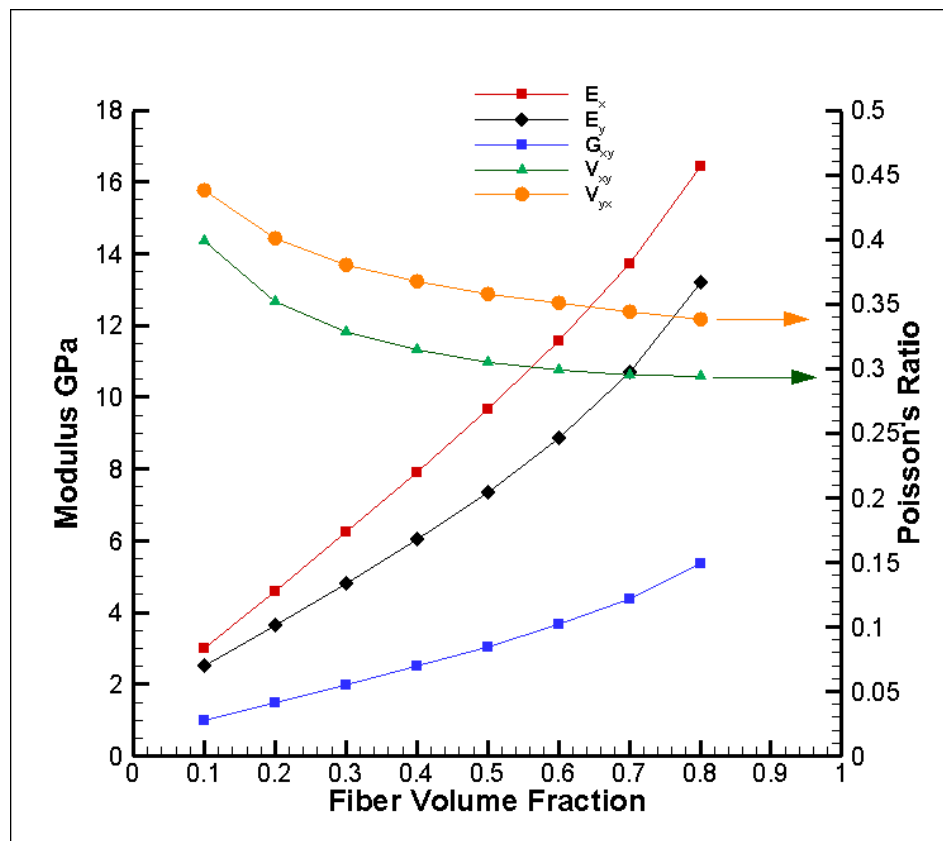
Figure 13 Analytical model results for the effect of changing the fiber volume fraction on the elastic moduli ( E_x , E_y , G_{xy} ) and Poisson's ratio ( \nu_{xy} , \nu_{yx} )
