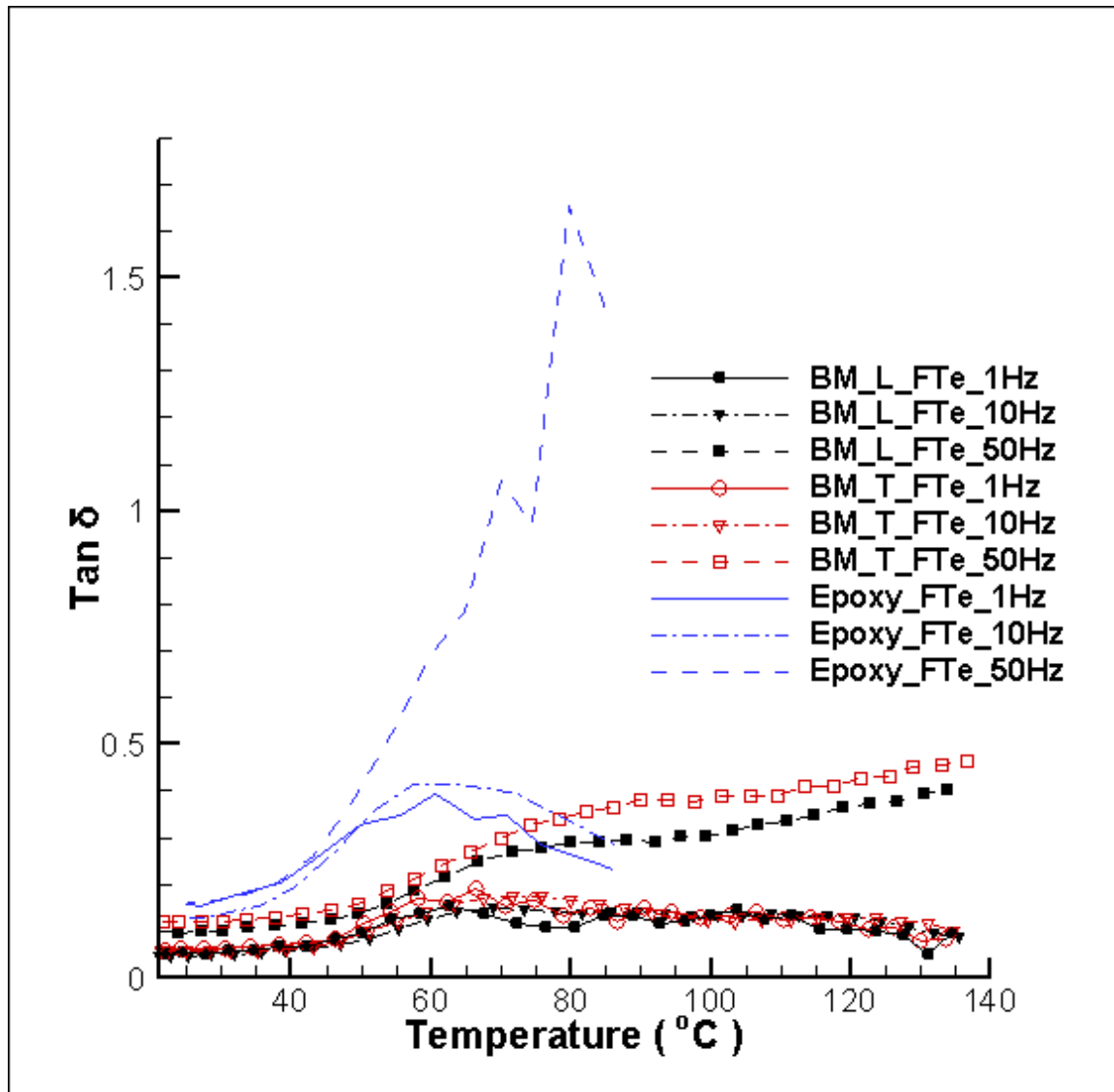
Figure 38 Changes in \tan \delta plots of neat epoxy and longitudinal and transverse dry triaxially braided cellulose composites with temperature ramping at different frequencies
