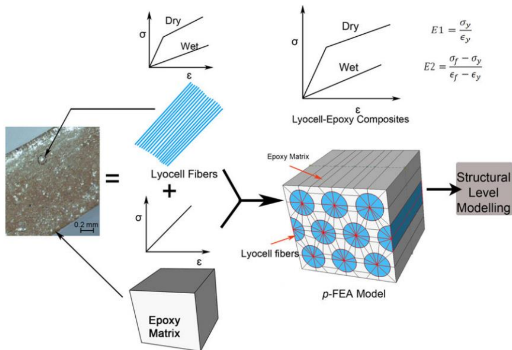
Figure 1 Schematic of analysis approach for Lyocell/epoxy composites with bilinear elastic-plastic fiber response ( Elhajjar and Qamhia, 2013 )
