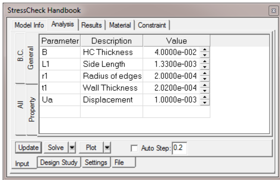
Figure 53 Parameterized parameters for the directionally oriented CNFs unit cell model
