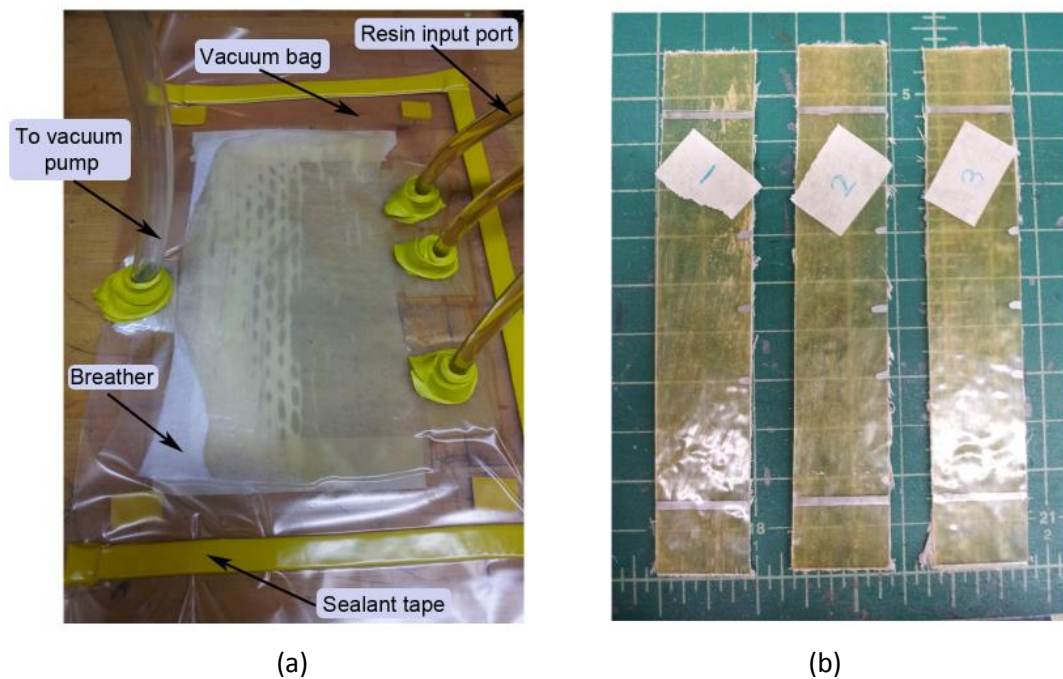
Figure 6 Fabrication techniques for Lyocell/epoxy composites showing (a) a resin infusion panel and (b) specimens prepared by manual layup
