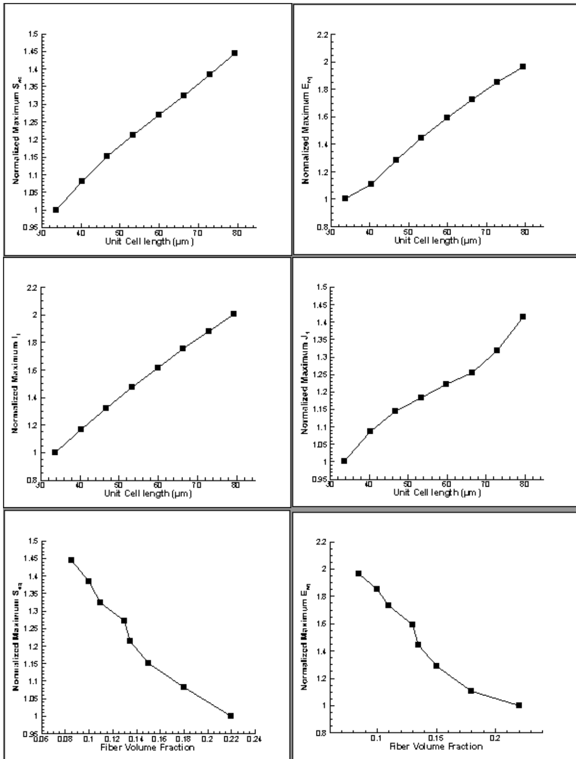
Figure 56 Model results for varying unit cell length and a constant wall thickness (5.1 \mu\text{m} )
