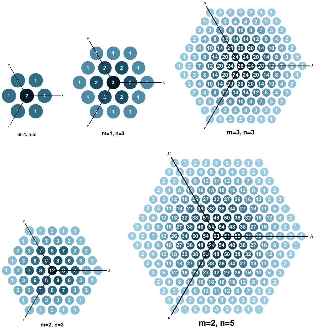
Figure 12: Plots of the distribution of D -values for d = 3 . By Theorem 6.14, these are also the weight diagrams of the space U = \otimes^3 S^m(\mathbb{C}^n) as a virtual \mathfrak{sl}_3 -representation.
