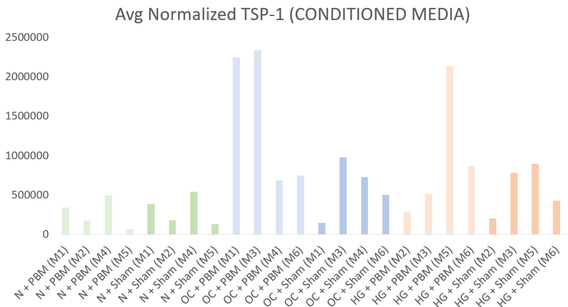
Supplementary Figure 5: Compiled relative quantities of TSP-1 in Muller cell conditioned media across blots. TSP-1 signal normalized to total protein. Y-axis represents chemiluminescent signal density. No inter-blot normalization. Each bar represents a duplicate average. M# = media blot number.
